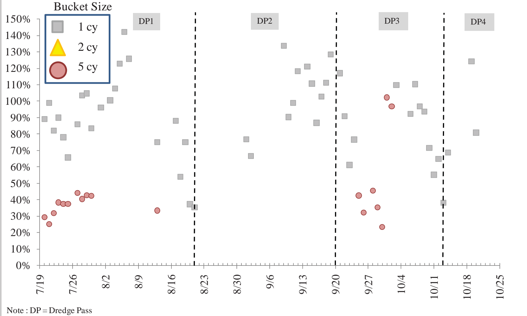
Average Daily Bucket Filling Efficiency
