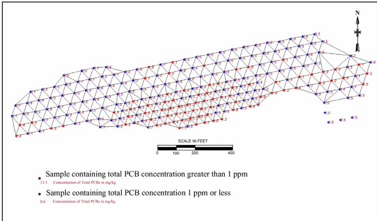
Figure 2-8 Reynolds Post-Dredging PCB Data Semi-Variogram Analysis 70' x 70' and 50' x 50' Triangular Grid Spacing
