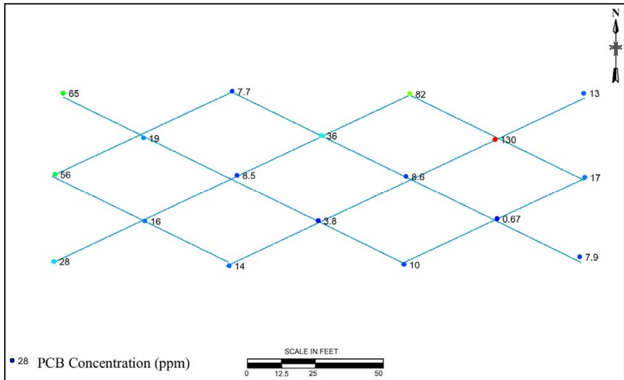
Figure 2-12 New Bedford Harbor Core Sample Semi-Variogram Analysis 40' Triangular Grid Spacing
