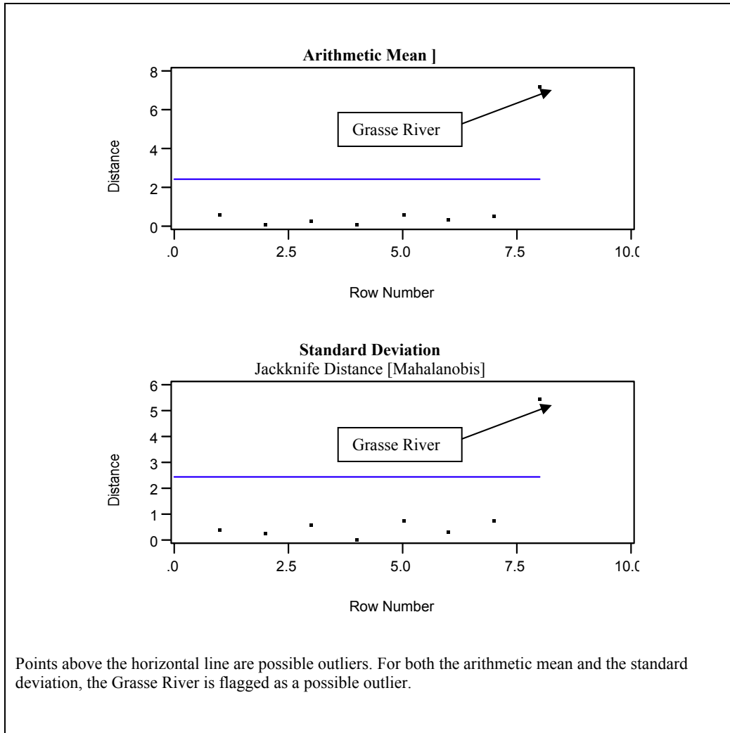
Figure 2-3 Mahalanobis Jackknife Distance for the Eight Case Studies
