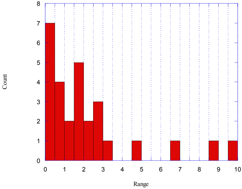
Figure 2-4 Histograms for Lognormal or Approximately Lognormal Data Sets Fox SMU PCB Concentrations (ppm)
