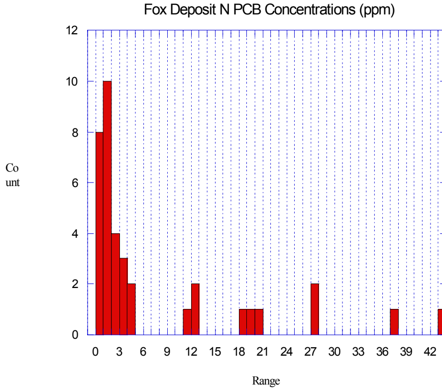
Figure 2-4 Histograms for Lognormal or Approximately Lognormal Data Sets
