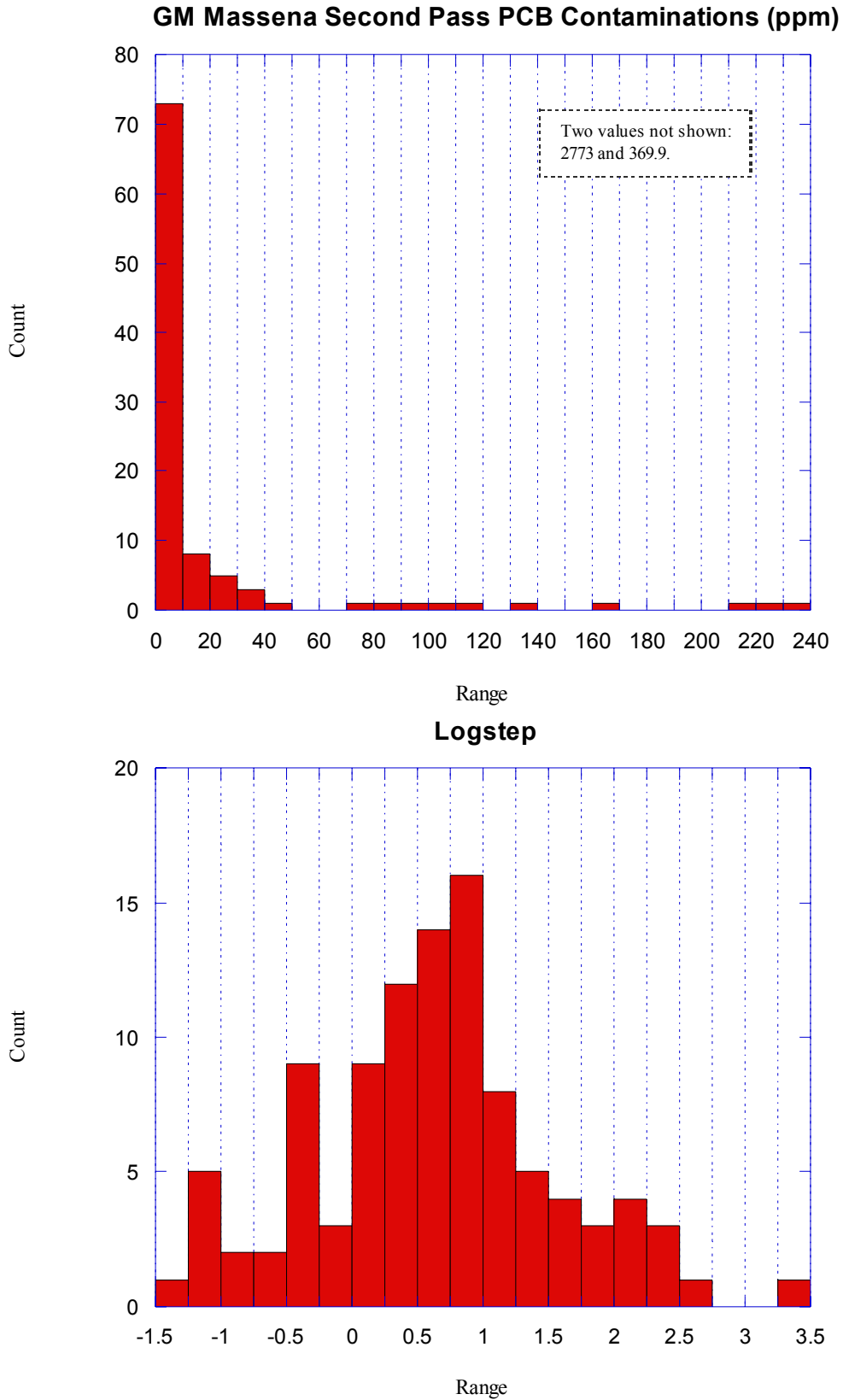
Figure 2-4 Histograms for Lognormal or Approximately Lognormal Data Sets
