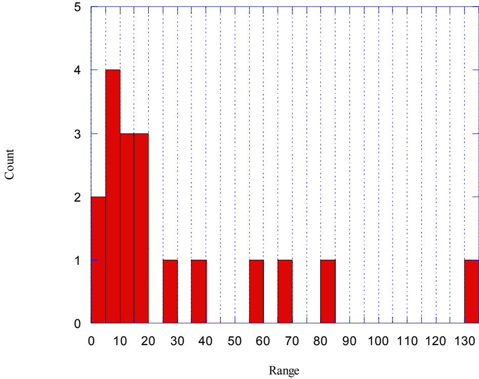
Figure 2-4 Histograms for Lognormal or Approximately Lognormal Data Sets New Bedford Harbor (Cores) PCB Concentrations (ppm)
