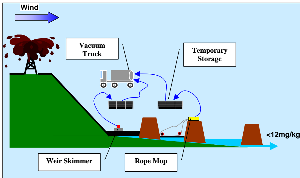
Figure 3. Diagrammatic representation of the oil / water separation pits.
