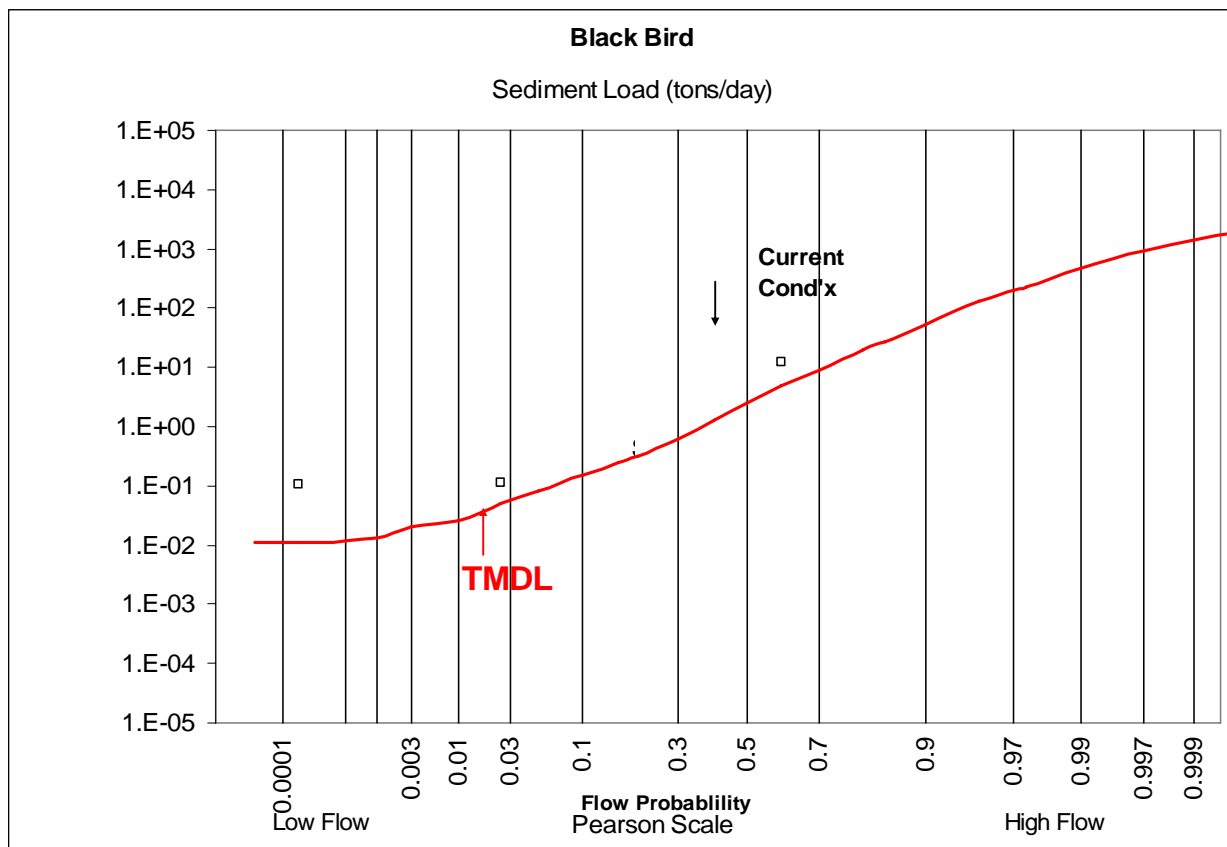
Figure 1 -- TMDL curve over the range of flows.
