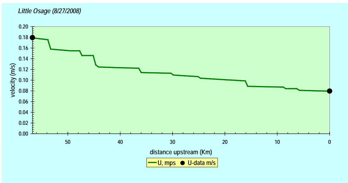
Figure 2. Measured and predicted flow, depths and velocities for Little Osage River
