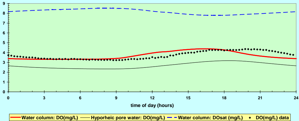
Figure 3. Comparison of measured and model predicted DO for Little Osage sites.
