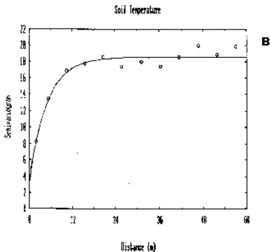
Figure 3.3.1. The semivariogram function for the surface moisture content (in A) and the surface soil temperature (in B) using the Variogram Calculation (Sample) program and the data set, C912.DAT.
