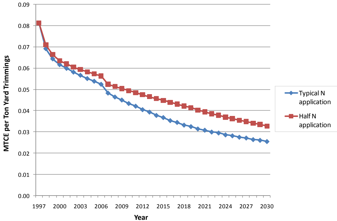
Exhibit 5: Incremental Carbon Storage as a Function of Nitrogen Application Rate at the Iowa Site
