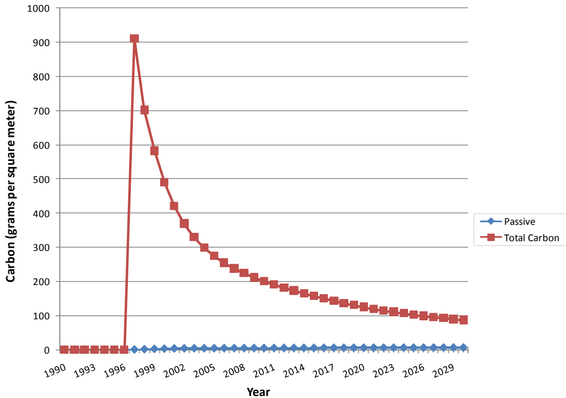
Exhibit 7: Difference in Carbon Storage Between Compost Addition and Base Case Yearly Application with 20 Tons Compost
