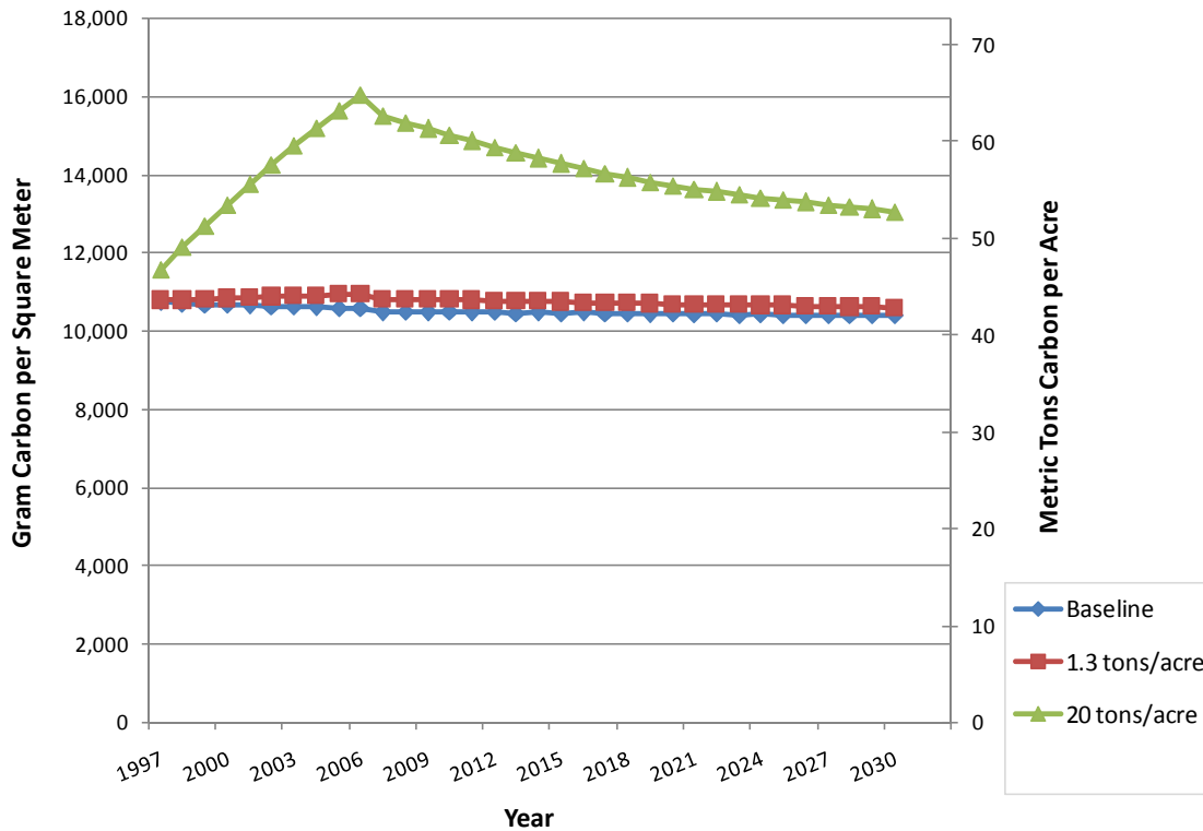
Exhibit 4: Total Soil C; Iowa Site, Corn Harvested for Grain
