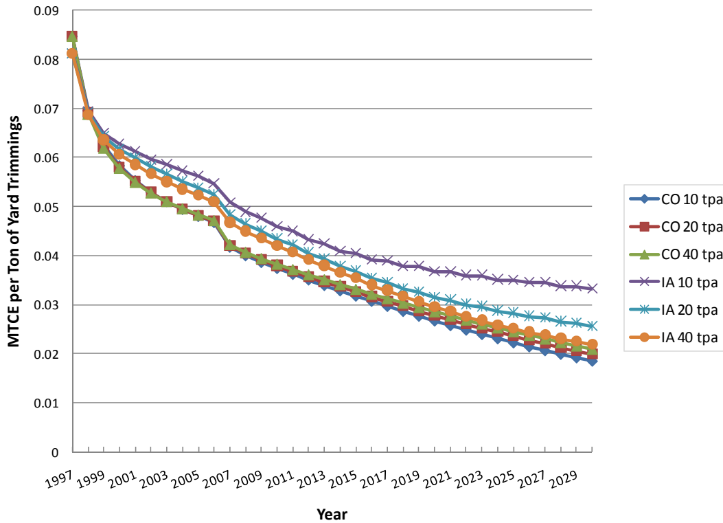
Exhibit 3: Soil Carbon Storage—Colorado and Iowa Sites; 10, 20, and 40 Tons-per-Acre Application Rates
