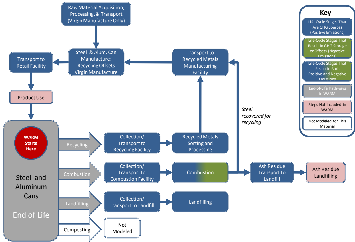
Exhibit 1: Life Cycle of Aluminum and Steel Cans in WARM
