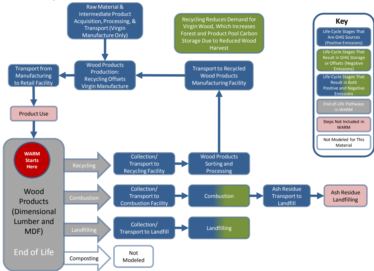
Exhibit 1: Life Cycle of Wood Products in WARM
