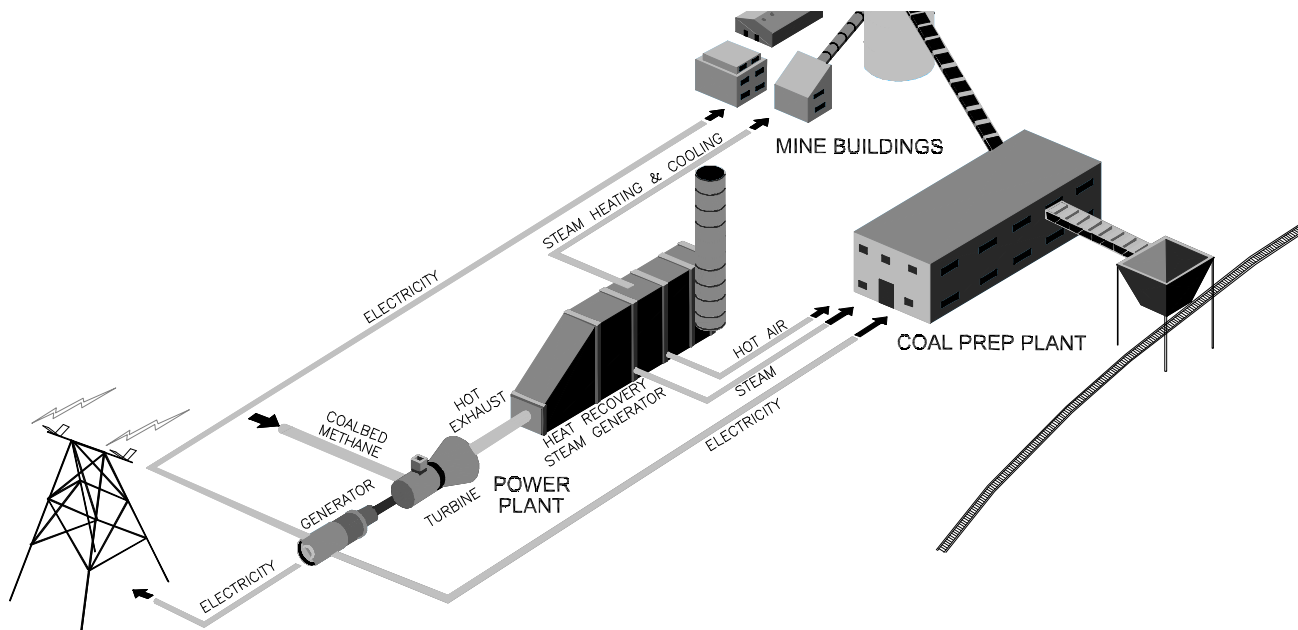
Schematic of a cogeneration facility located at a coal mine with a coal prep plant on site
