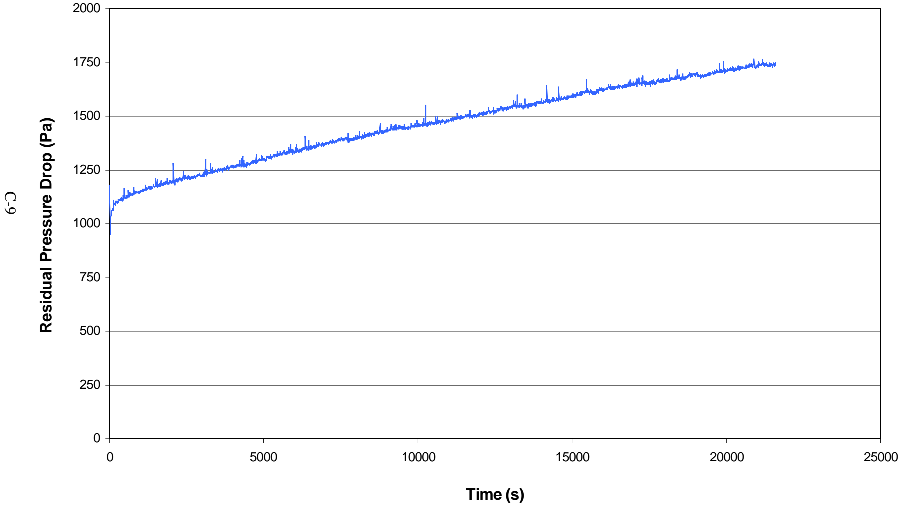
Figure C-2. Residual pressure drop across filter fabric during performance test run V012-1.
