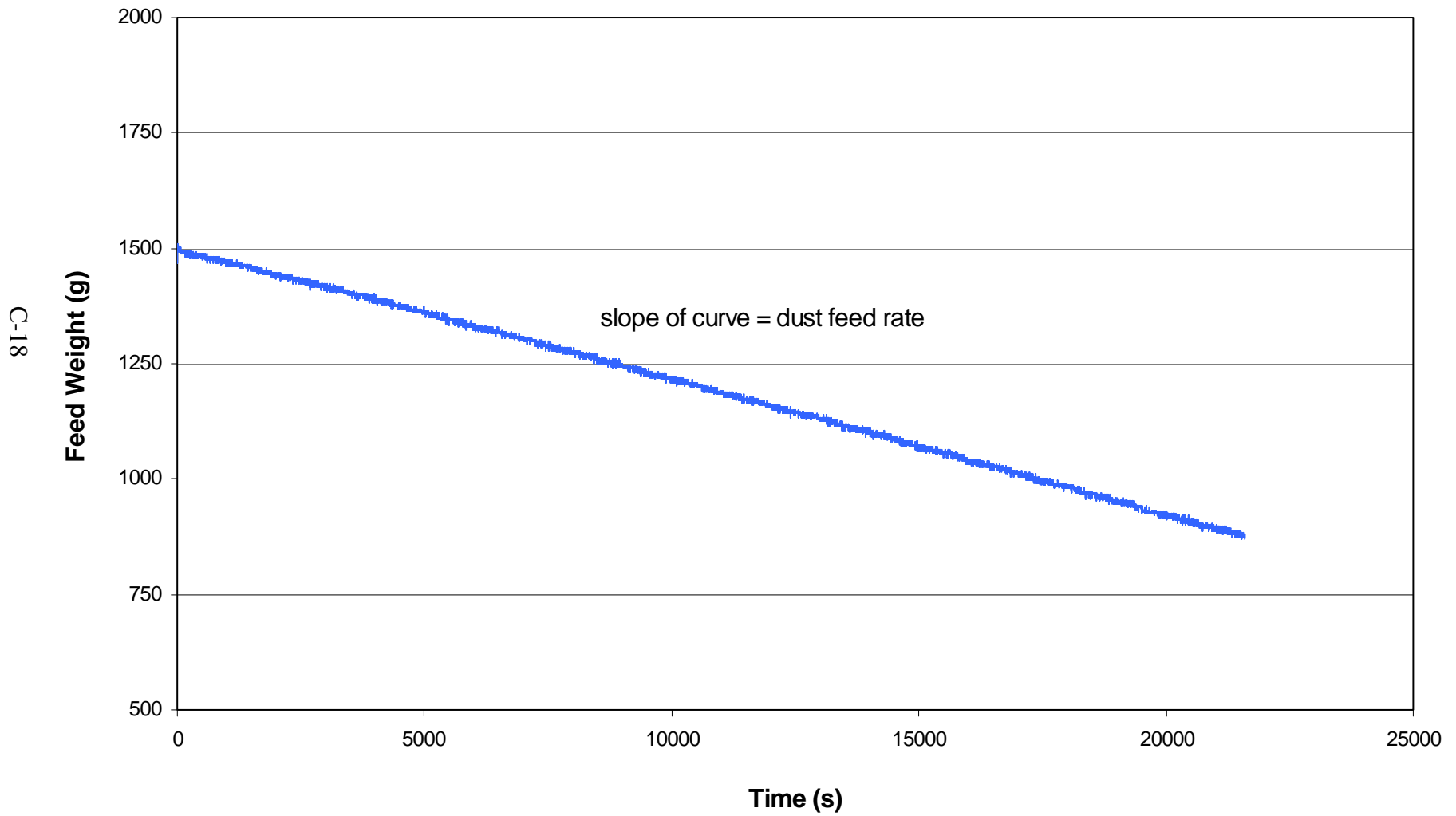
Figure C-5. Change in Pural NF dust scale reading with time during performance test run V012-3.
