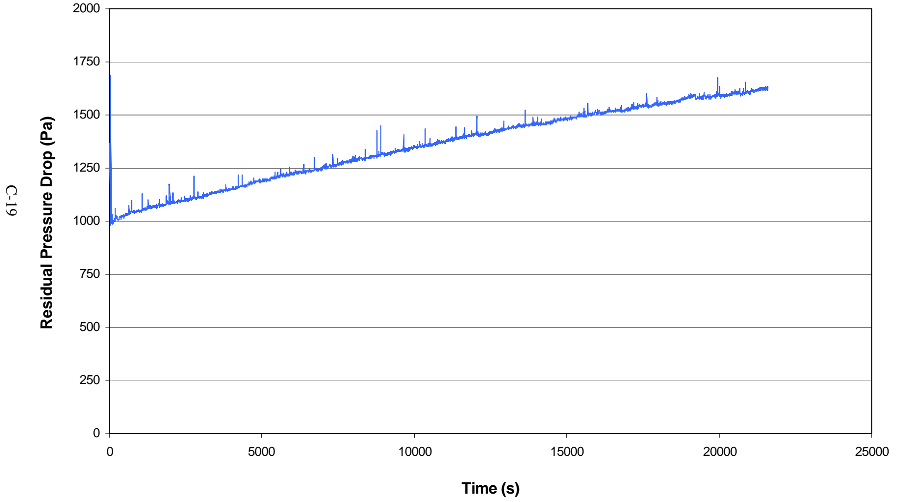
Figure C-6. Residual pressure drop across filter fabric during performance test run V012-3.
