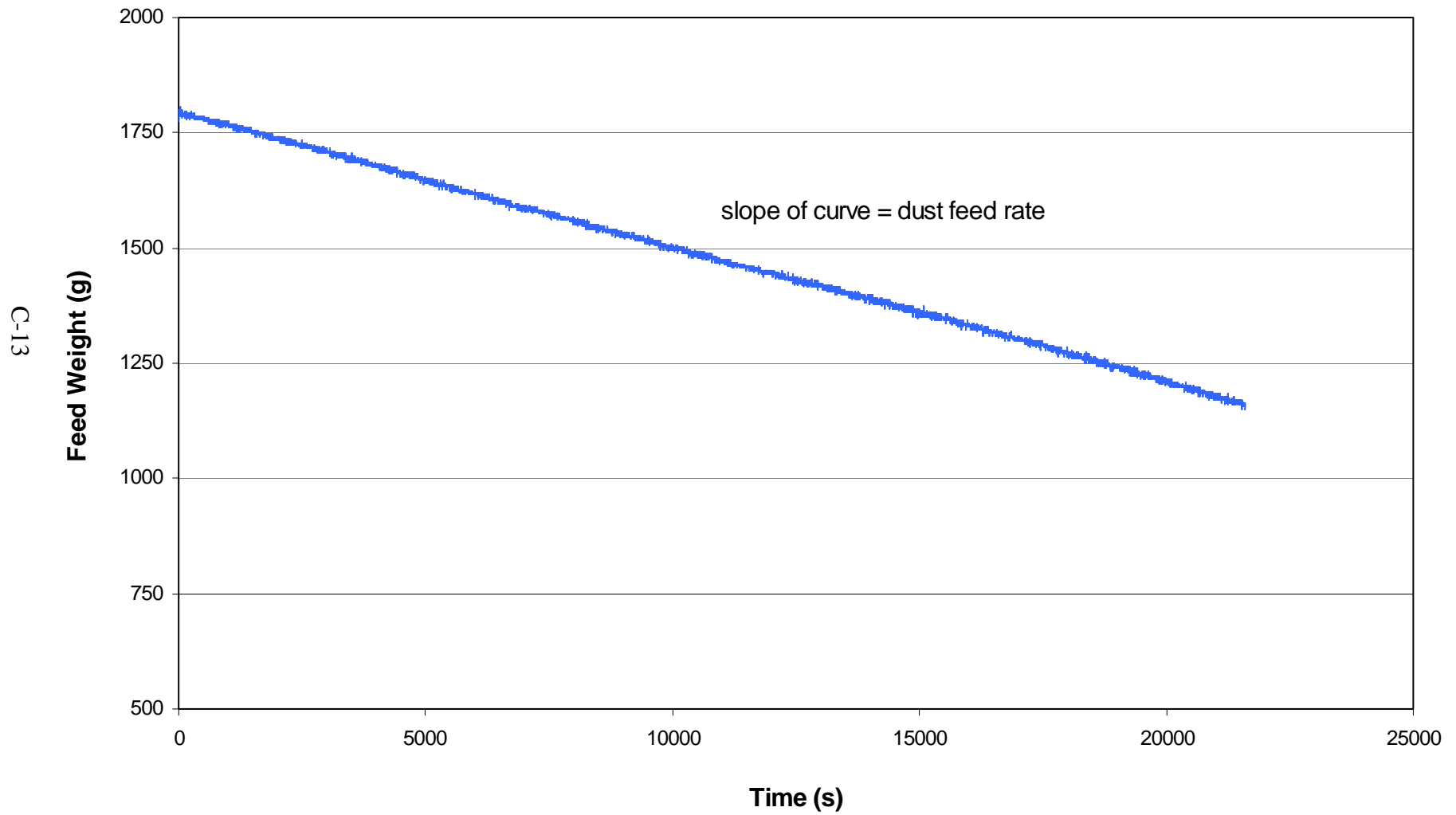
Figure C-3. Change in Pural NF dust scale reading with time during performance test run V012-2.
