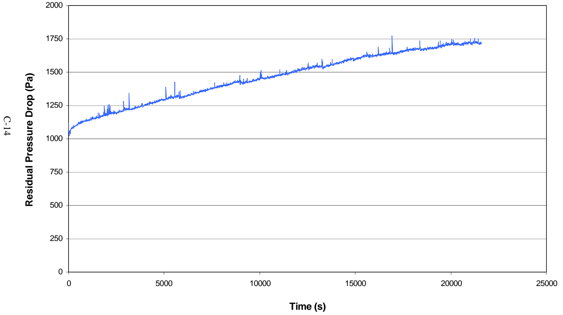
Figure C-4. Residual pressure drop across filter fabric during performance test run V012-2.
