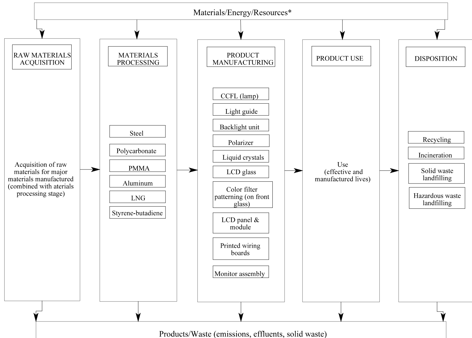
Figure 1-7. LCD Life-Cycle
