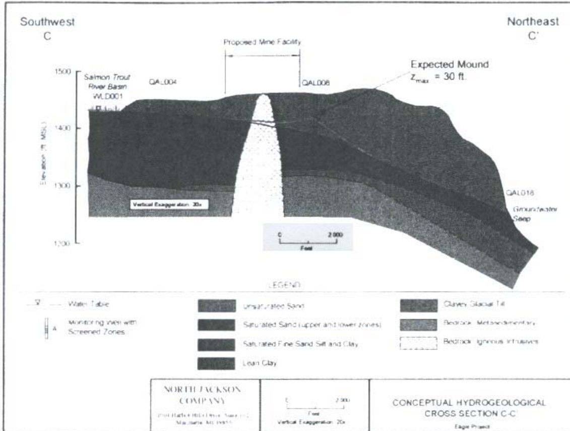
Figure 2. Conceptual Hydrogeological Cross Section C-C'. From Foth and Van Dyke, 2006
