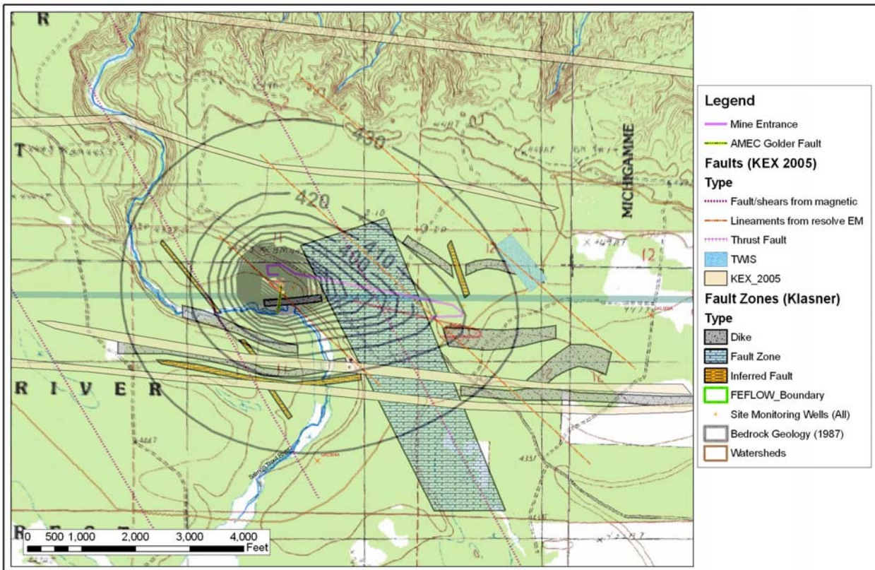
Figure 6. Site geology, and hydraulic heads predicted for when mining has ceased, using revised base case (Golder Associates, 2006b, Figure 9.2). The mapped area is within the FEFLOW model area.
