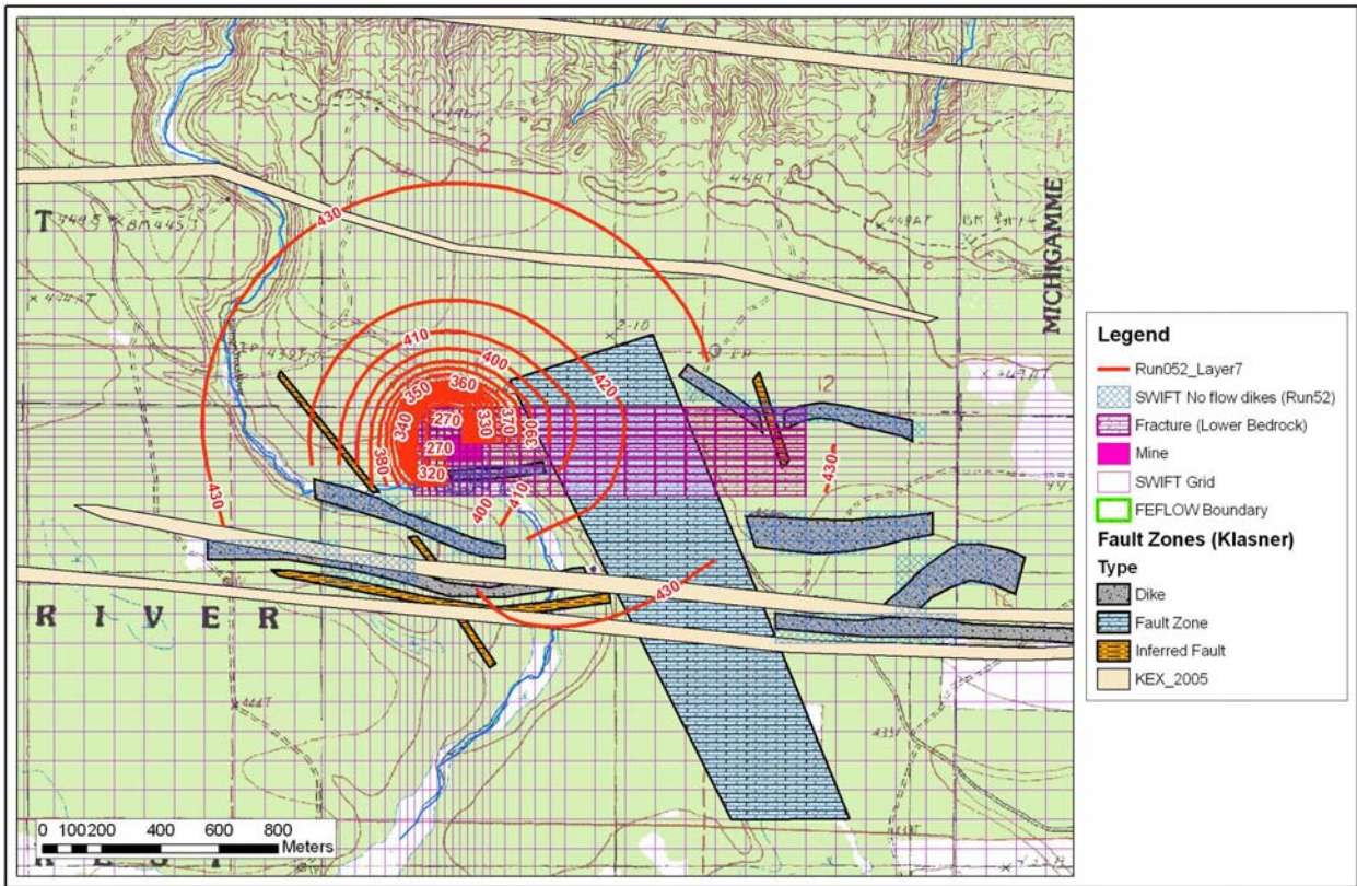
Figure 12. Predicted results including hypothesized no-flow dikes. The mapped area is within the FEFLOW model area.
