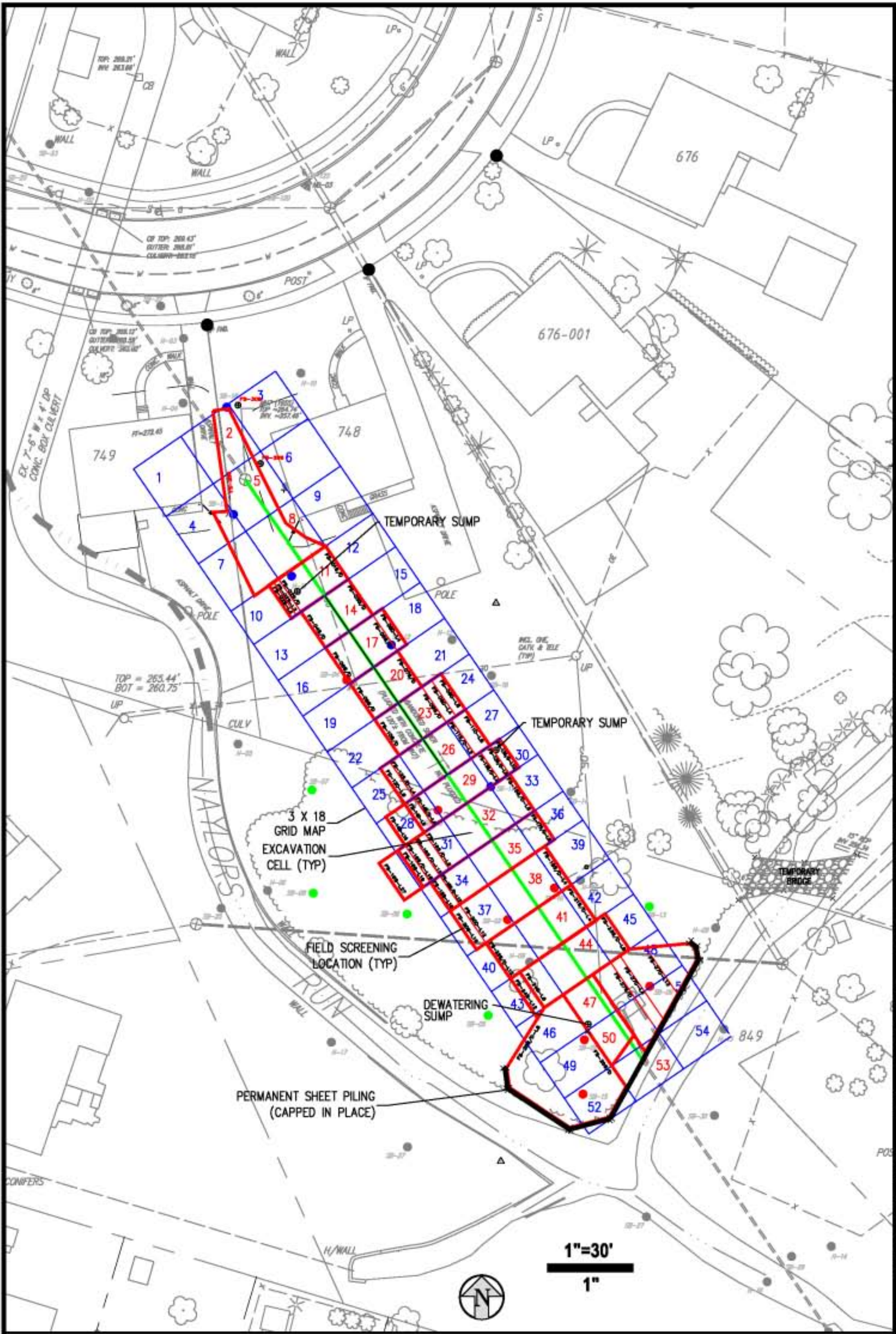
OU3 RA CLOSEOUT REPORT HAVERTOWN PCP SUPERFUND SITE ROS AREA EXCAVATION CELLS LAYOUT
