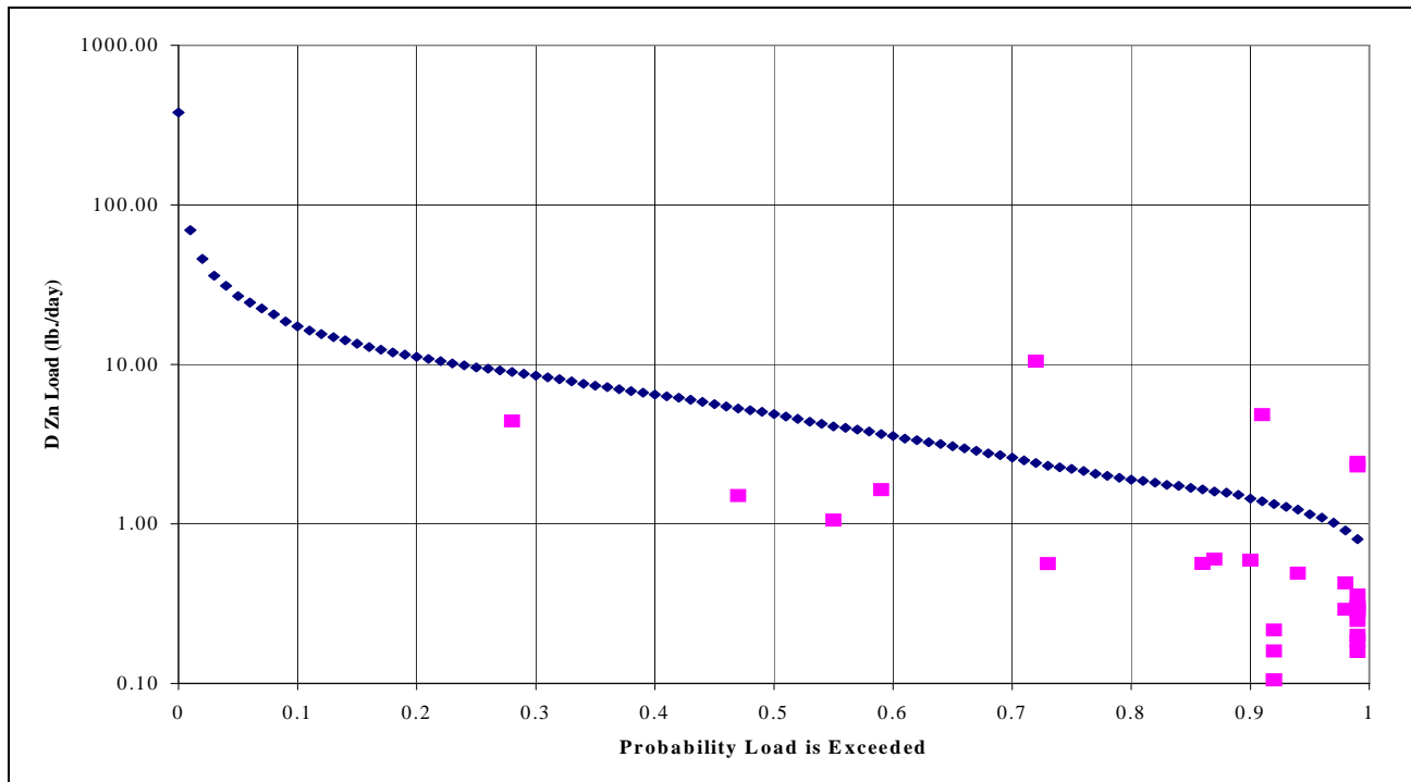
Figure 1: Load Duration Curve of Dissolved Zinc (TMDL) and Observed Loads.
