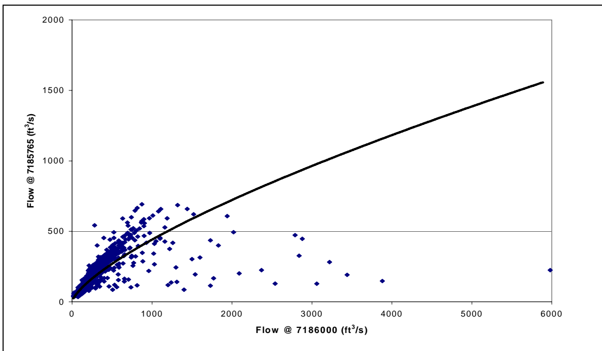
Figure 3. Flow relationship between USGS 07185765 at Carthage and USGS 07186000 near Waco, MO – both gauges are on Spring River.
