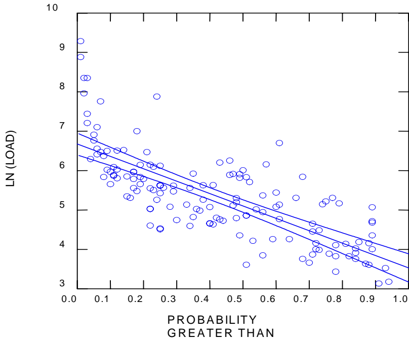
Figure A-2: Confidence Interval Band (95percent) around the regression line of ln (load)* probability flow for observed loads within base flow range (0 – 250 ft 3 /s)
