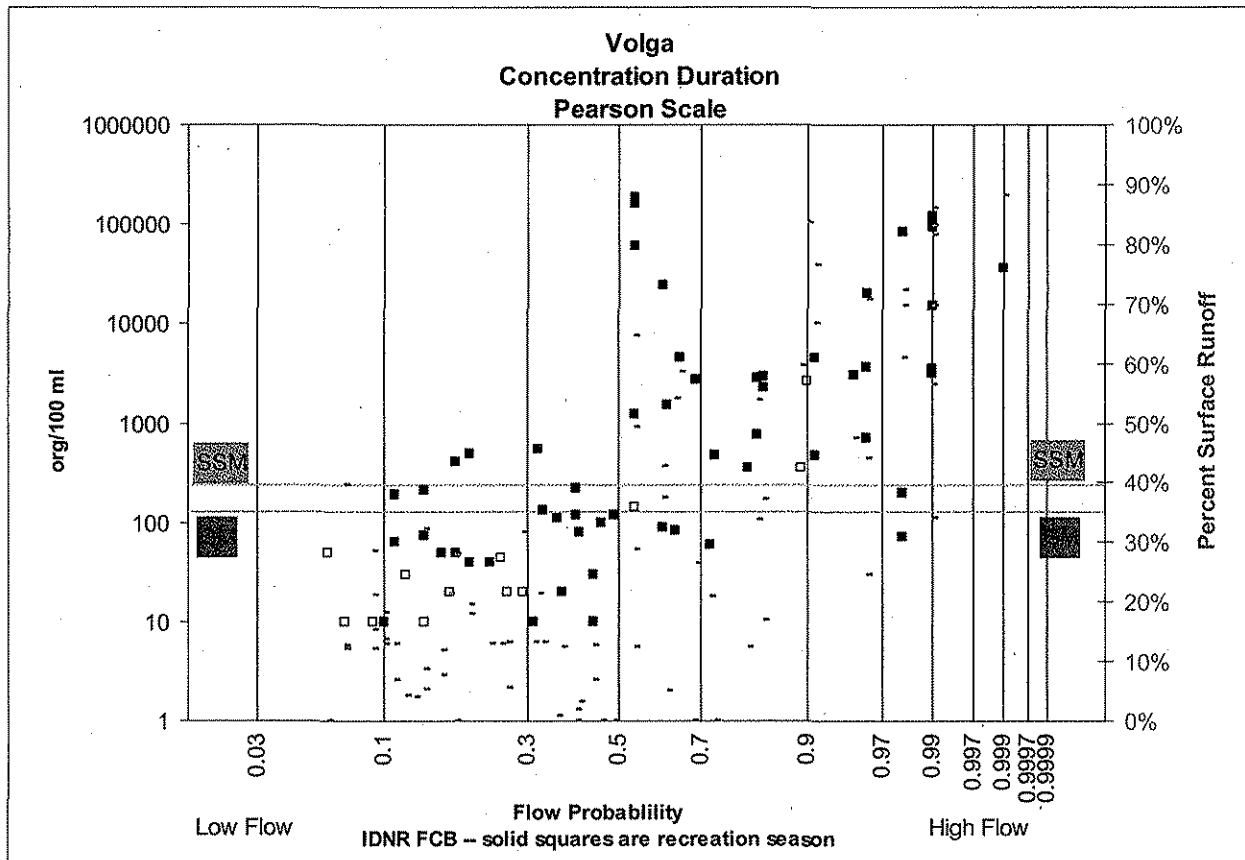
Figure 5 Sample results shown for various flow conditions and the estimated percent coming from surface runoff estimated using the base-flow separation procedure
