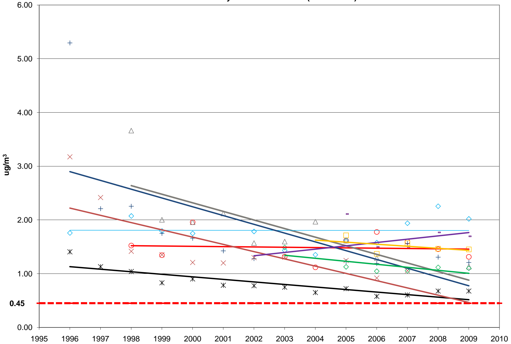
Annual Acetaldehyde Concentrations (1996 - 2009)
