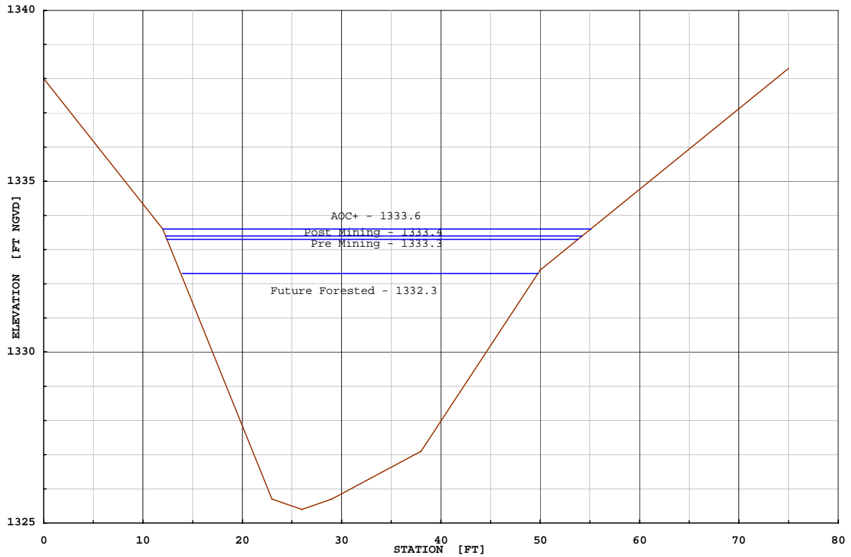
COMPARISON OF STAGES FOR 100 YEAR FLOWS
