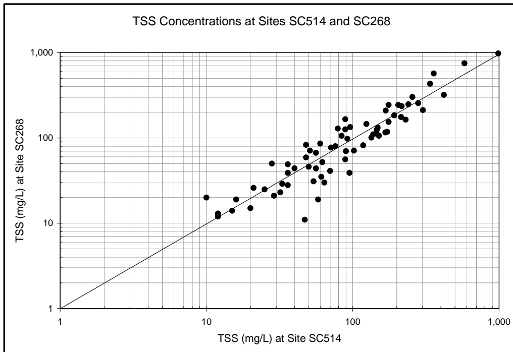
Figure 5a. A scatter plot of TSS concentrations for Sites SC514 and SC268 during 1997 – 2008.
