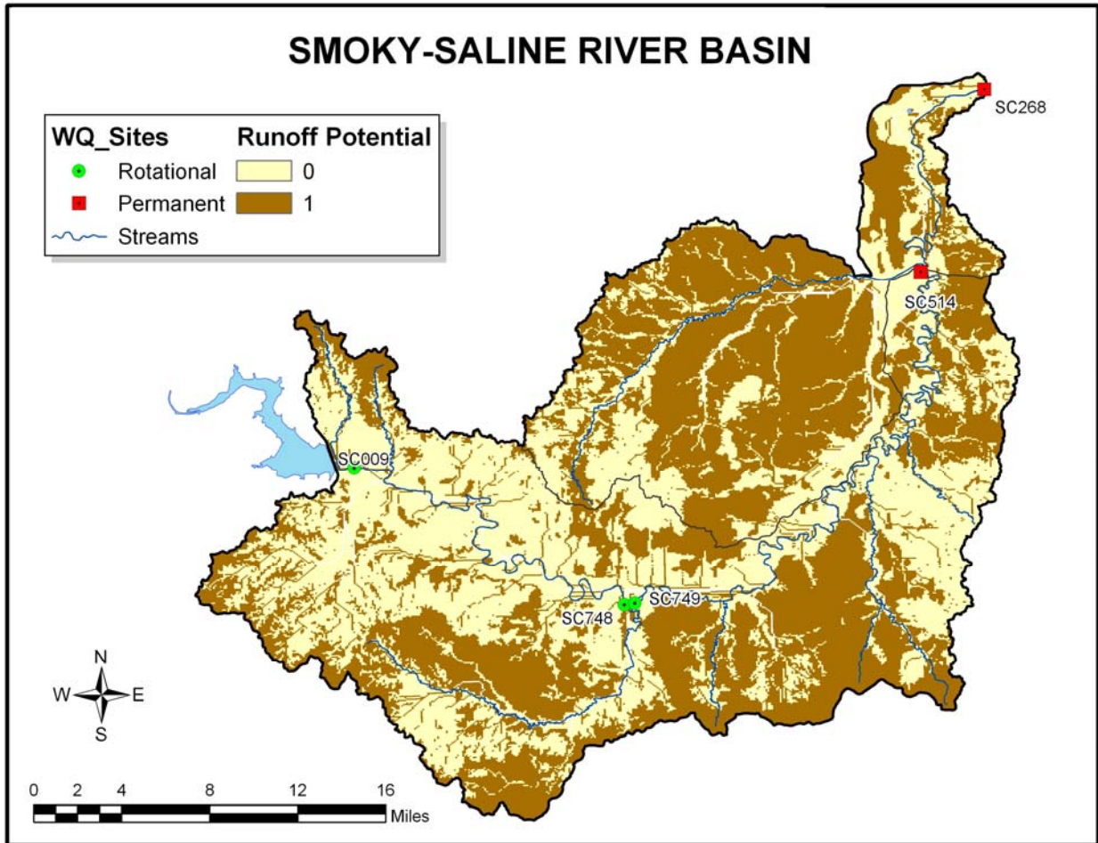
Figure 13. Estimated Runoff potential based on the very low (1.14"/hr) runoff condition (a value of 1 depicts potential contributing area, and 0 is for potential noncontributing area).
