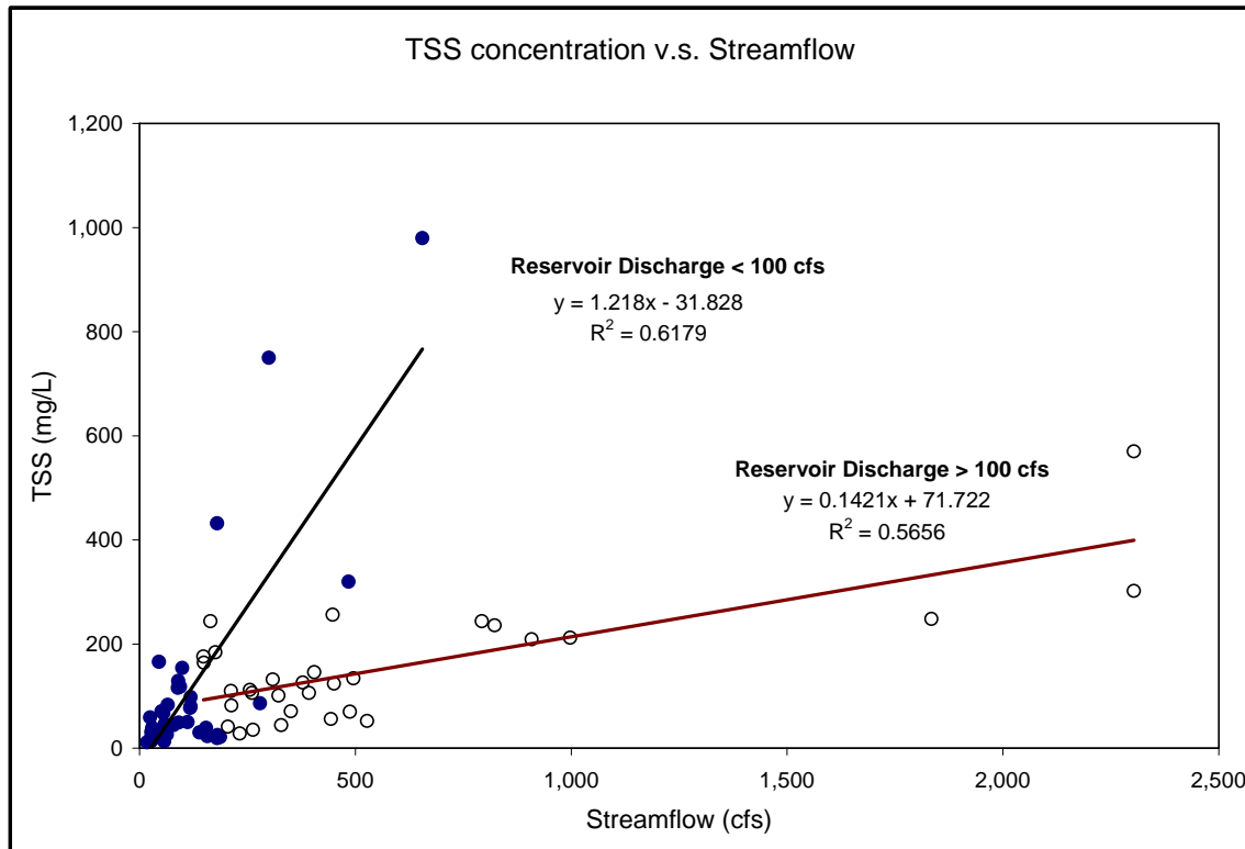
Figure 8. The TSS-streamflow relationship at Site SC268 during 1997 – 2008.
