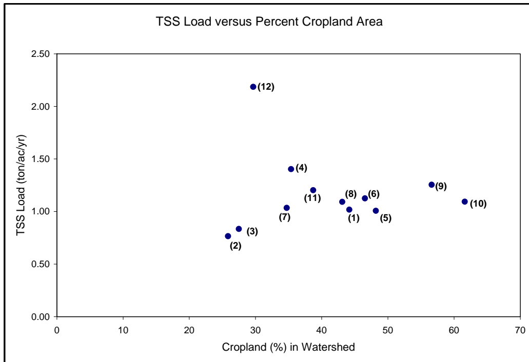
Figure 17. A scatter plot of TSS loads and percent cropland areas. The values in parenthesis are watershed identification (ID) numbers.
