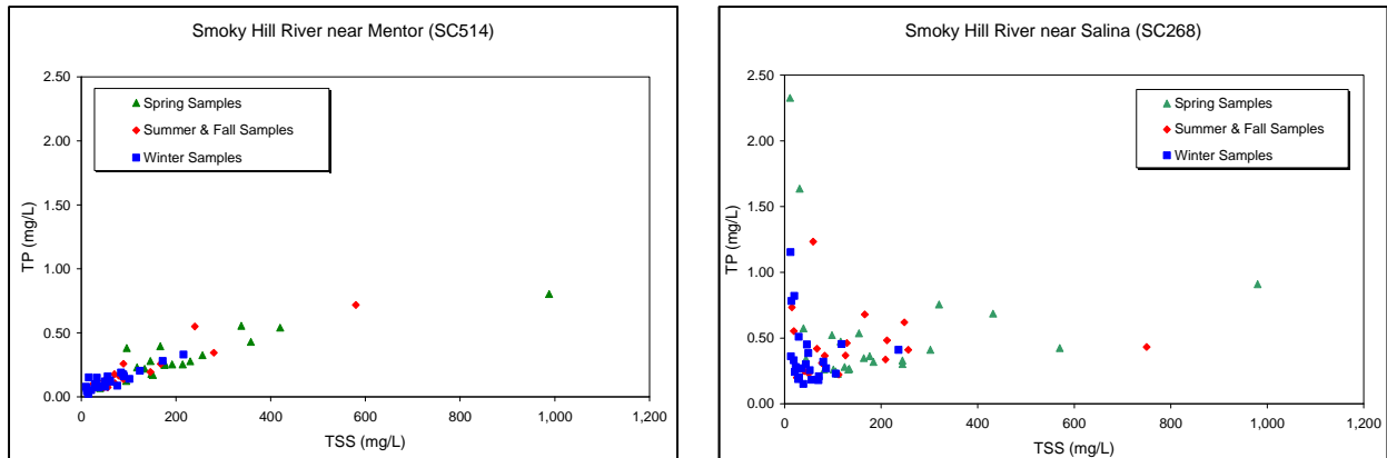
Figure 6. Seasonal scatter plots of TSS and TP concentrations for Sites SC514 and SC268.
