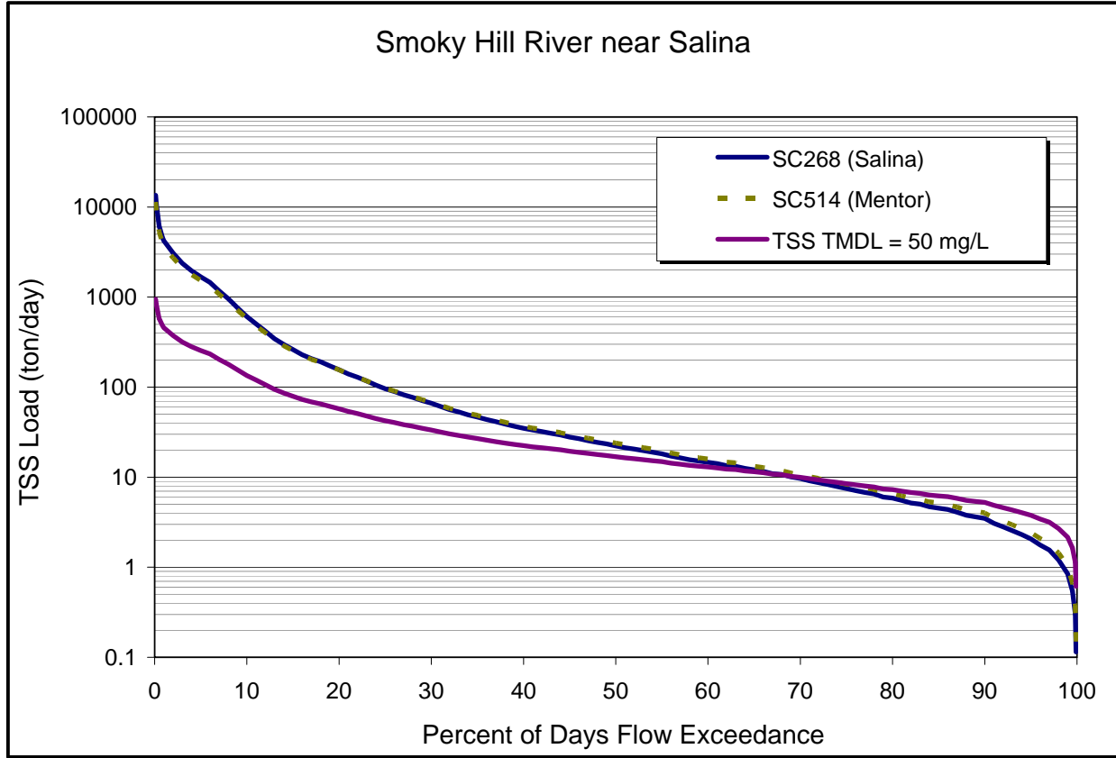
Figure 16. The daily TSS loads and TMDL's Load Allocation (LA) for the Smoky Hill River at Sites SC514 and SC268.
