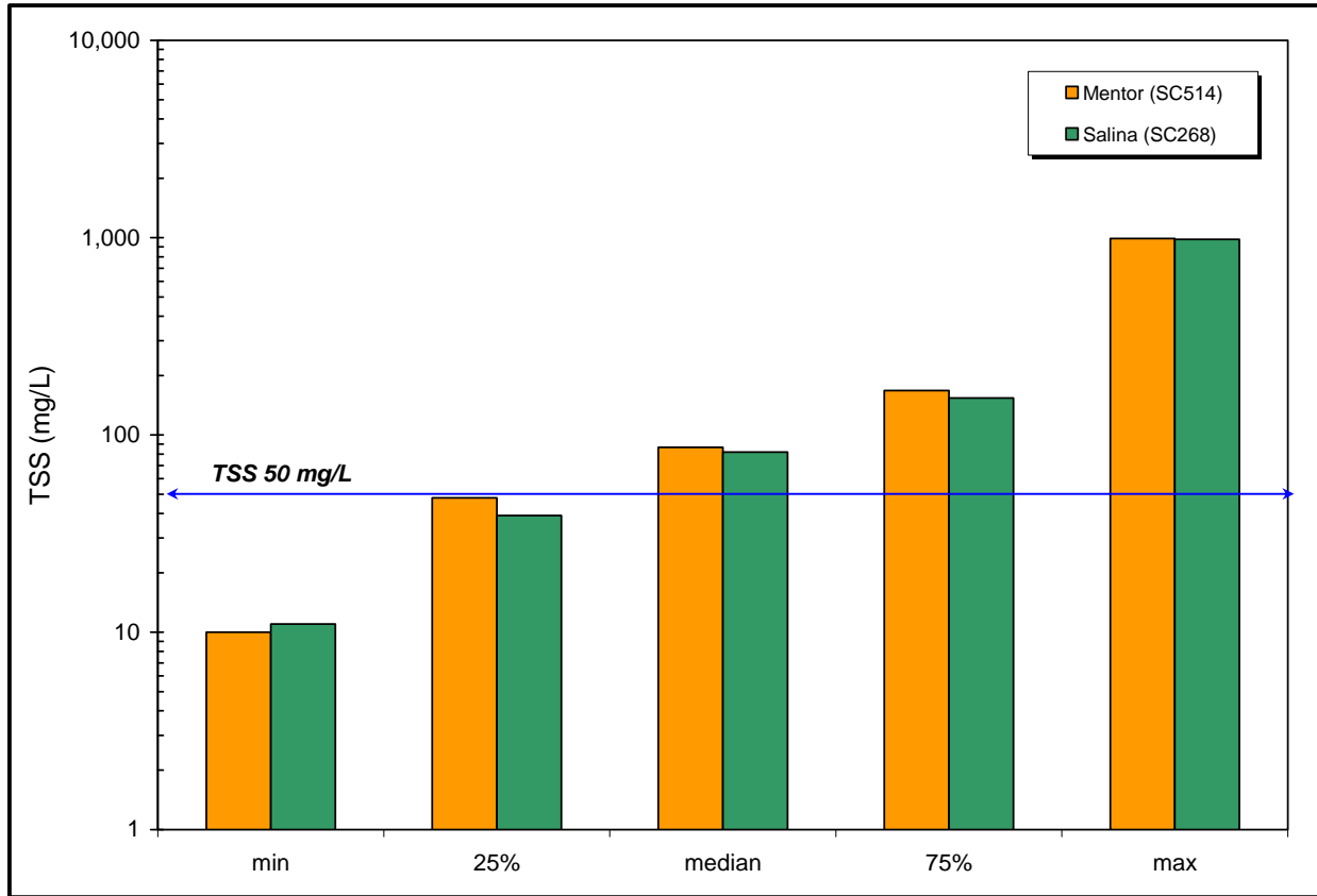
Figure 4. TSS percentile values during 1997 – 2008.
