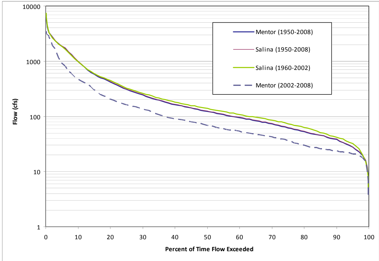
Figure 2. Flow duration curve plots for Smoky Hill River near Salina and Mentor (streamflow values were derived from USGS Gaging Station 06866500).
