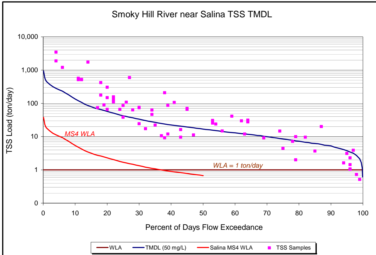
Figure 14. Smoky Hill River TSS TMDL near Salina.
