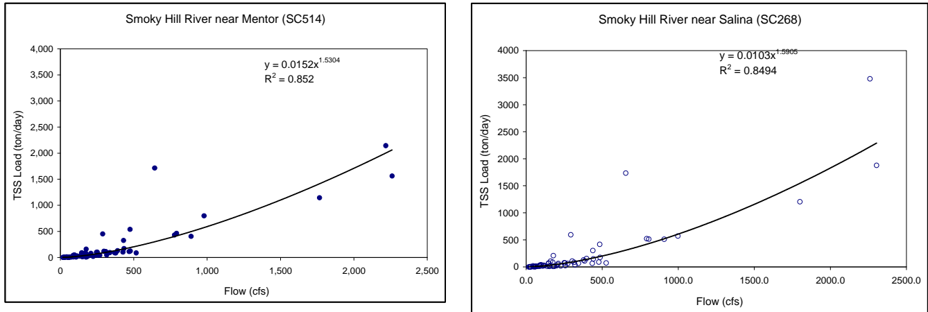
Figure 15. The relationships between flows and associated TSS loads for the Smoky Hill River at Sites SC514 and SC268.
