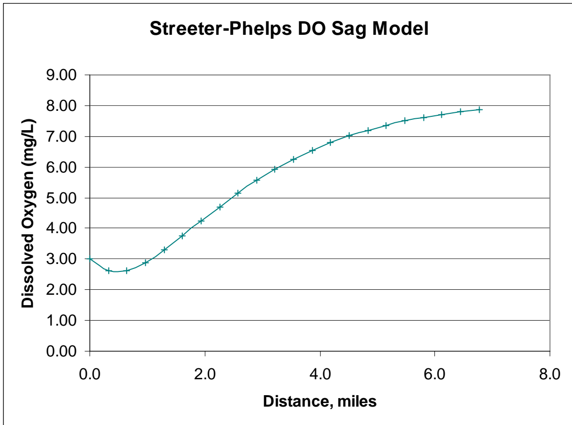
Figure 2. Sanborn WWTP Streeter Phelps Model Oxygen Sag Curve.
