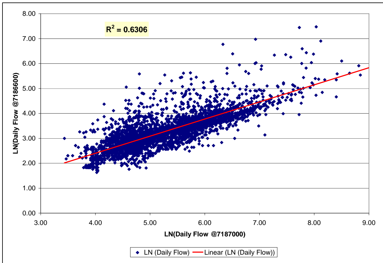
Figure 4: Daily Flow Relation at two Stations from October 1, 1963 to November 3, 1972 \text{LN}(Y) = 0.68 * \text{LN}(X) - (0.34)
