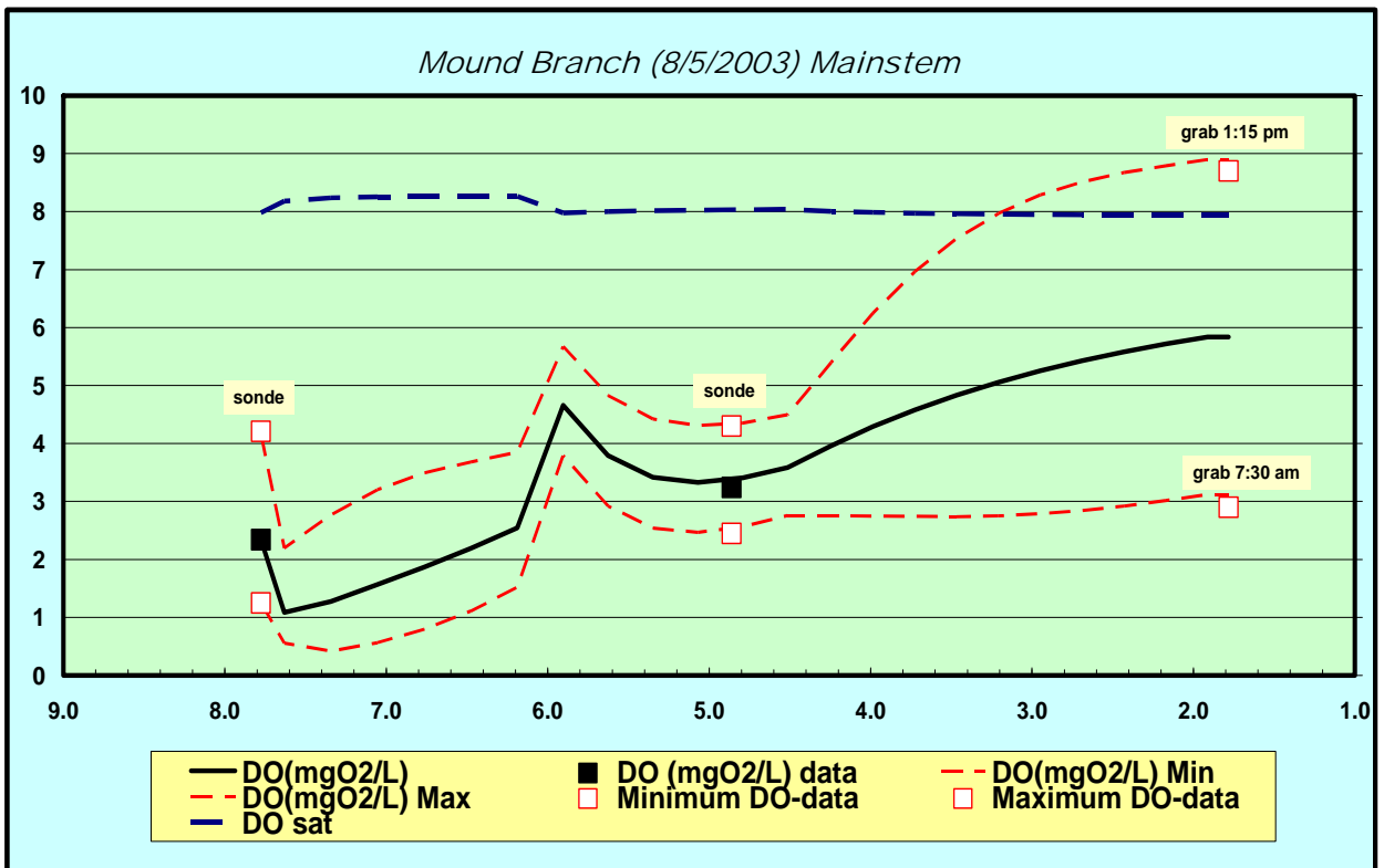
Figure B5. Predicted longitudinal profile of minimum, maximum and mean DO.
