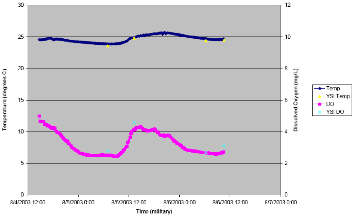
Figure Y. Temperature and dissolved oxygen data, Mound Branch Survey, Site B3/5 (downstream of Butler WWTP), Aug 4-6, 2003
