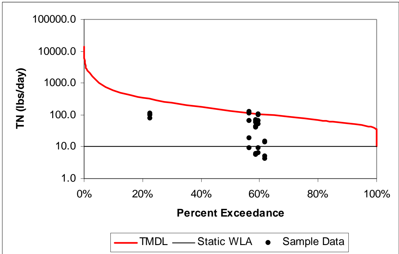
Figure 6. Load Duration Curve for Total Nitrogen – Mound Branch
