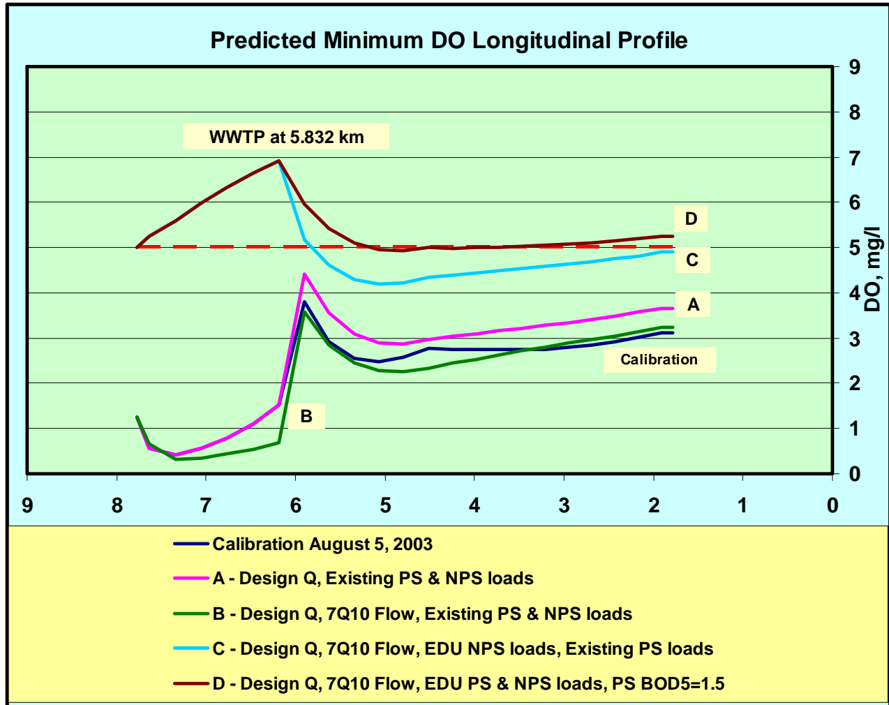
Figure B6. Predicted longitudinal profile of minimum dissolved oxygen for various simulation scenarios.
