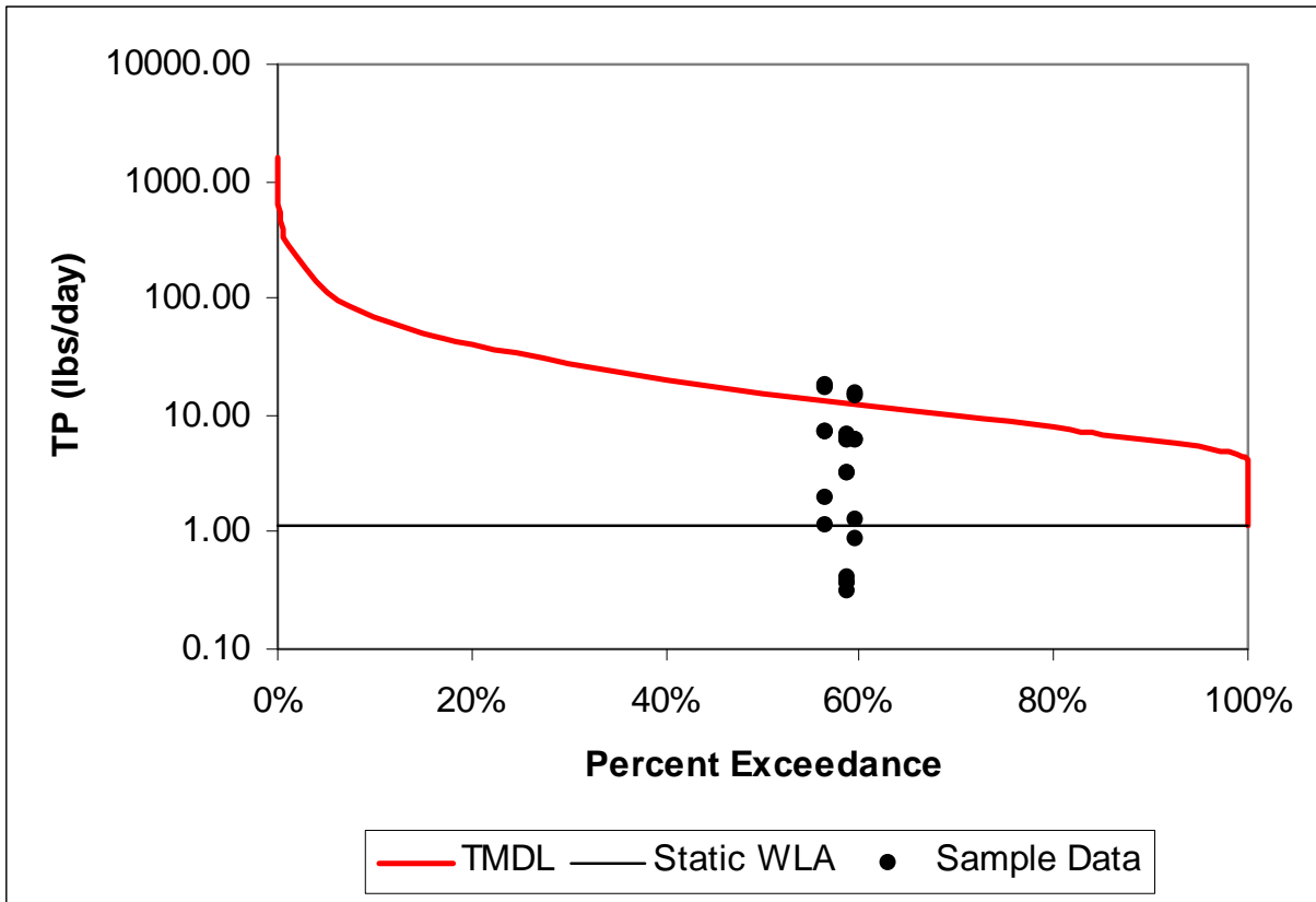
Figure 7. Load Duration Curve for Phosphorus – Mound Branch
