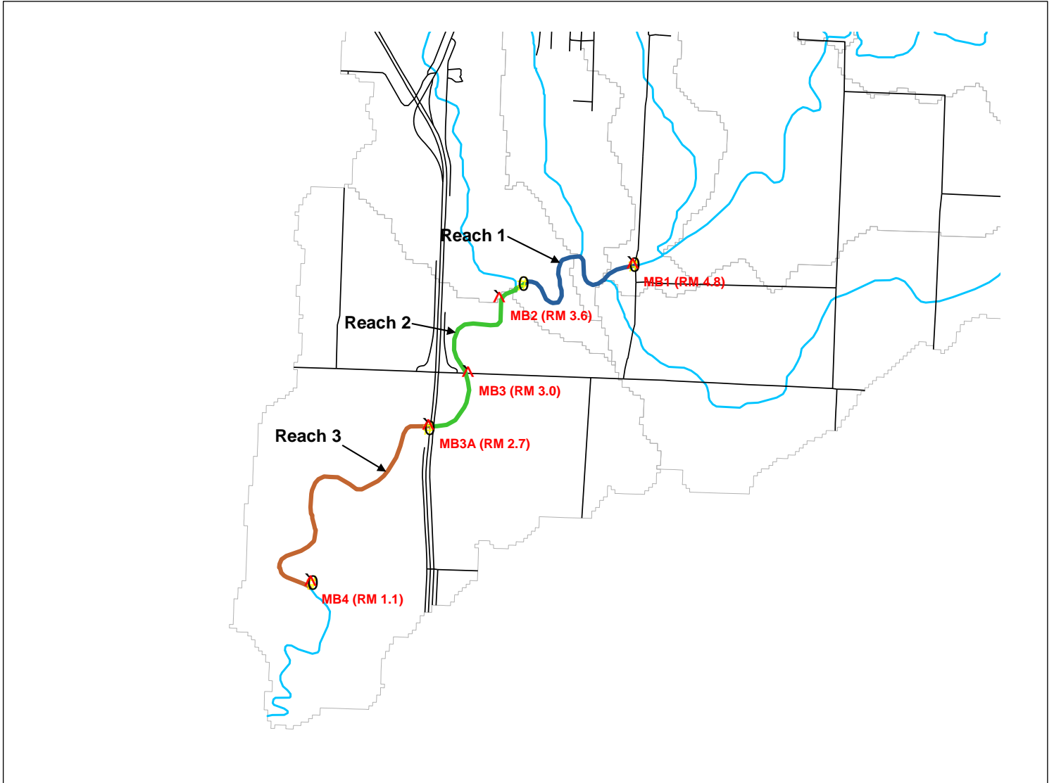
Figure B1. Map of Schematic QUAL2K Model Domain
