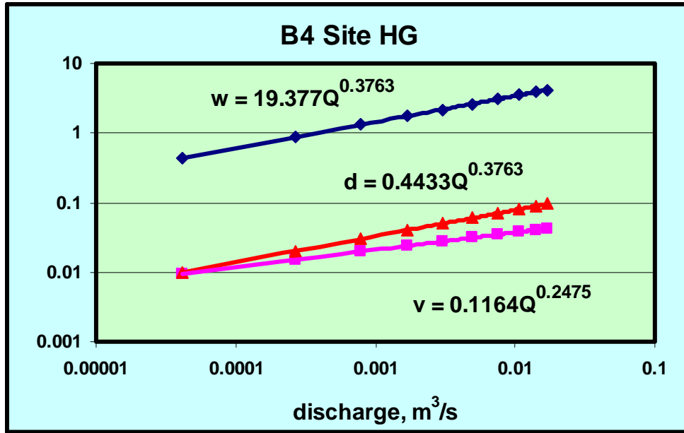
Figure B2. Hydraulic geometry functions for Mound Branch, August 5, 2003.
