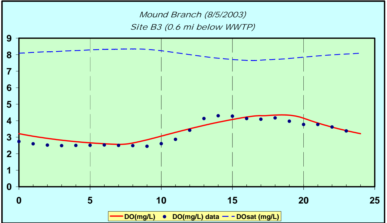
Figure B4. Observed and predicted diurnal dissolved oxygen at site B3.
