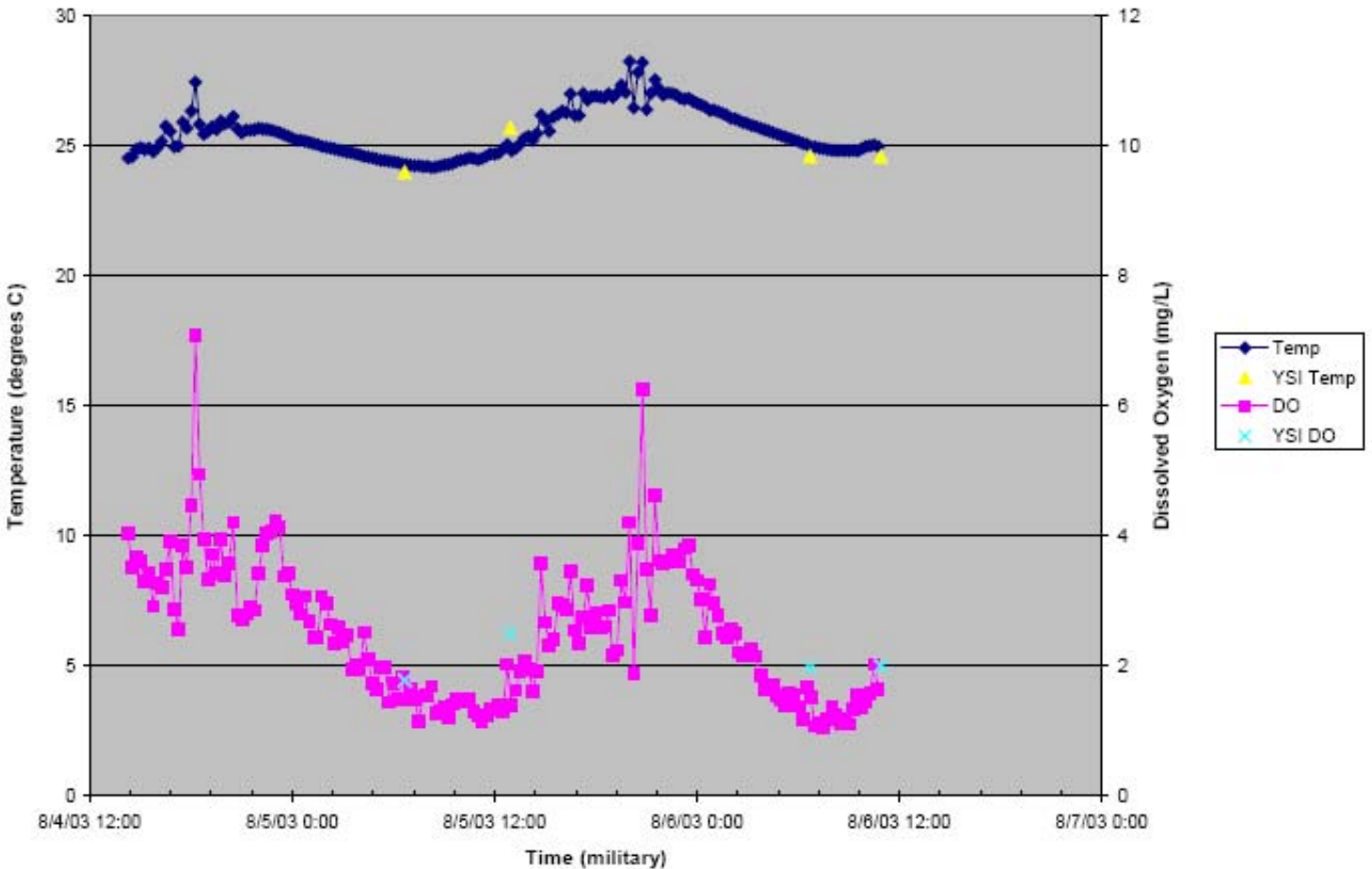
Figure X. Temperature and dissolved oxygen data, Mound Branch Survey, Site B1/3 (upstream of Butler WWTP), Aug 4-6, 2003
