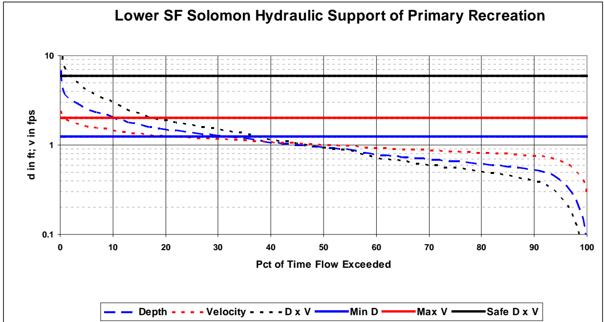
Figure 16. Hydraulic Geometry Supporting Primary Recreation on South Fork Solomon River
