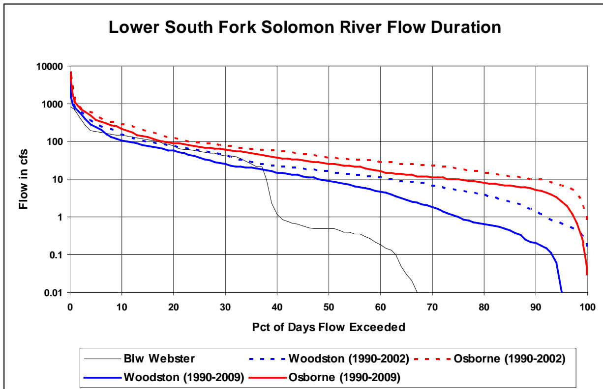
Figure 2. Flow Duration for Lower South Fork Solomon River
