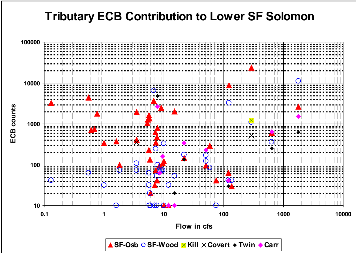
Figure 10. Tributary Contribution of E coli Bacteria to Lower South Fork Solomon River
