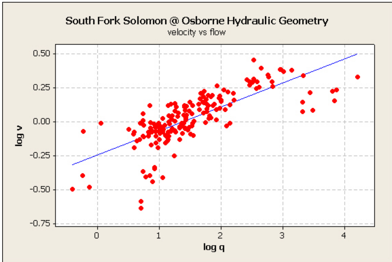
Figure 15. Log-normal relationship of velocity & flow on South Fork Solomon at Osborne
