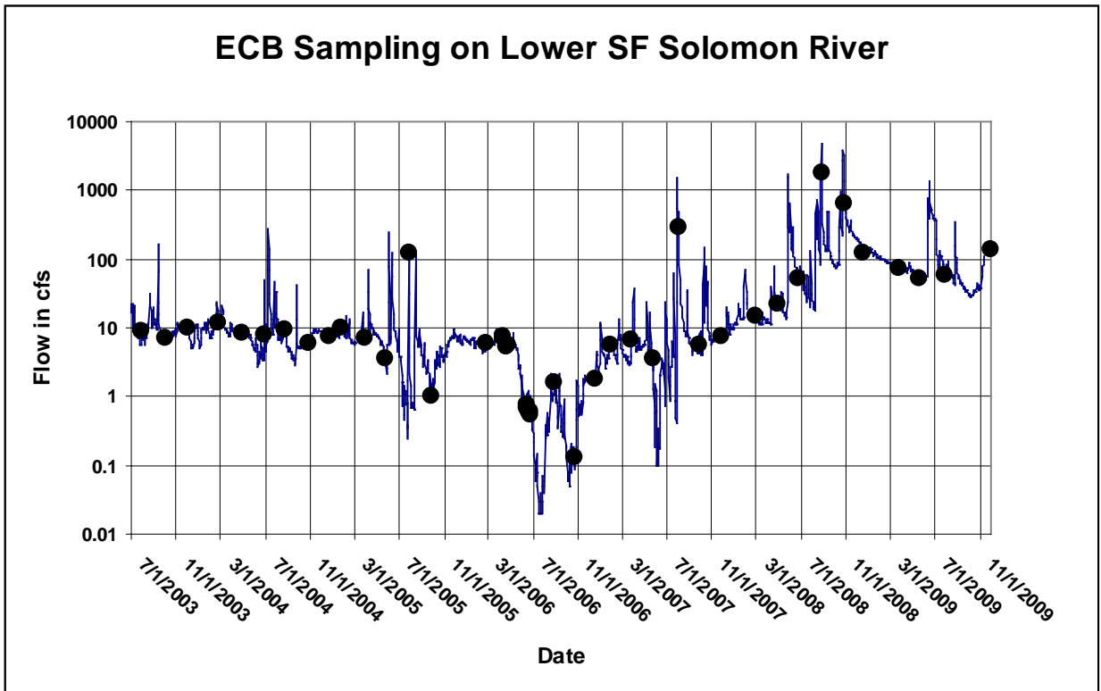
Figure 4. Daily Flows of South Fork Solomon River during 2003-2009 E coli Sampling
