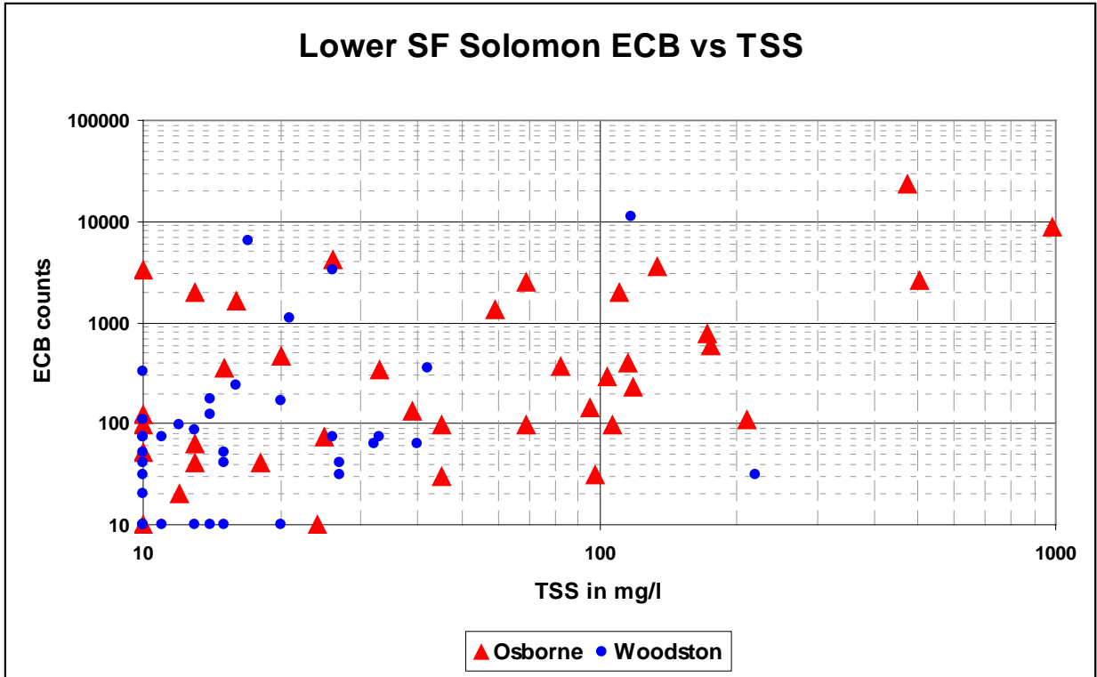
Figure 11. Bacteria – Suspended Solids Relationship in Lower South Fork Solomon River
