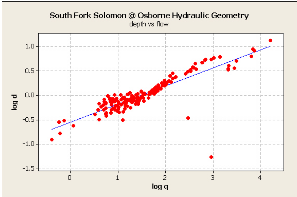
Figure 14. Log-normal relationship of depth & flow on South Fork Solomon at Osborne
