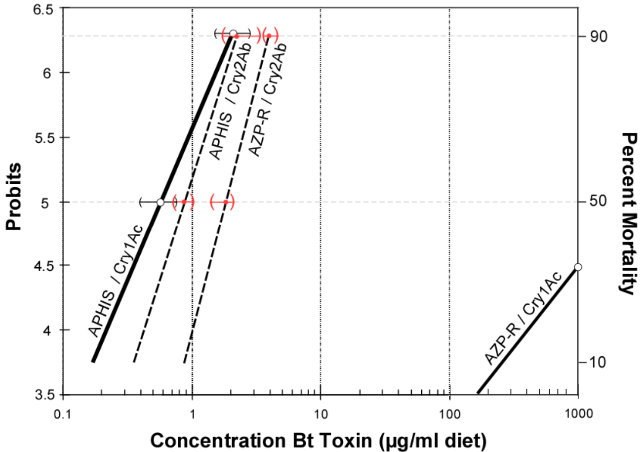
Figure 1. Susceptibility to Cry1Ac and Cry2Ab of two laboratory strains of pink bollworm from Arizona. The APHIS strain was maintained in the laboratory for over 3 decades without exposure to insecticides. The AZP-R strain was collected in the field in 1997 and repeatedly exposed to Cry1Ac in the laboratory. Probit lines with LC_{50} and LC_{90} estimates ( \pm 95% F.L.) are provided for all culture/toxin combinations except AZP-R/Cry1Ac. Response of AZP-R to Cry1Ac departed significantly from the probit model and thus is provided as mean corrected mortality observed at the concentrations tested. Mean corrected mortality of AZP-R was 2.16% (SEM 1.44) in bioassays of 100 \mu g Cry1Ac/ml diet and 29.8% (SEM 5.96) in bioassays of 1000 \mu g Cr1Ac/ml diet. Concentration response data for all evaluations are provided in Table 1.
