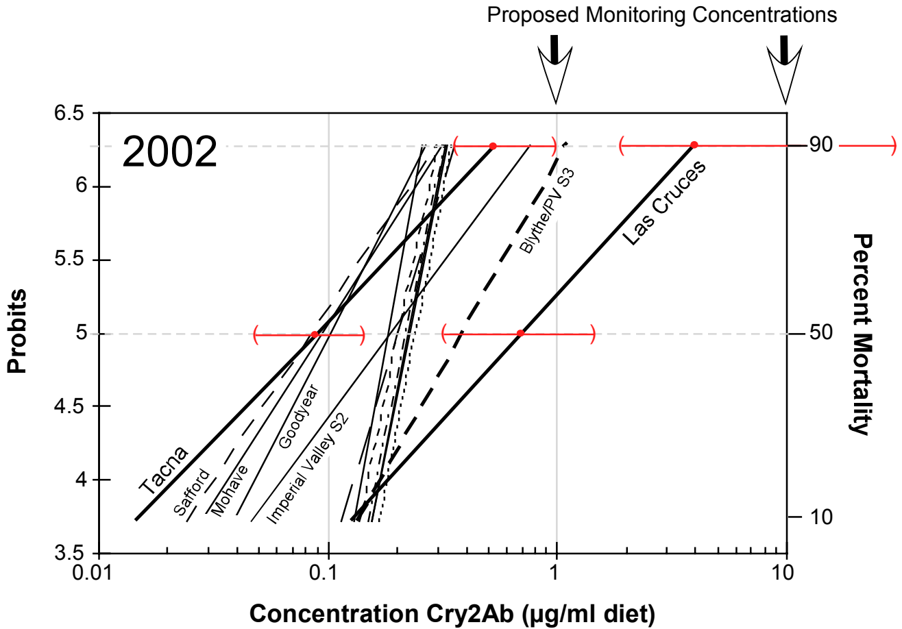
Figure 3. Susceptibility to Cry2Ab of pink bollworm collections made in 2002 in Arizona (9 strains), California (3 strains), New Mexico (1 strain), and Texas (1 strain). Probit lines with LC 50 and LC 90 estimates (95% F.L.) were generated using the POLO program (Robertson and Preisler 1992). 2002 results confirmed the conclusion from 2001 monitoring that concentrations of 1.0 and 10 µg Cry2Ab/ml are suitable for routine monitoring of susceptibility to Cry2Ab. Concentration response results and probit analysis estimates for all evaluations are provided in Table 3.
