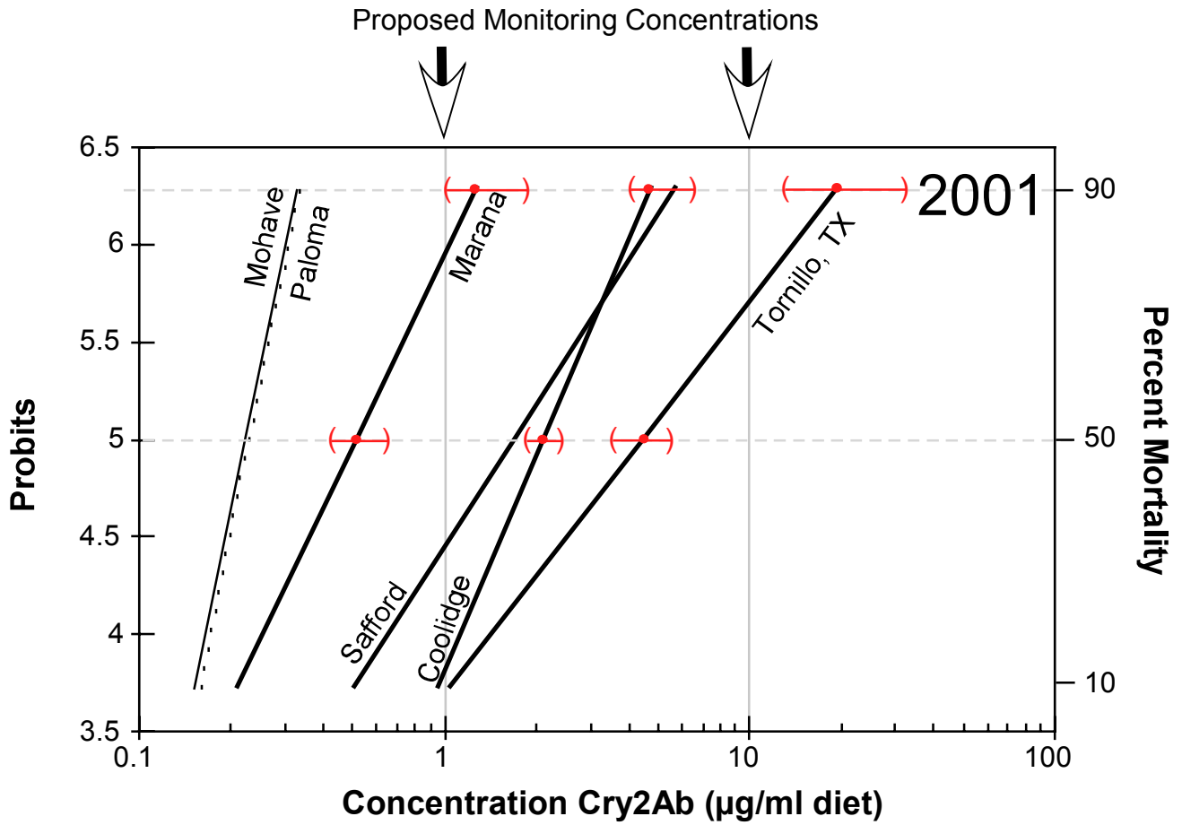
Figure 2. Susceptibility to Cry2Ab of pink bollworm collections made in 2001 in Arizona (5 strains) and Texas (1 strain). Probit lines with LC 50 and LC 90 estimates (95% F.L.) were generated using the POLO program (Robertson and Preisler 1992). Responses indicate that concentrations of 1.0 and 10 µg/ml would be suitable for routine monitoring of susceptibility to Cry2Ab. Concentration response results and probit analysis estimates for all evaluations are provided in Table 2.
