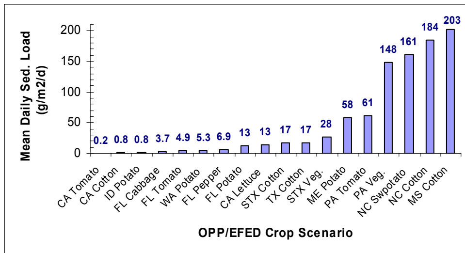
Figure 4.8. Mean daily soil erosion (resulting in sediment loads) from various PRZM scenarios.
