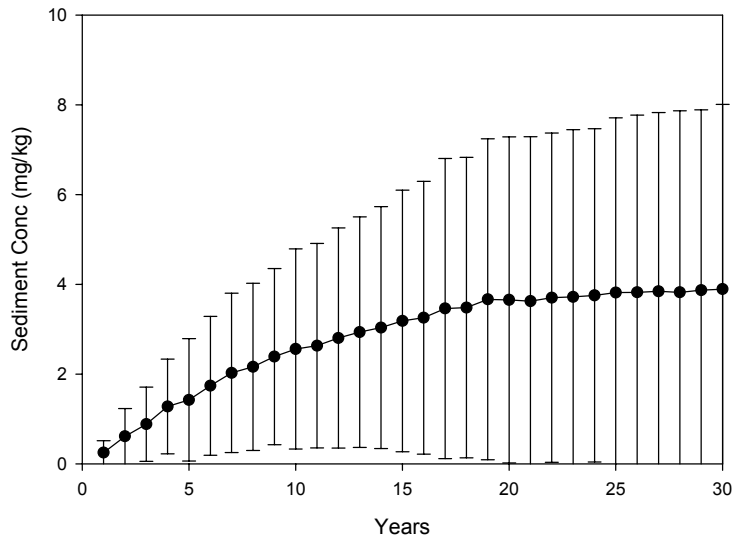
Figure 3.15. PRZM/EXAMS Predicted Mean Sediment Concentration (Standard Deviation) for Representative PRZM/EXAMS Scenarios with Pesticide 4
