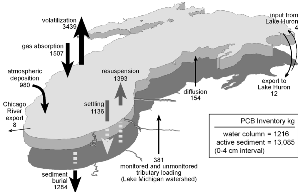
Figure 4.2. Process Diagram: Lake Michigan Mass Balance Project (Source: USEPA, 2006).
