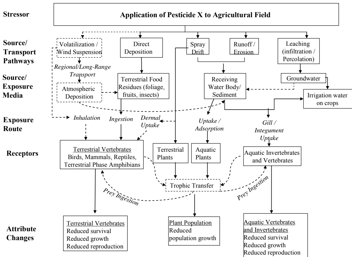
Figure 2.2. Generic Conceptual Model of Pesticide Ecological Risk Assessment by OPP (Dashed sources and pathways are not routinely modeled by OPP/EFED)
