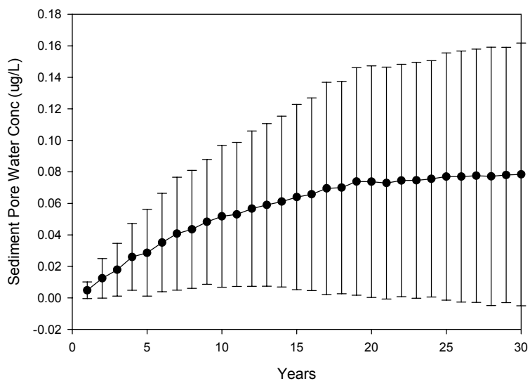
Figure 3.16. PRZM/EXAMS Predicted Mean Sediment Pore Water Concentration (Standard Deviation) for Representative PRZM/EXAMS Scenarios with Pesticide 4
