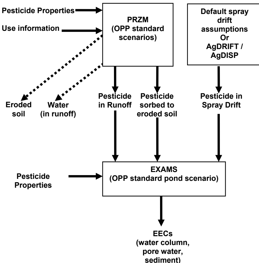
Figure 4.4. Diagram of OPP/EFED Aquatic Ecological Exposure Modeling Scheme. (Dashed lines represent PRZM outputs that are not included as inputs to the Standard Pond.)
