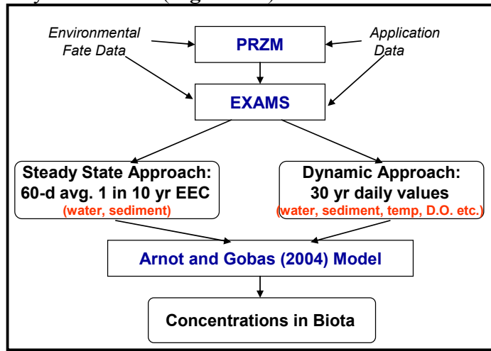
Figure 5.3. Bioaccumulation Modeling Approach Using PRZM/ EXAMS/Arnot & Gobas Models for Pesticide 3
