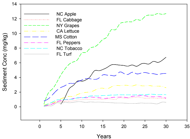
Figure 3.14. PRZM/EXAMS Predicted Accumulation in Sediment for Representative PRZM/EXAMS Scenarios for Pesticide 4
