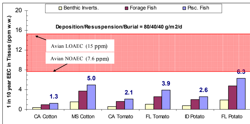
Figure 5.10. Tissue-Based EECs for Pesticide 3 Determined from Bioaccumulation Approach 3
