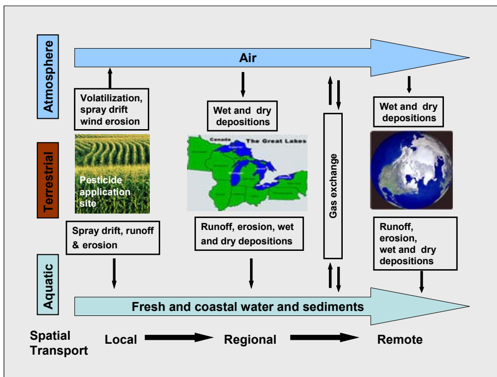
Figure 6.1. Conceptual Model Depicting Long-range Transport Potential of Persistent Substances
