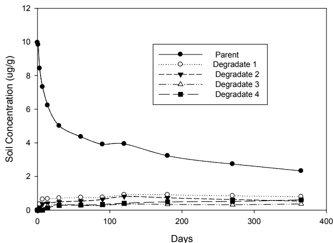
Figure 3.2. Degradation Pattern of Pesticide 2 in an Aerobic Soil Metabolism Study
