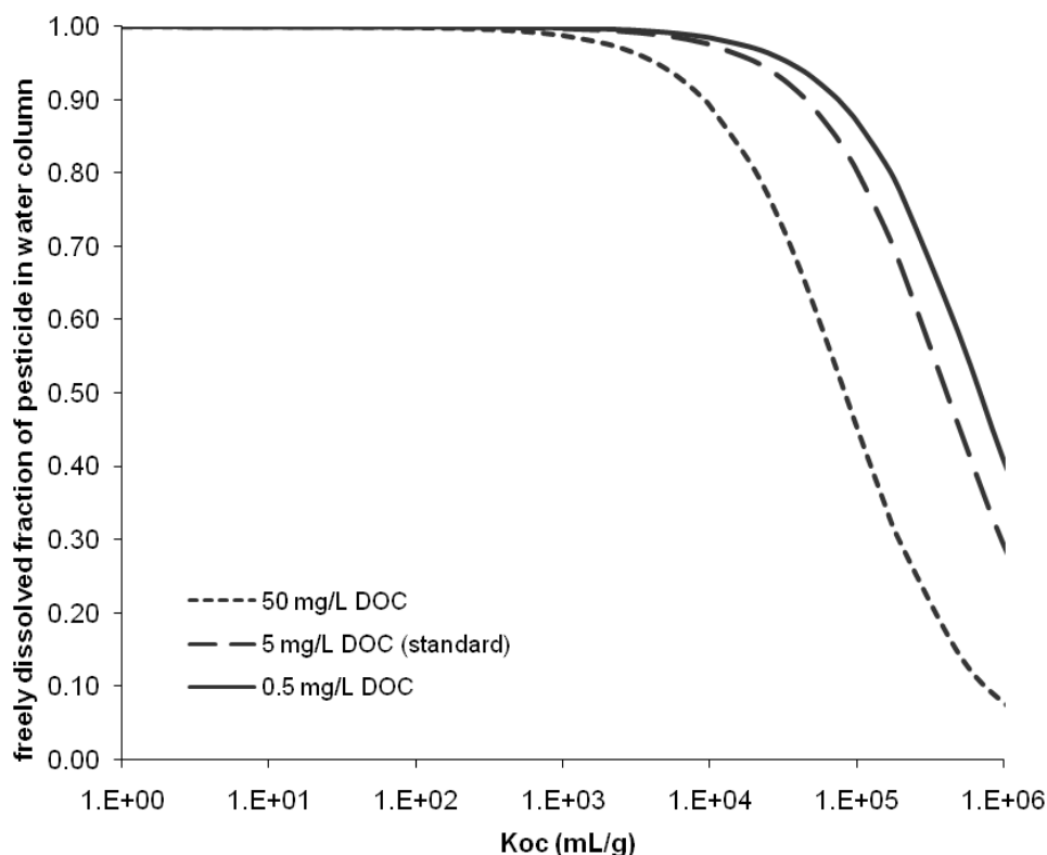
Figure 4.10. Freely Dissolved Fraction of Pesticide in Water Column at Different K_{OC} and DOC Concentrations. (Concentrations of suspended sediment and biota (30 and 0.4 mg/L, respectively), are consistent with the standard pond).
