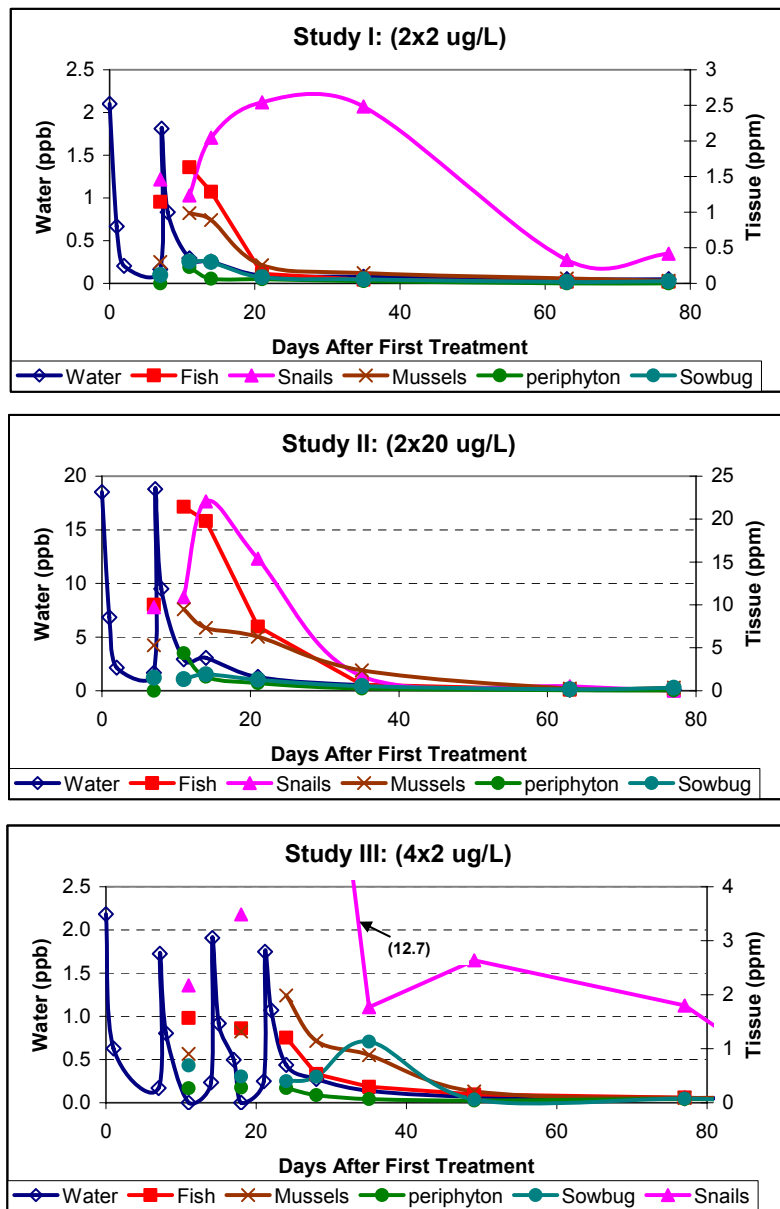
Figure 5.2. Results from a Mesocosm Study with Pesticide 3
