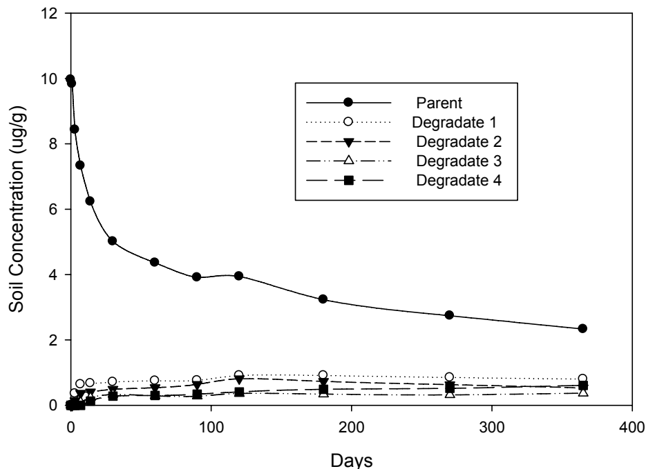
Figure 3.7. Degradation Profile of Pesticide 2
