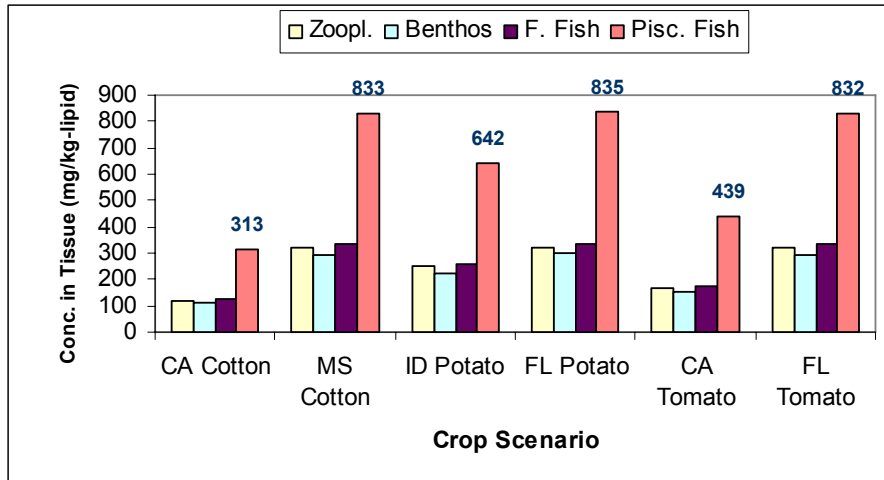
Figure 5.6. Lipid-Normalized Concentrations of Pesticide 3 in Aquatic Biota
