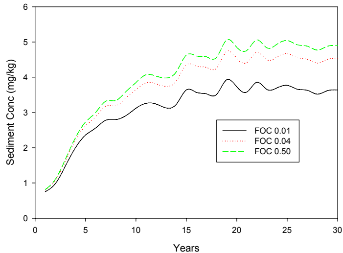
Figure 3.17. PRZM/EXAMS Predicted Pesticide 4 Accumulation in Sediment for the MS Cotton Scenario
