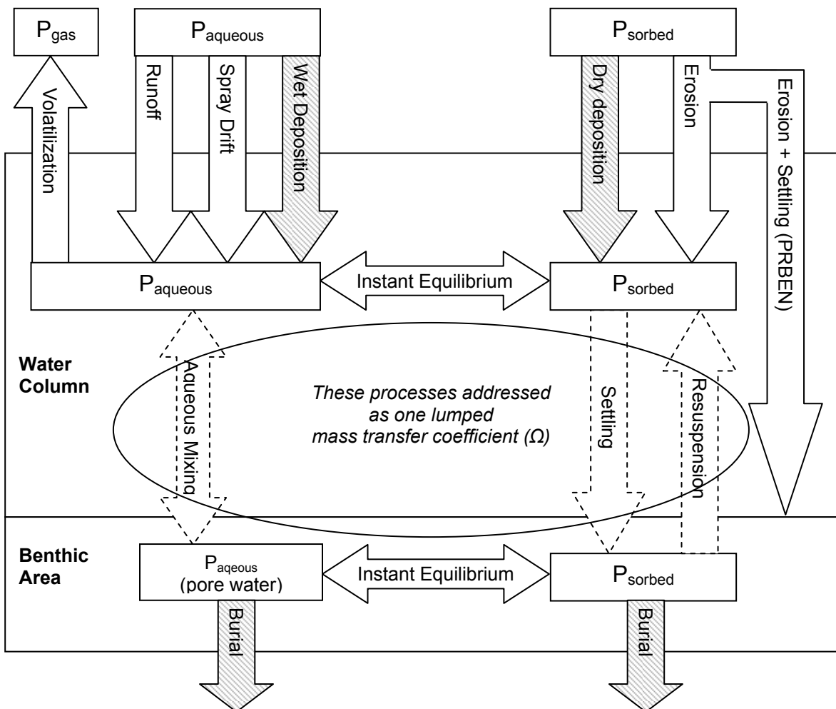
Figure 4.5. Conceptual model of OPP Standard Pond Scenario for Depicting Pesticide Transport (P). Arrows represent movement of pesticide mass from one phase ( i.e. , sorbed or aqueous) or compartment to another. In this figure, P_{\text{aqueous}} =aqueous mass of pesticide; P_{\text{sorbed}} = sorbed mass of pesticide; and P_{\text{gas}} = gaseous mass of pesticide.
