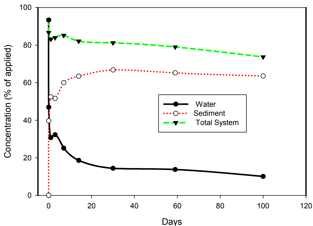
Figure 3.12. Concentrations of Pesticide 3 in the water column, sediment, and total system of aerobic aquatic metabolism studies
