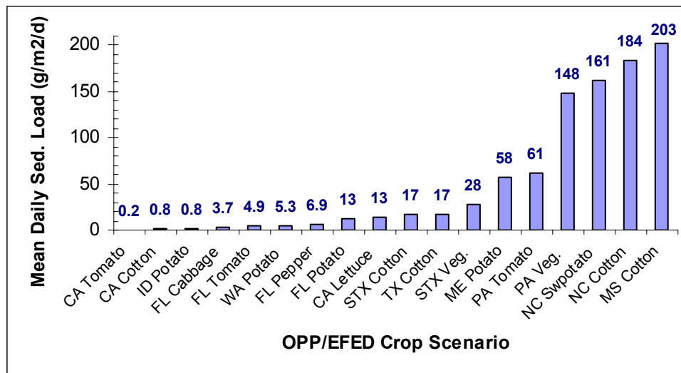
Figure 5.11. Mean Daily PRZM-predicted Soil Erosion for 18 Crop Scenarios
