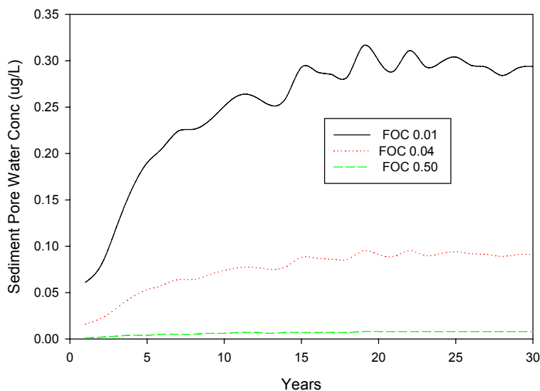
Figure 3.18. PRZM/EXAMS Predicted Pesticide Enrichment of Pore Water of Pesticide 4 for the MS Cotton Scenario
