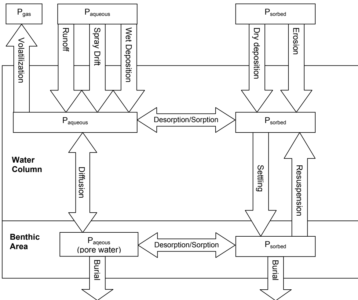
Figure 4.1. Conceptual Model of Pesticide Transport Within A Lentic Aquatic Ecosystem. Arrows represent movement of mass from one phase ( i.e. , sorbed or aqueous) or region to another. Aquatic ecosystems are conceptualized as comprising a water column and a benthic region. In this figure, P_{\text{aqueous}} =aqueous mass of pesticide; P_{\text{sorbed}} = sorbed mass of pesticide; and P_{\text{gas}} = gaseous mass of pesticide.
