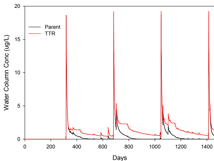
Figure 3.8. Time Series Comparison for the Pesticide 2 TROC Modeling Strategies
