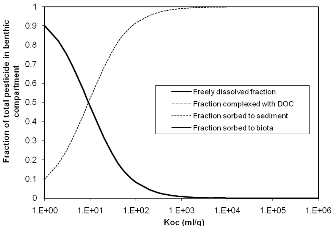
Figure 4.7. Calculated Fractions of Pesticide in the Benthic Compartment of the Standard Pond in Different Phases as a function of K_{OC} .
