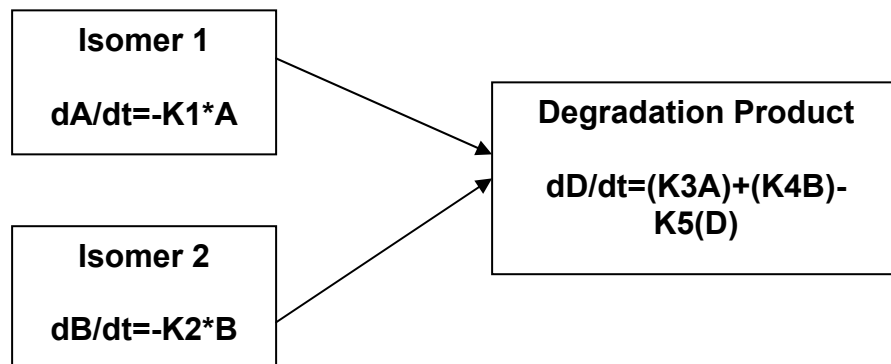
Figure 3.4. Schematic of Simultaneous Formation / Decline Kinetics Approach for Pesticide 1
