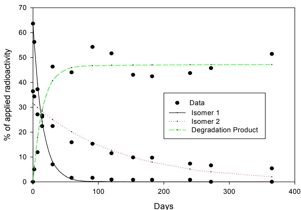
Figure 3.5. Model Simultaneous Degradation of Pesticide 1 and Formation of the Toxic Degradation Product Using Simultaneous Formation Decline Kinetics
