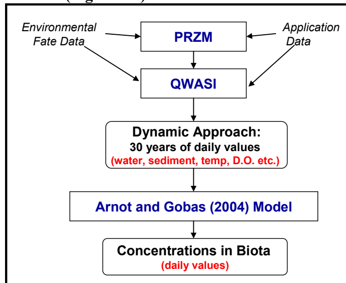
Figure 5.4. Schematic of AGRO Aquatic Bioaccumulation Modeling System
