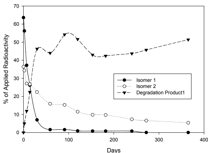
Figure 3.1. Degradation Pattern of Pesticide 1 in an Aerobic Soil Metabolism Study
