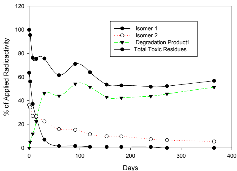
Figure 3.3. Pesticide 1 Degradation Pattern in an Aerobic Soil Metabolism Study
