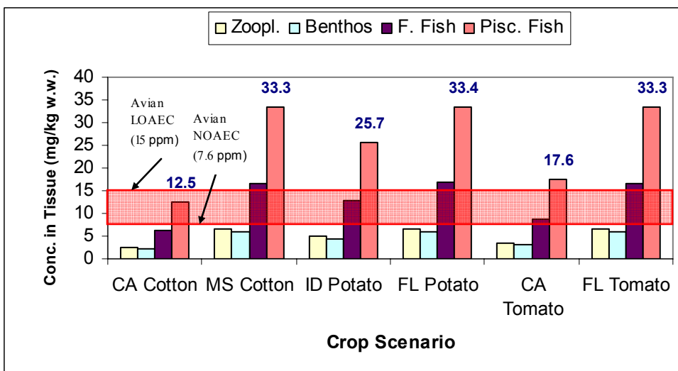
Figure 5.5. Steady State Bioaccumulation Modeling Results for Pesticide 3
