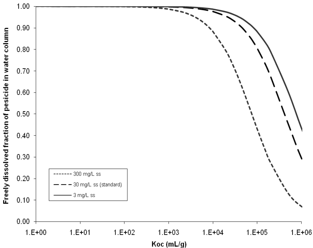
Figure 4.9. Freely Dissolved Fraction of Pesticide in Water Column at Different K_{OC} and Suspended Sediment (Ss) Concentrations. (Concentrations of DOC and biota (5 and 0.4 mg/L, respectively), are consistent with the standard pond.)
