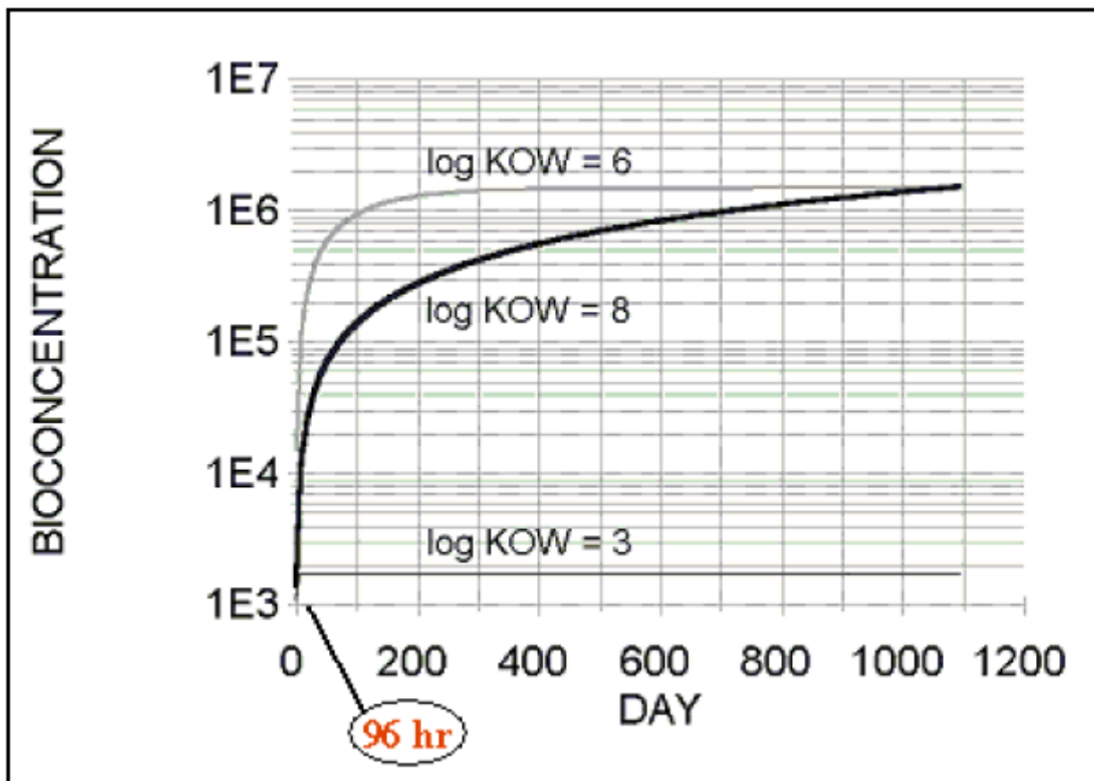
Figure 7.1. Bioconcentration as a function of time and K_{ow}
