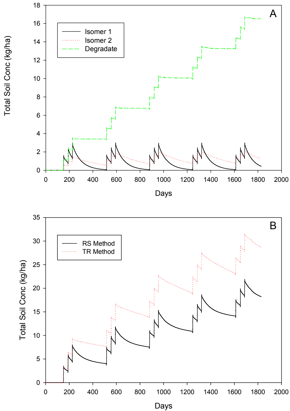
Figure 3.13. PRZM Time Series for Total Soil Concentration of Pesticide 1 Residues in a FL Tomato Scenario (A= Individual Residues from RS Method; B= RS and TR Methods)
