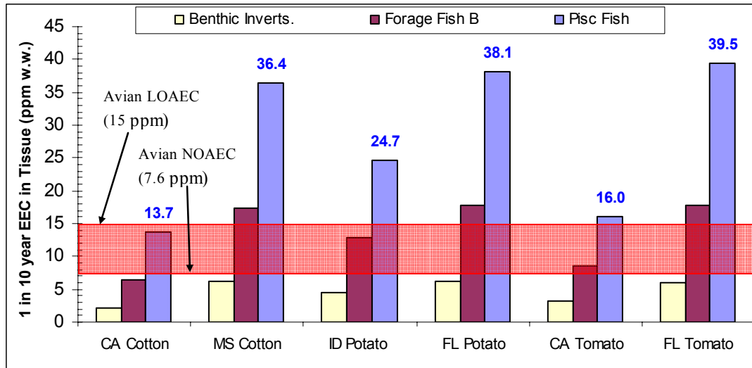
Figure 5.8 Tissue-Based EECs for Pesticide 3 Using Bioaccumulation Approach 2
