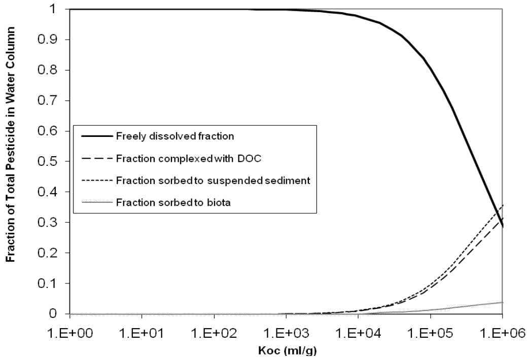
Figure 4.6. Calculated Fraction of Pesticides in the Water Column of the Standard Pond in Different Phases as a function of K_{OC} .
