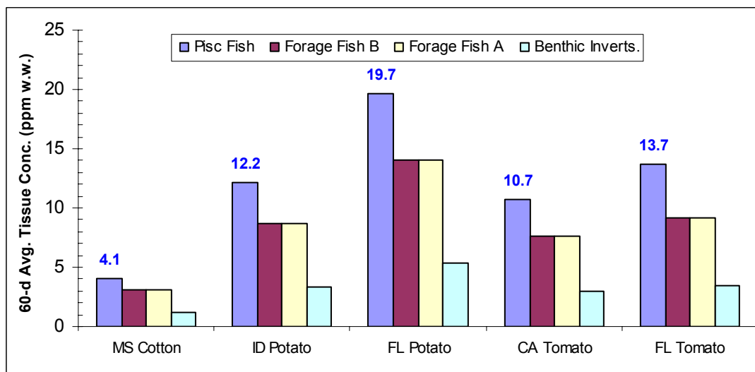
Figure 5.13. Effect of Alternate Assumptions Regarding Rates of Deposition, Resuspension and Burial (PRZM Values) on Tissue-based EECs for Pesticide 3
