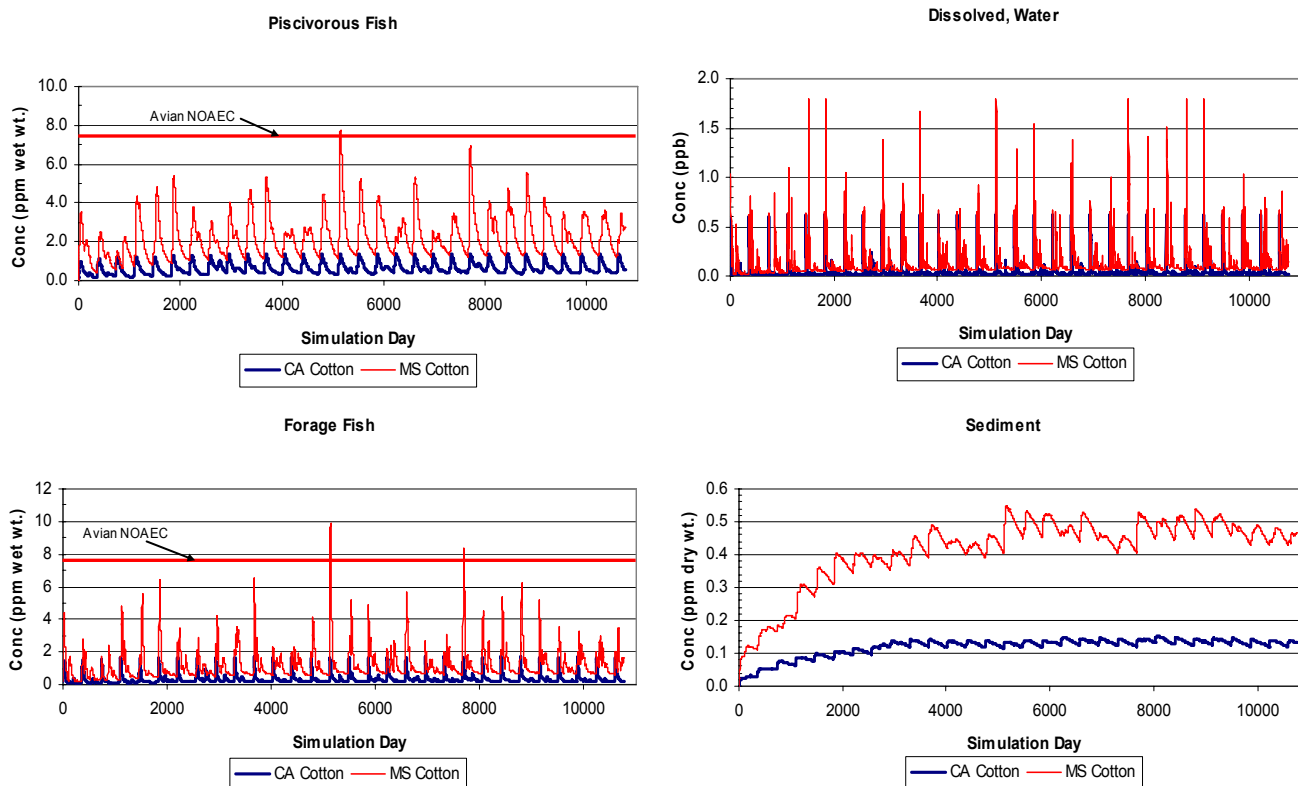
Figure 5.9. Pesticide 3 Modeling Results using Approach 3 (PRZM/QWASI/Arnot & Gobas)
