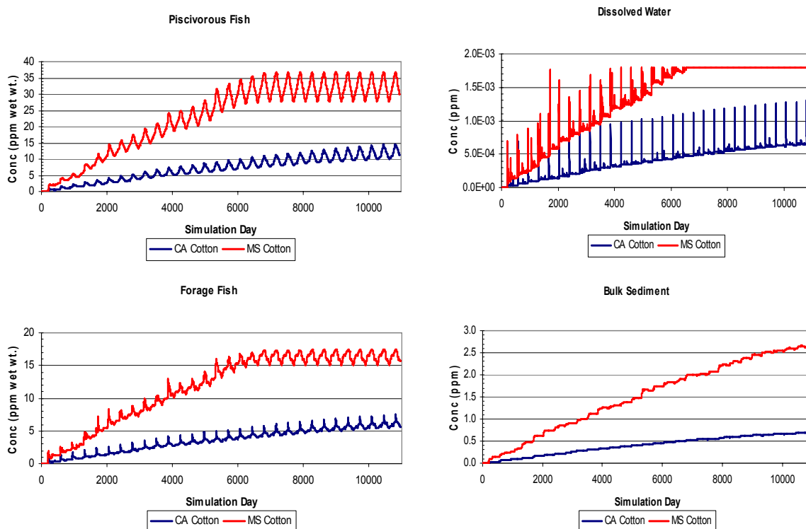
Figure 5.7 Dynamic Bioaccumulation Modeling Results for Pesticide 3 Using Approach 2
