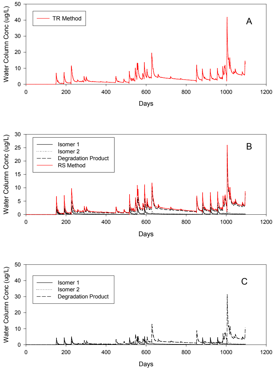
Figure 3.6. Time Series of TROC Modeling Strategies for Pesticide 1 (A = Total Residue; B=Residue Summation; C=Simultaneous Formation Decline Kinetics)
