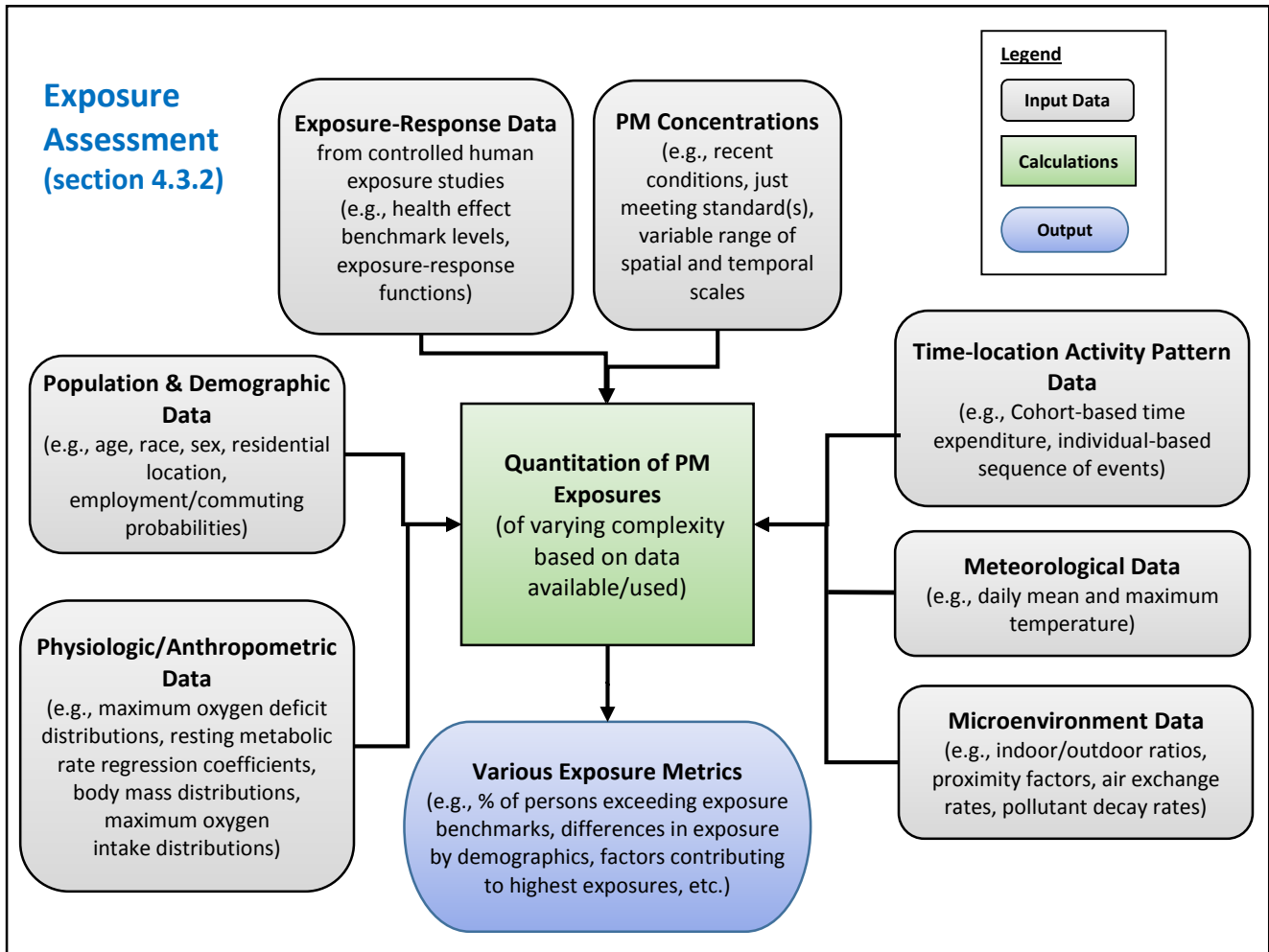
Figure 4-3. Analytical approach for the microenvironmental exposure analysis.
