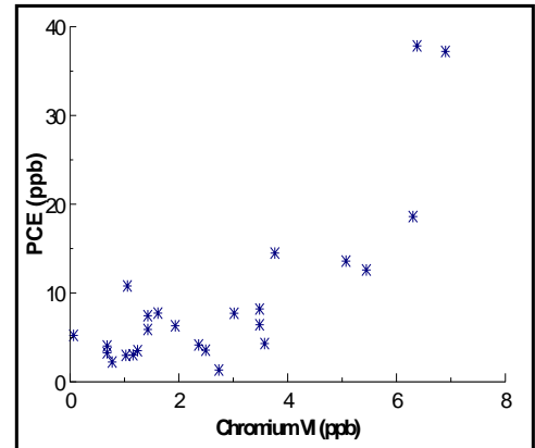
Example Scatter Plot
