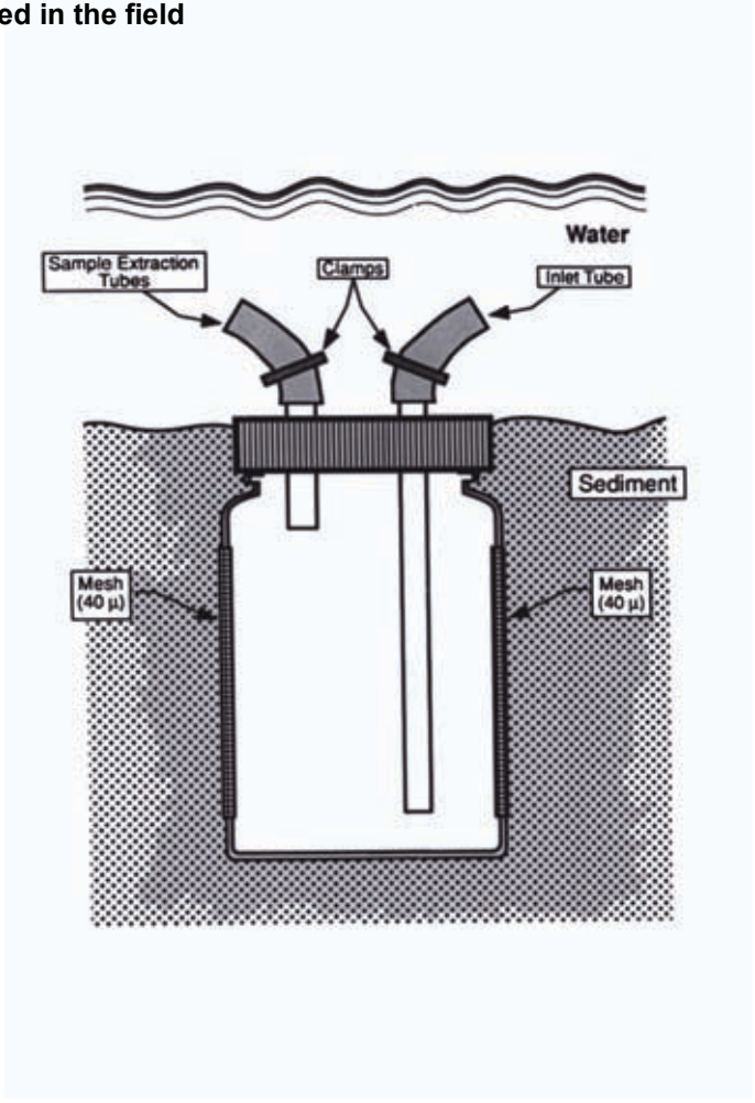
General peeper design with in-situ sample extraction
