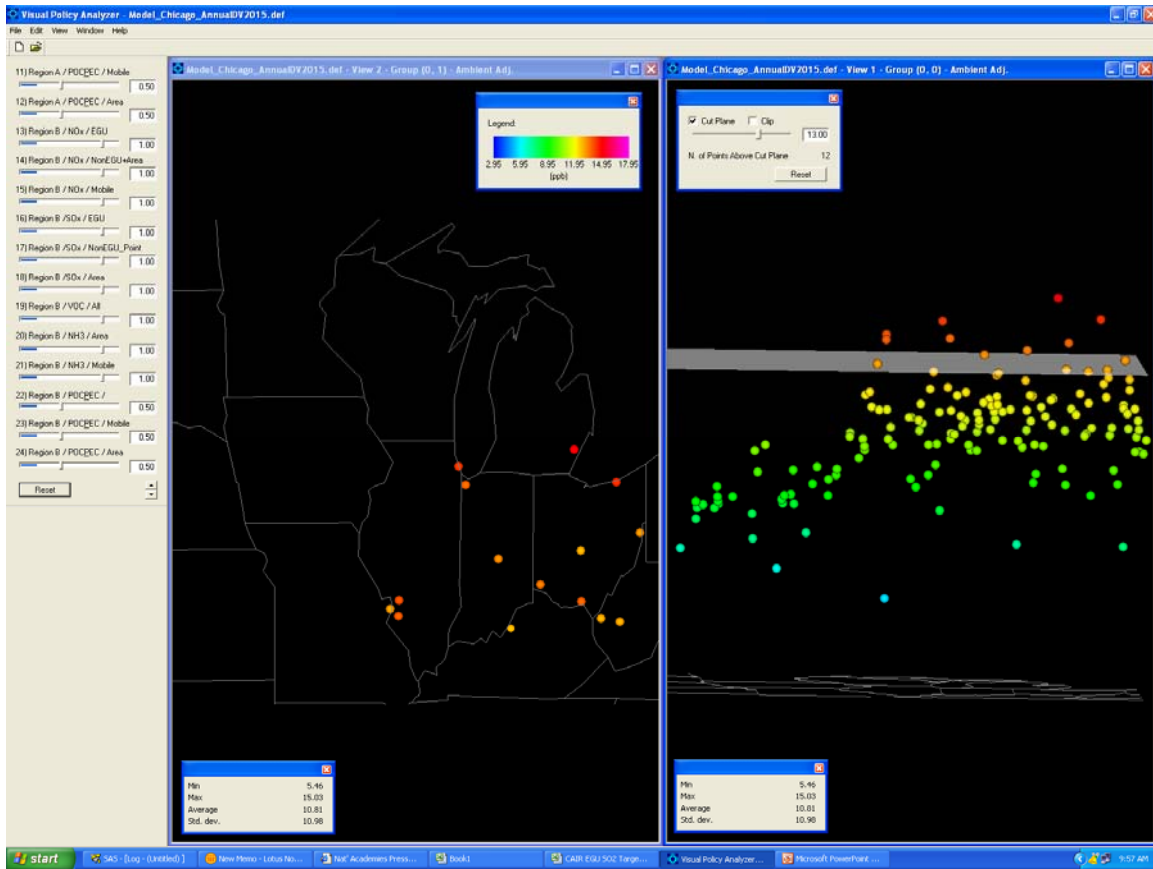
Figure III-8. VPA example: Monitors with annual average PM 2.5 Post CAIR 2015 greater than 13 \mu\text{g}/\text{m}^3 after applying 50 percent reduction in carbon.
