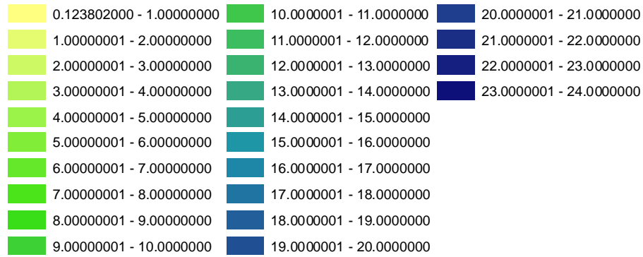
Figure IV-5. PM 2.5 spatial gradient map for RSM predictions for October mean total PM 2.5 based on Run 120.
