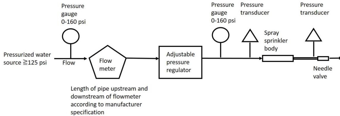
Figure 1. Equipment Setup for Pressure Regulation Test
