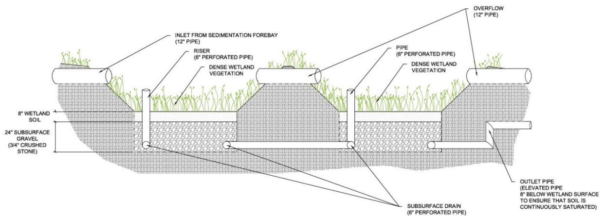
Figure 23. Gravel Wetland Schematic.
