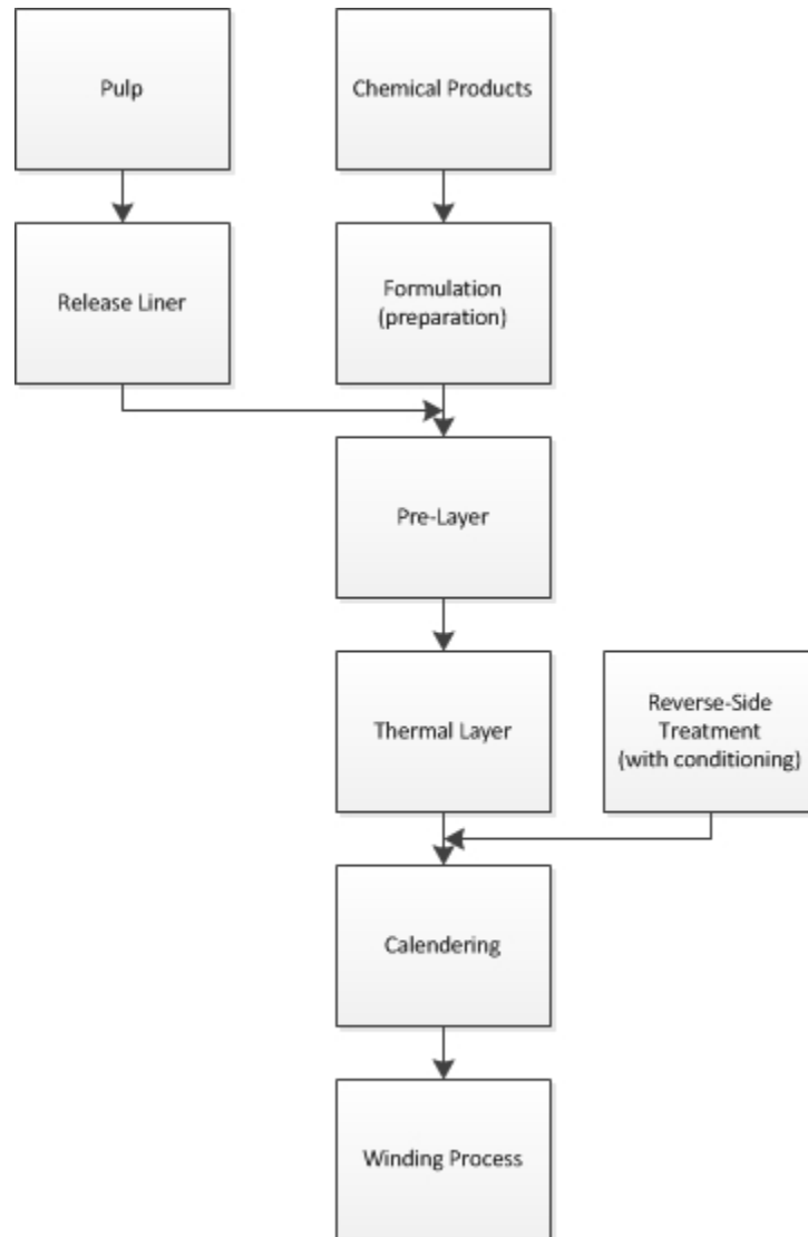
Figure 5-3: The Production Process for Thermal Paper
