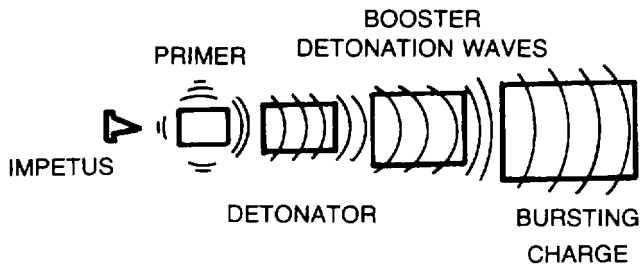
Figure 3-1. Explosive train.
