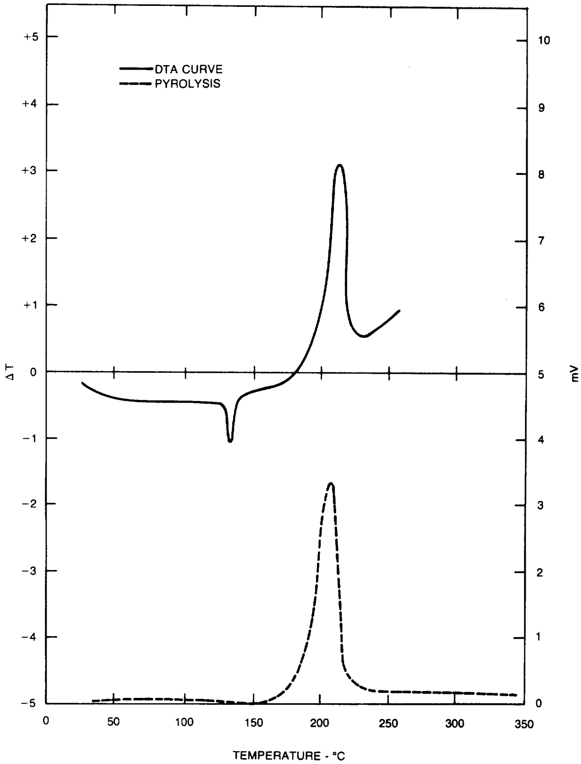
Figure 8-39. DTA curve for tetryl.
