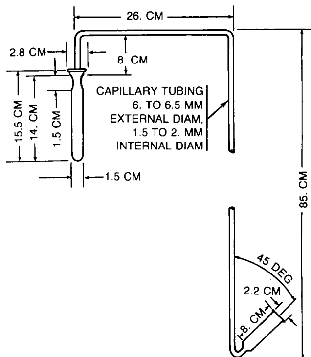
Figure 5-1. Vacuum stability test.
