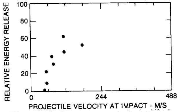
Figure 8-85. Susan test results for LX-74.
