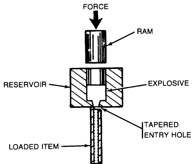
Figure 8-91. Injection loading operation.
