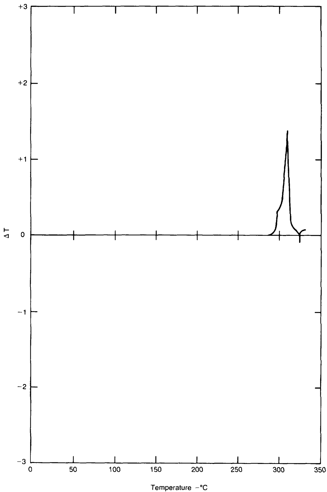
Figure 7-2. DTA curve for lead azide.
