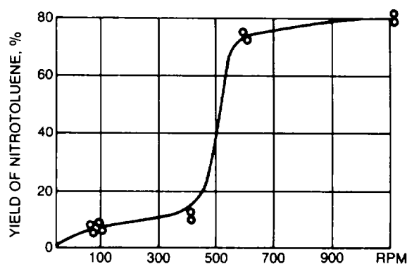
Figure 8-66. Agitation versus MNT yield.
