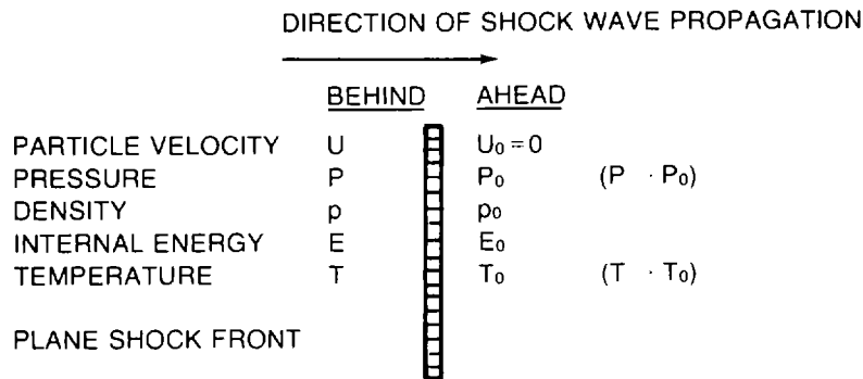
Figure 4-2. Steady plane shock front.
