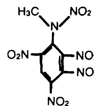
Figure 8-30. Trinitrophenyl methylamine.
