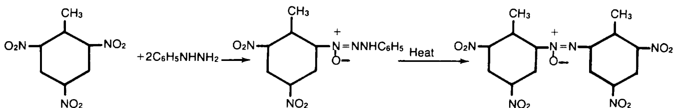
Figure 8-65. Reaction of TNT with phenylhydrazine.
