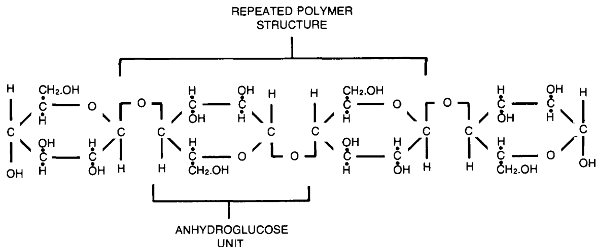
Figure 8-3. Cellulose.
