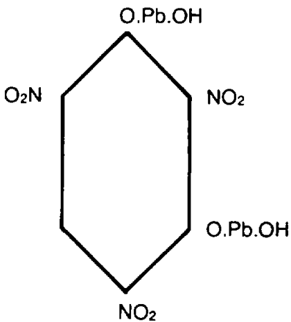
Figure 7-5. Basic lead styphnate.
