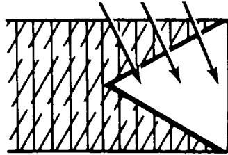
A. LINER IS ACCELERATED NORMAL TO EXPLOSIVE-LINER INTERFACE
