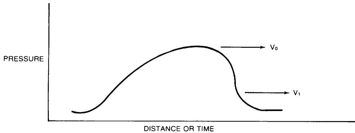
B. DIFFERENTIAL VELOCITY CAUSES THE LEADING EDGE TO BECOME SHARPER
