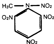
Figure 8-29. Structural formula for tetryl.
