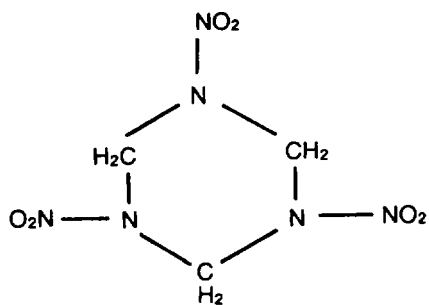
Figure 8-18. Structural formula for RDX.
