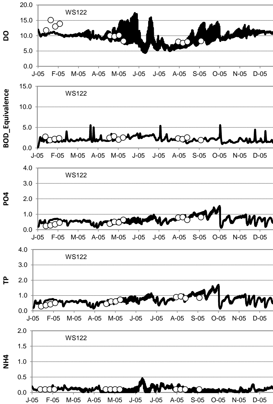
Figure G-3. EFDC Water quality calibration at WS122.
