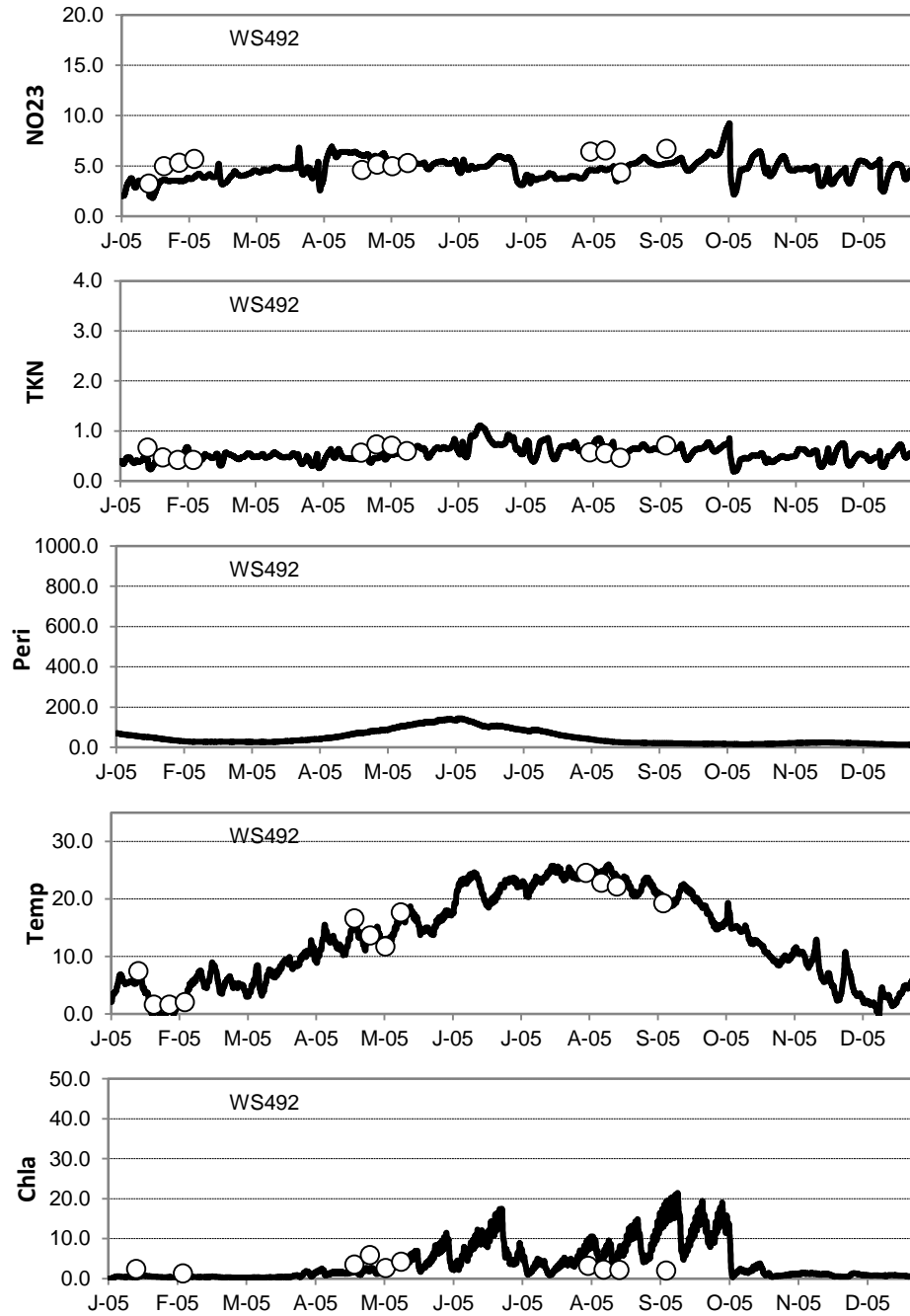
Figure G-5 (continued). EFDC Water quality calibration at WS492.
