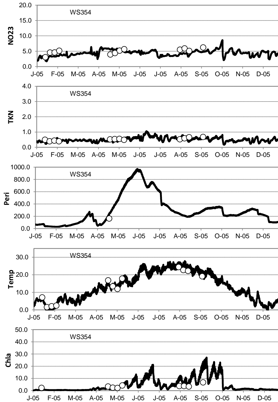
Figure G-4 (continued). EFDC Water quality calibration at WS354.
