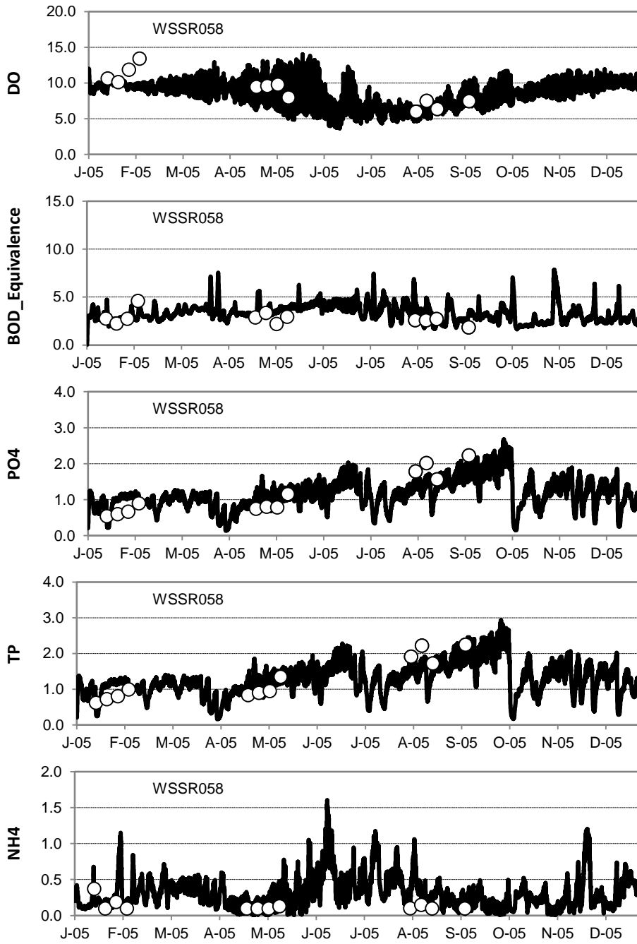
Figure G-1. EFDC Water quality calibration at WSSR058.
