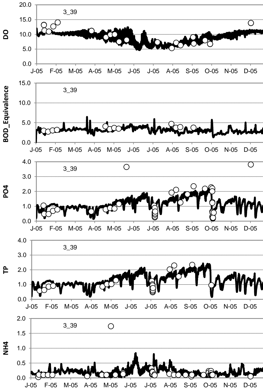
Figure G-7. EFDC Water quality calibration at 3_39.
