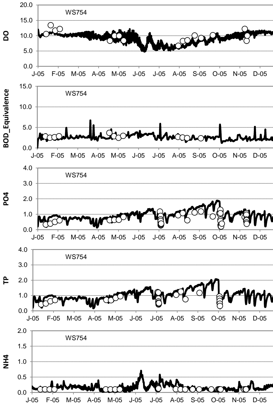
Figure G-6. EFDC Water quality calibration at WS754.
