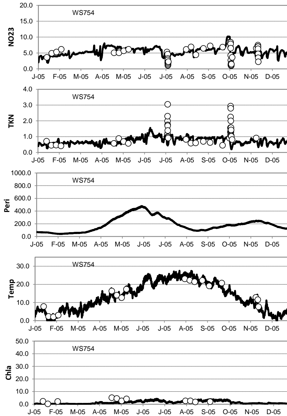
Figure G-6 (continued). EFDC Water quality calibration at WS754.
