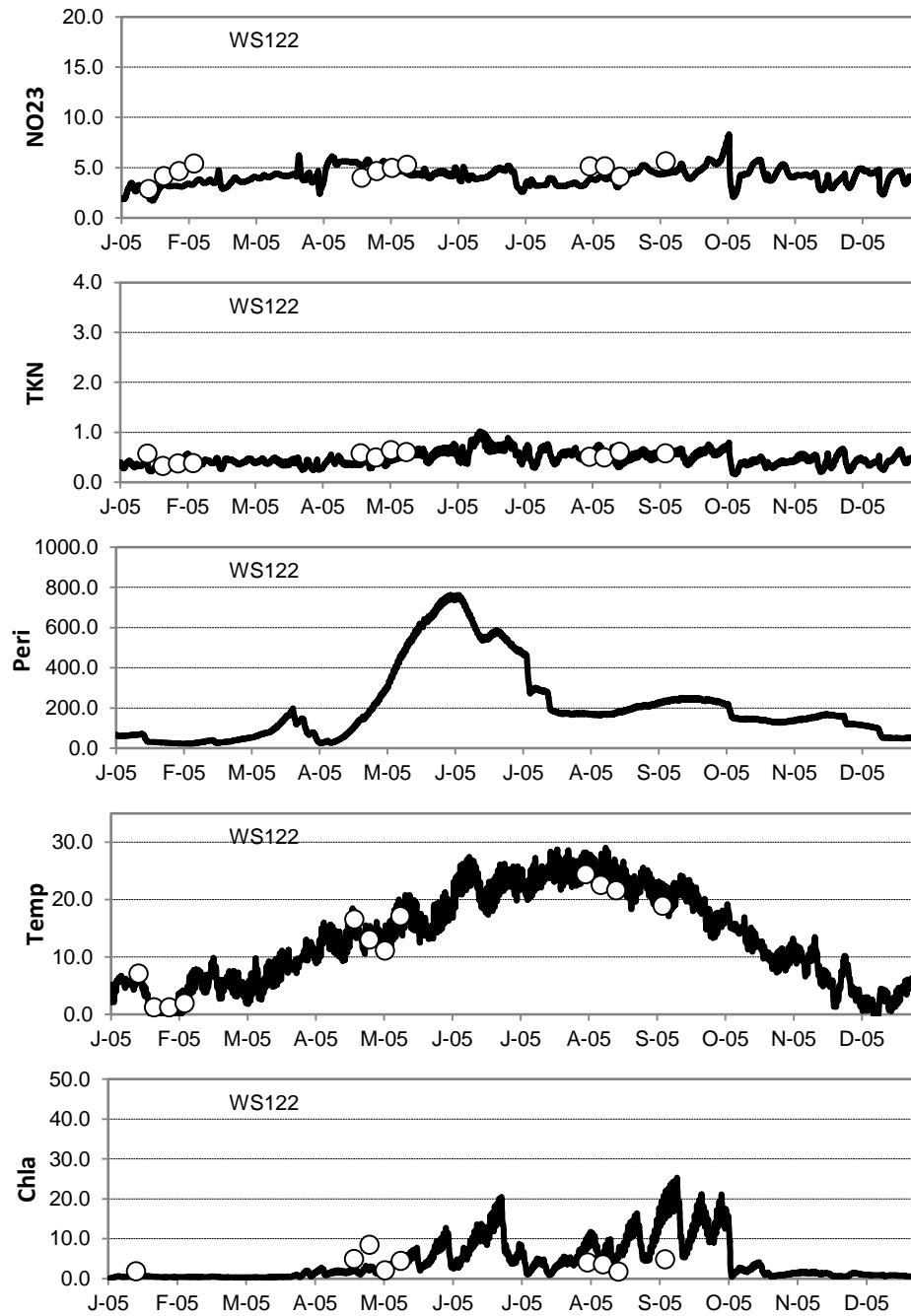
Figure G-3 (continued). EFDC Water quality calibration at WS122.
