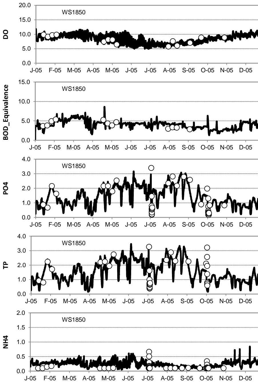
Figure G-9. EFDC Water quality calibration at WS1850.
