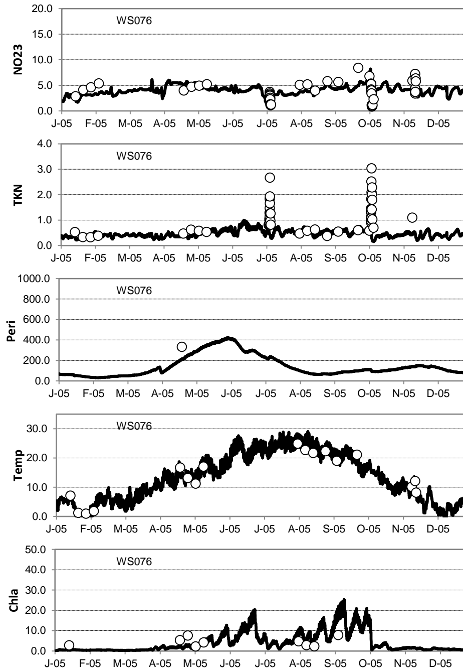
Figure G-2 (continued). EFDC Water quality calibration at WS076.
