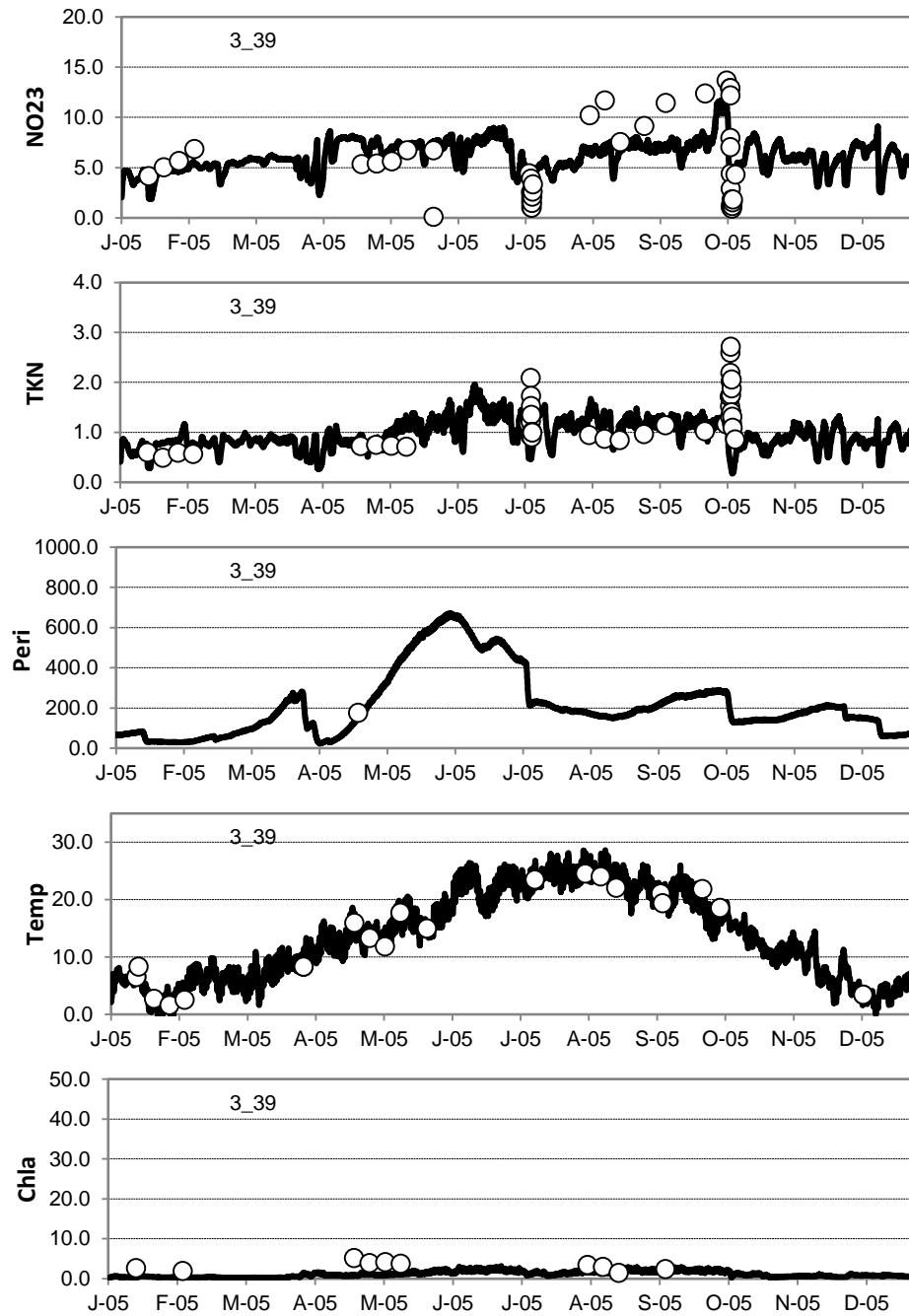
Figure G-7 (continued). EFDC Water quality calibration at 3_39.
