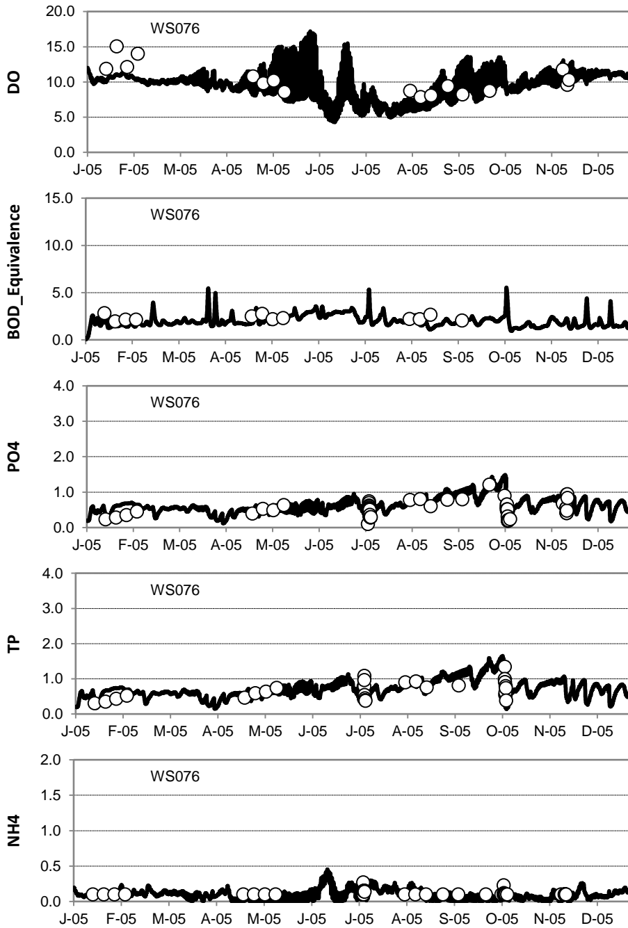
Figure G-2. EFDC Water quality calibration at WS076.
