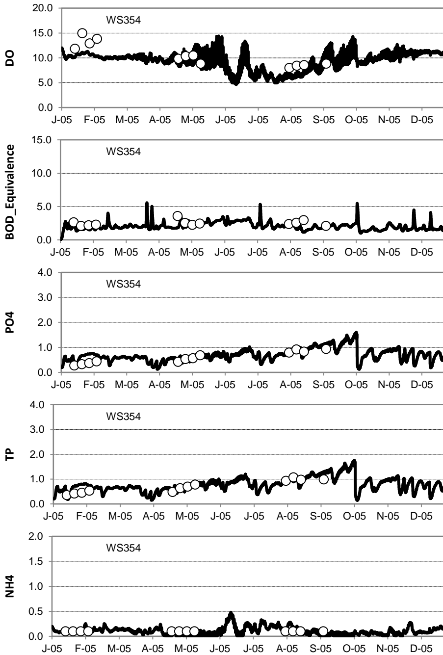
Figure G-4. EFDC Water quality calibration at WS354.
