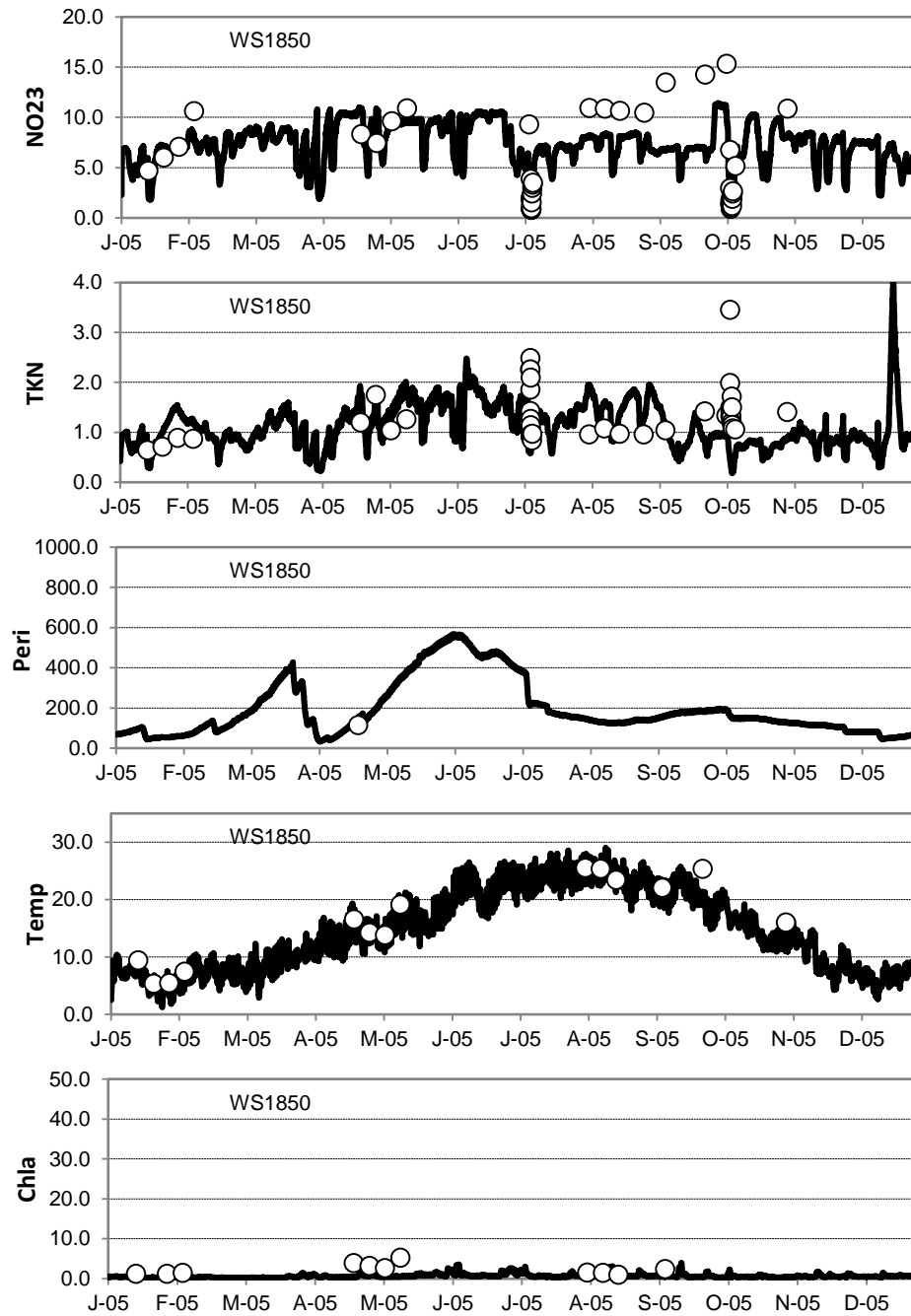
Figure G-9 (continued). EFDC Water quality calibration at WS1850.
