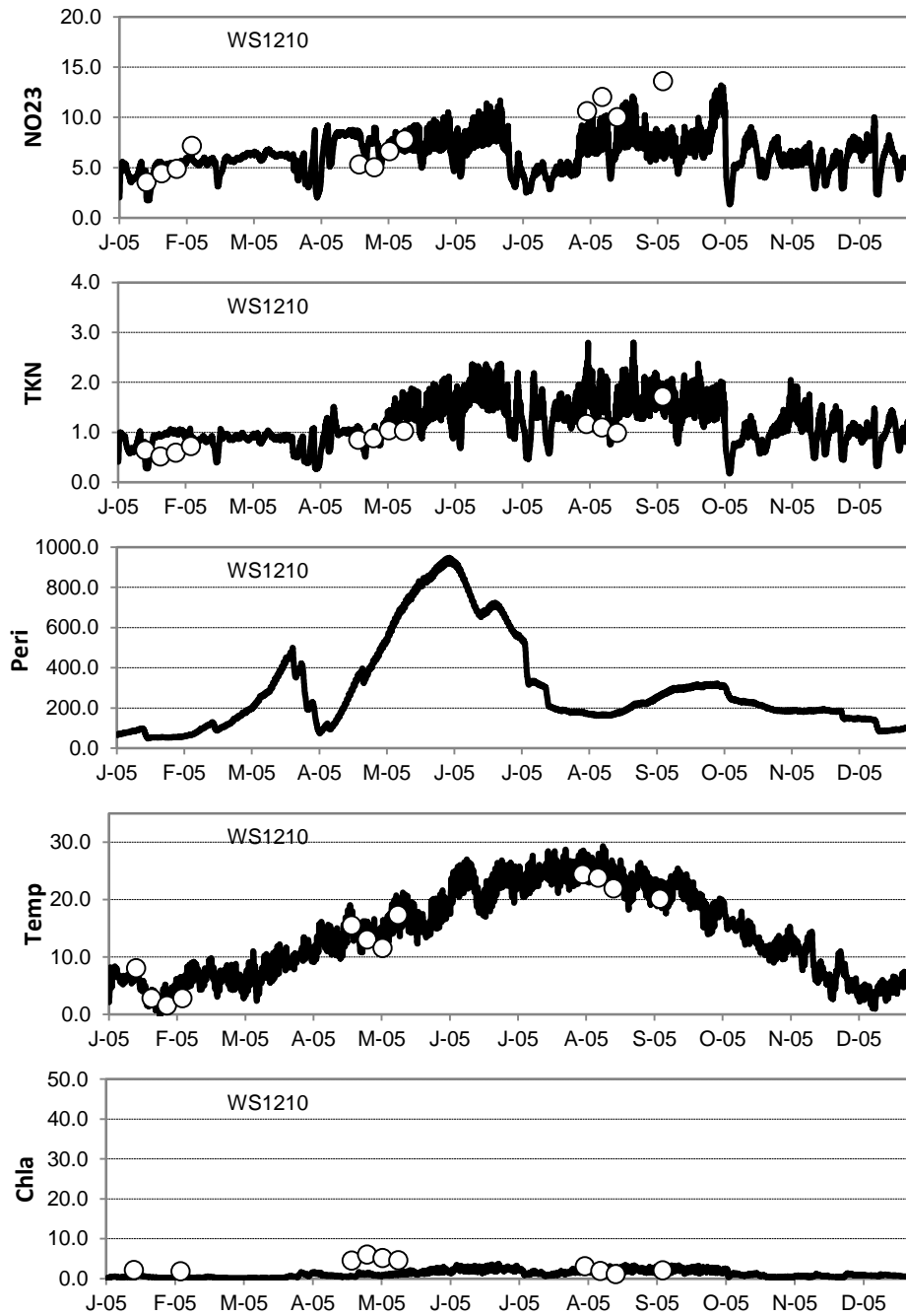
Figure G-8 (continued). EFDC Water quality calibration at WS1210.
