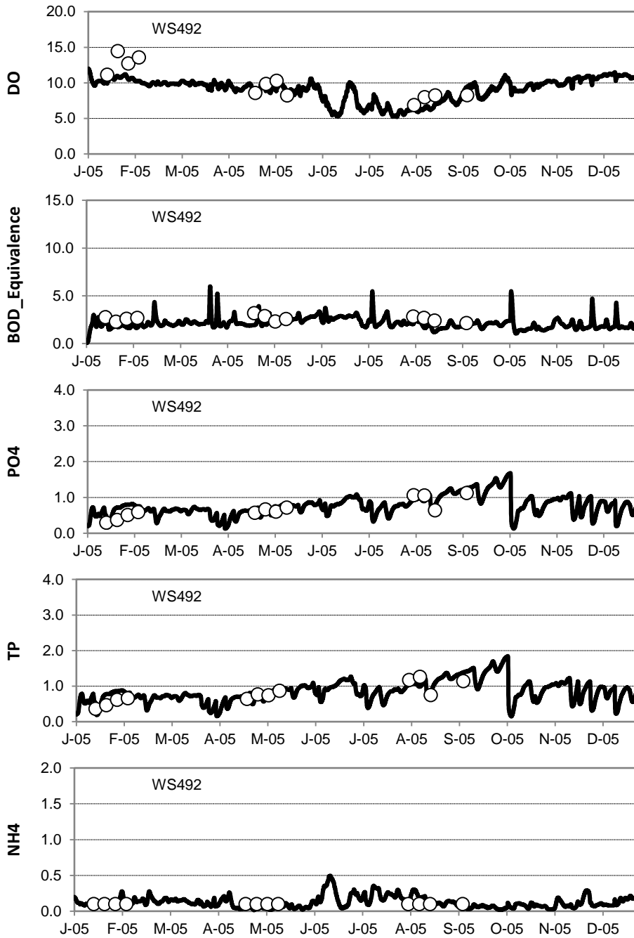
Figure G-5. EFDC Water quality calibration at WS492.
