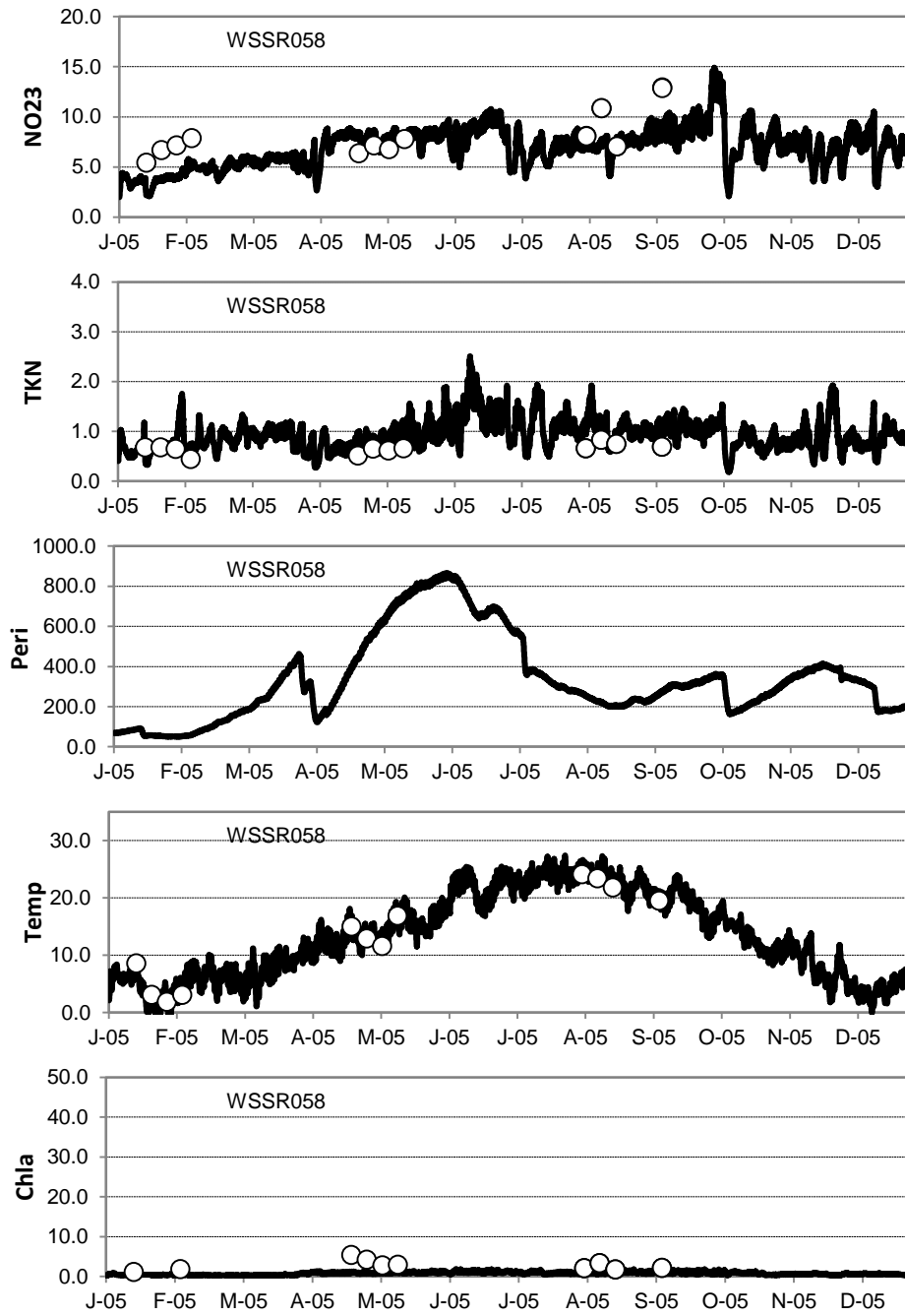
Figure G-1 (continued). EFDC Water quality calibration at WSSR058.
