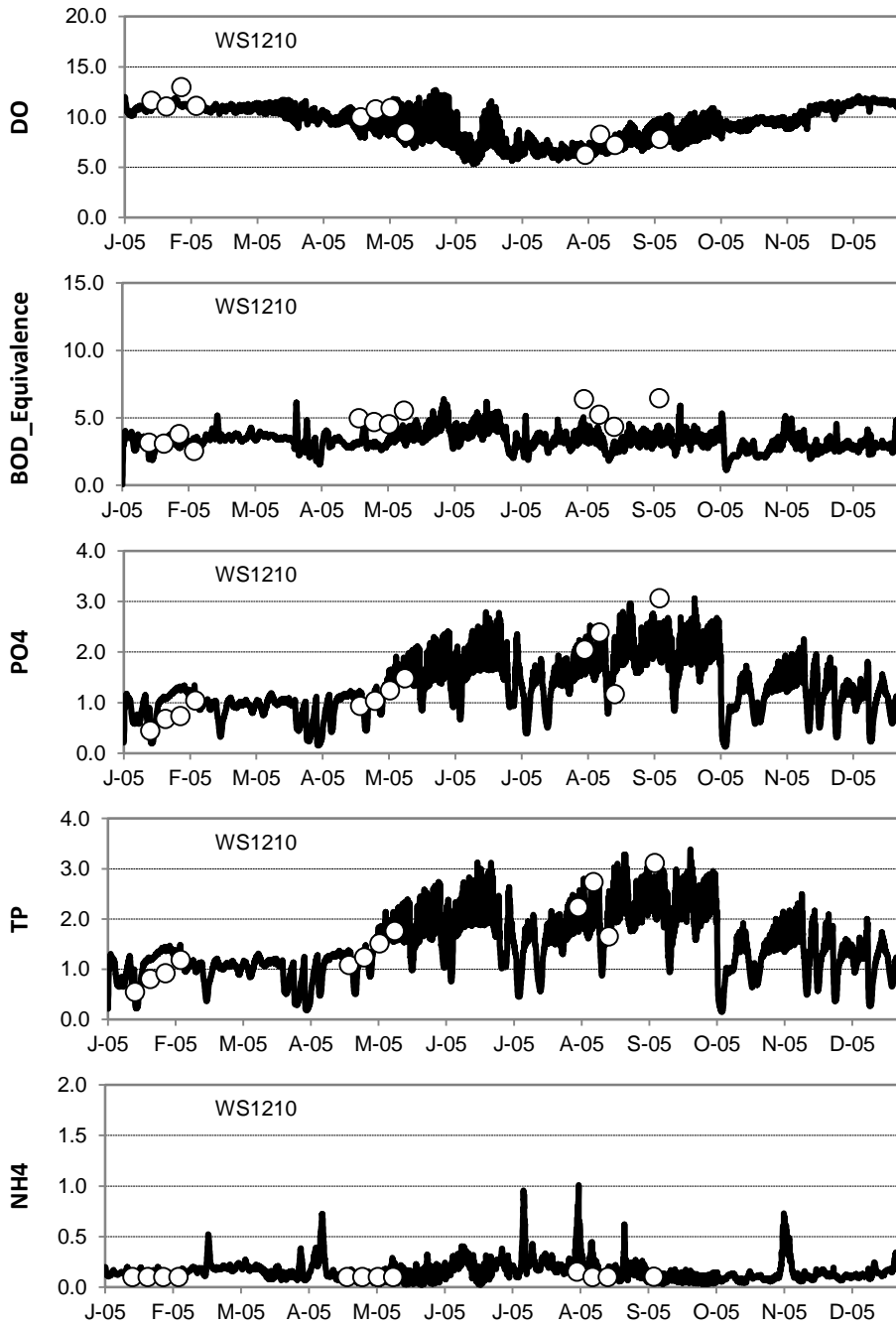
Figure G-8. EFDC Water quality calibration at WS1210.
