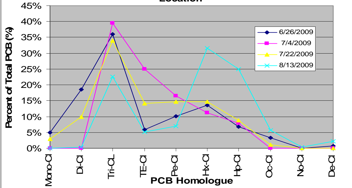
Figure 43. PCB Homologue Data from Storm Flow Samples Collected from the Rio Grande at Otowi Bridge Location
