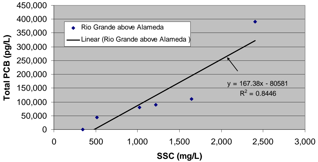
Figure 39. Pearson R 2 correlation between suspended sediment concentration and total PCB at Rio Grande above Alameda
