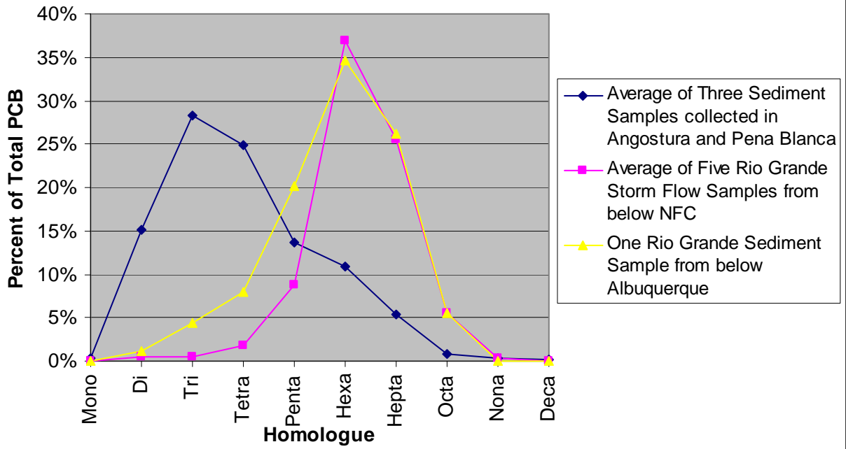
Figure 49. PCB Distribution in Rio Grande Sediments and Storm Flow Samples from Rio Grande above Alameda
