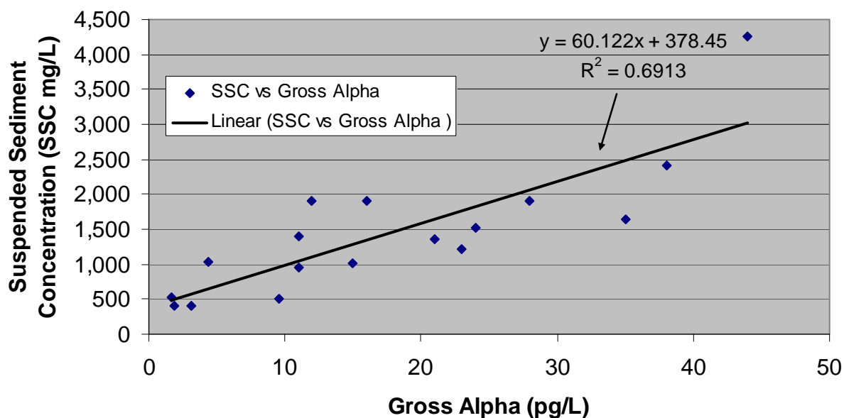
Figure 41. The Pearson R 2 correlation between suspended sediment concentration and gross alpha for all samples (excluding outlier with high sand content)
