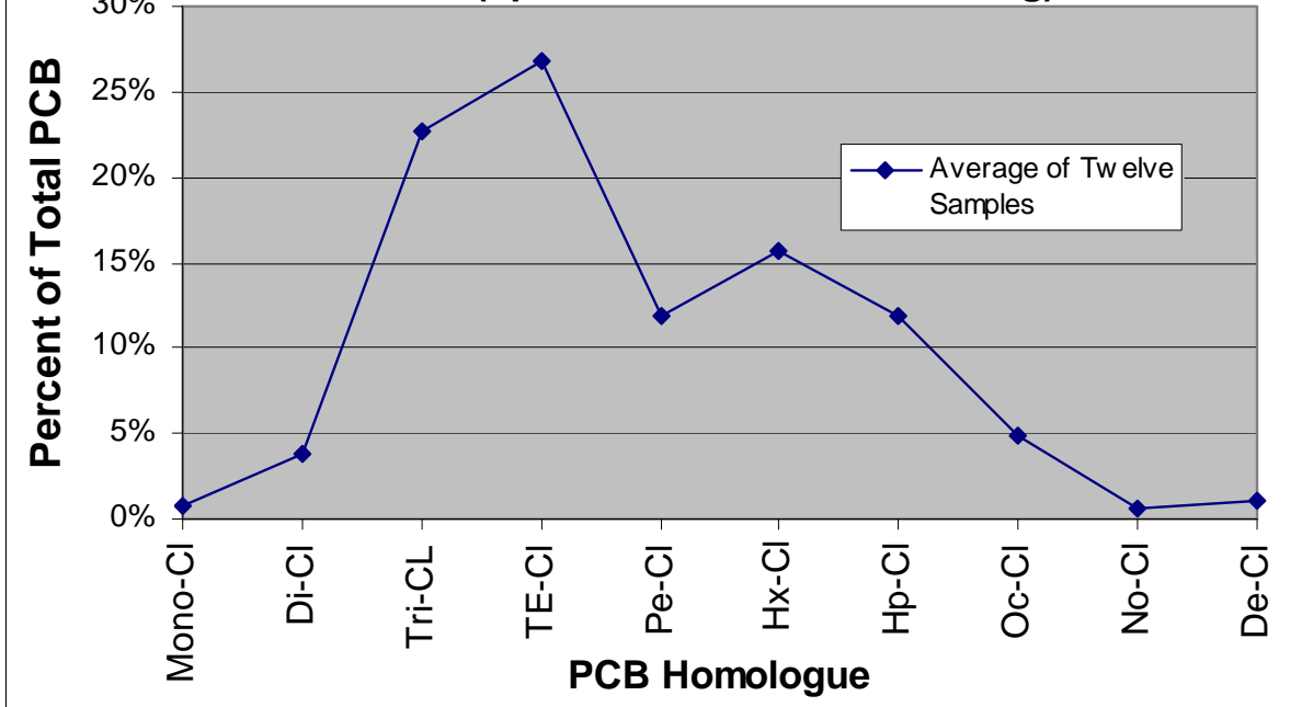
Figure 46. PCB Homologue Data from Storm Flow Samples Collected from the Rio Grande and Chama River Locations (upstream of Buckman Landing)
