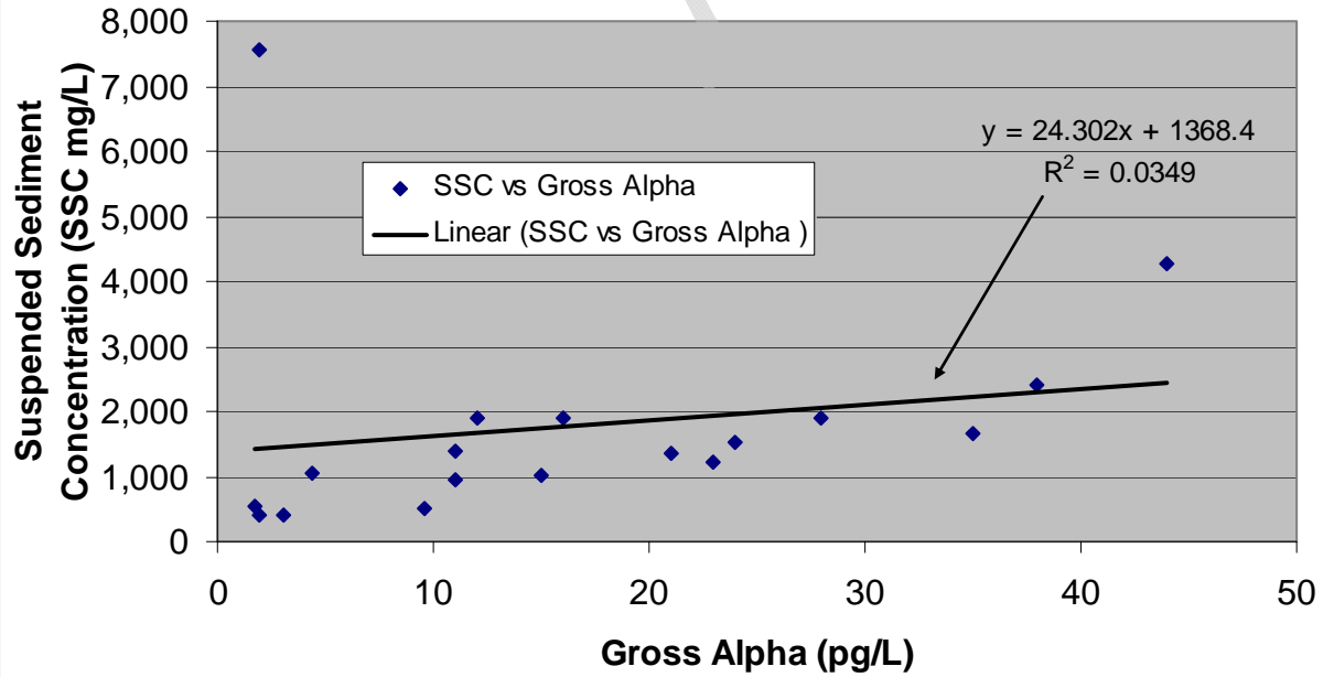
Figure 40. The Pearson R 2 correlation between suspended sediment concentration and gross alpha for all samples (including outlier with high sand content)
