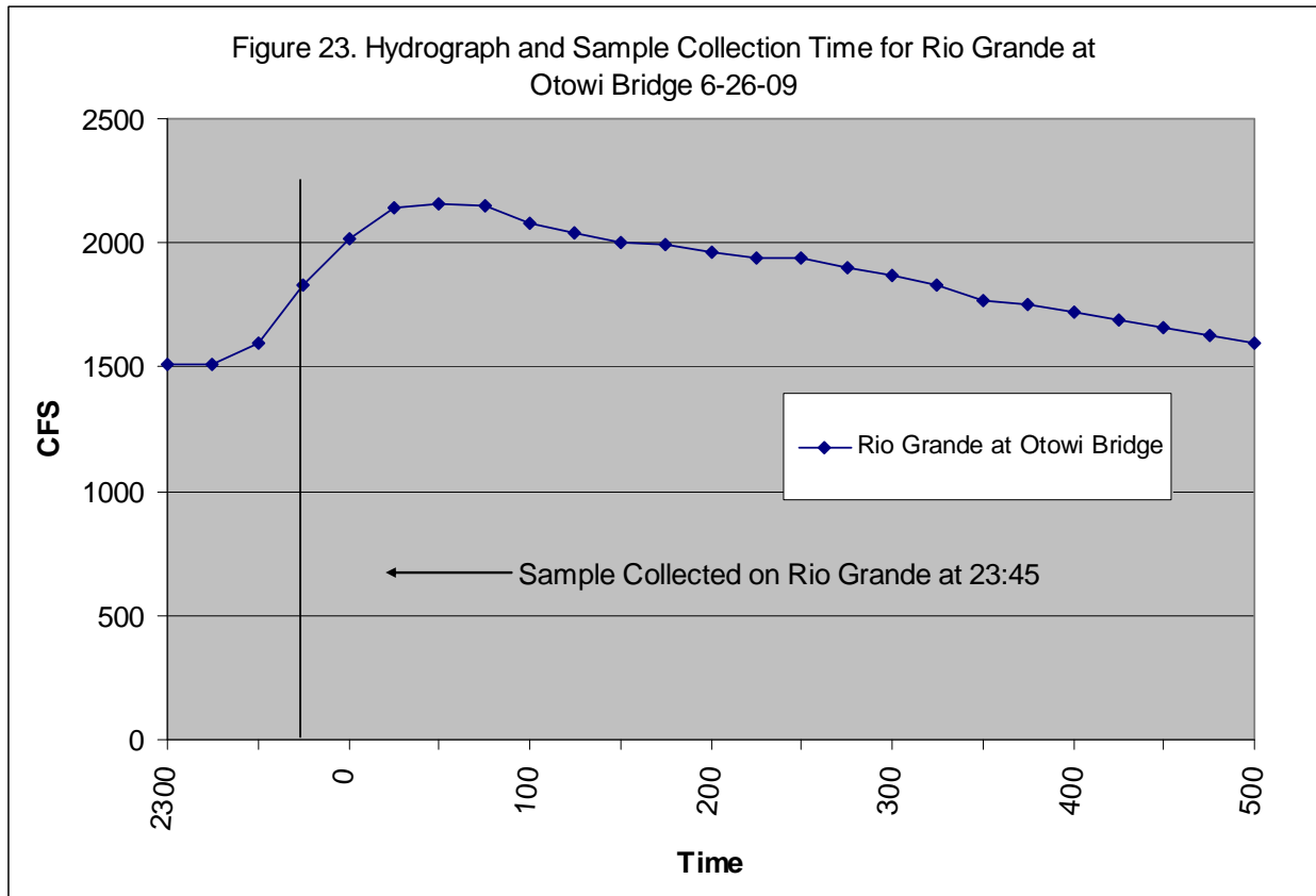
Figure 23 demonstrates flows in the Rio Grande at Otowi Bridge on 6-26-09. Flow at Otowi Bridge peaked at 00:30 and the sample was collected 45 minutes earlier on the rising leg of the hydrograph.
