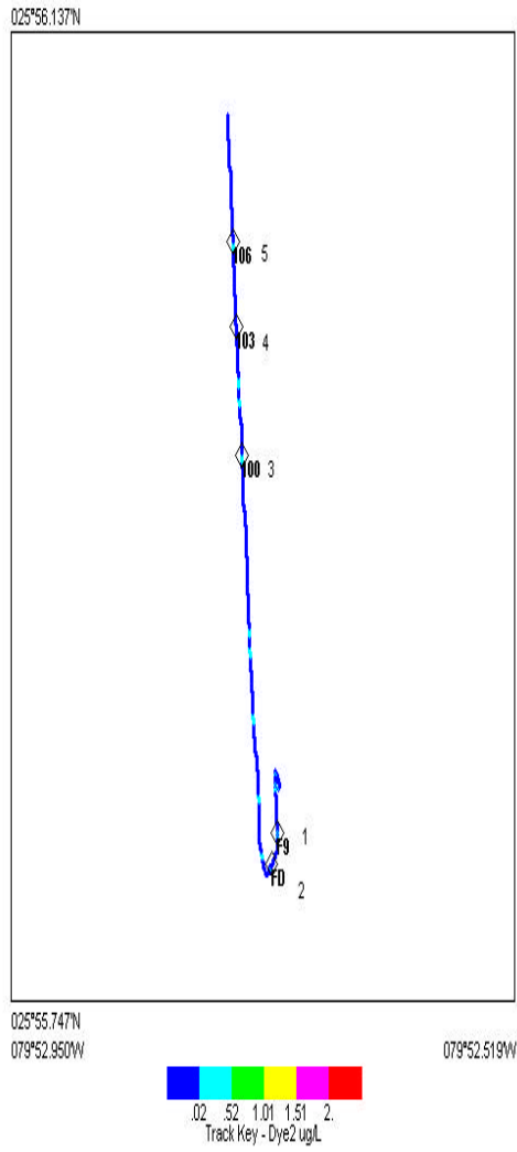
Background Transect
