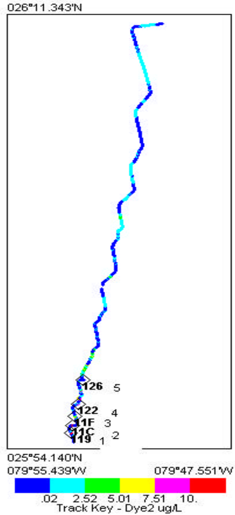
In-plume Transects
