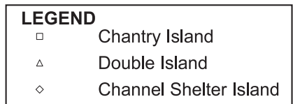
f) 2,3,7,8-tetrachlorodibenzo-p-dioxin
