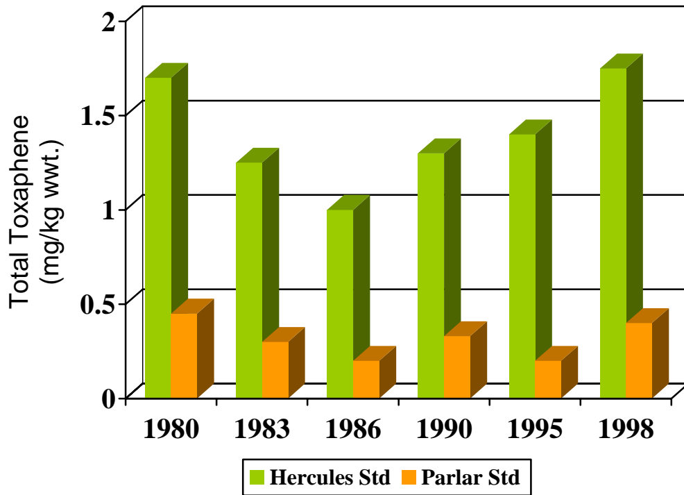
Figure 4-5. Total Toxaphene Concentrations in Whole Lake Superior Lake Trout Over Time Quantified Using Two Different Toxaphene Standards.
