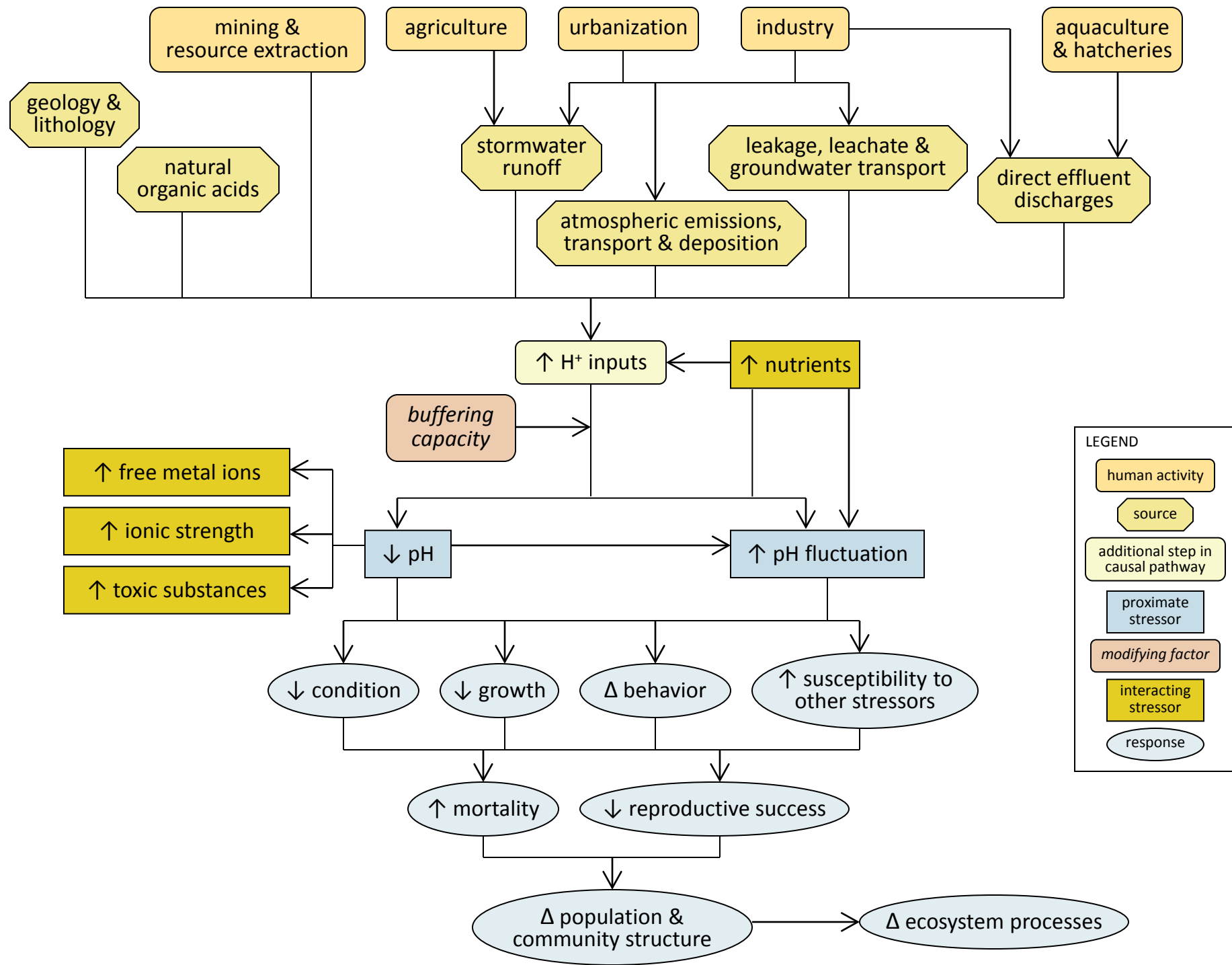
Simple conceptual model diagram for LOW pH
