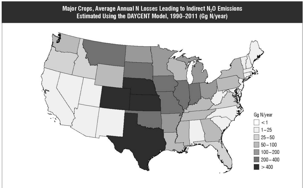
Figure 6-5: Major Crops, Average Annual N Losses Leading to Indirect N 2 O Emissions Estimated Using the DAYCENT Model, 1990-2011 (Gg N/year)
