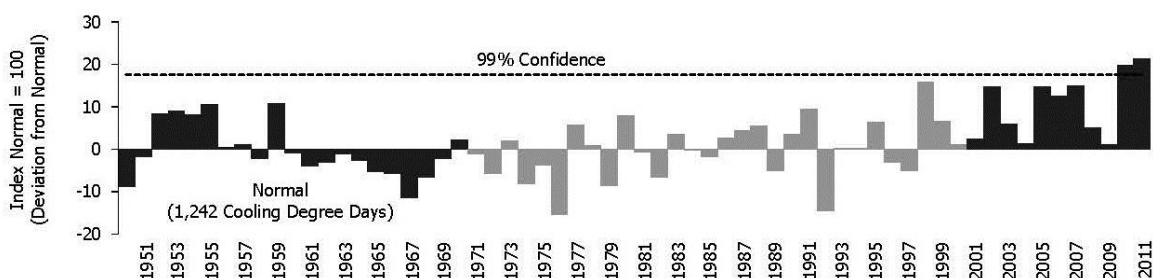
Figure 3-7: Annual Deviations from Normal Cooling Degree Days for the United States (1950–2011)
