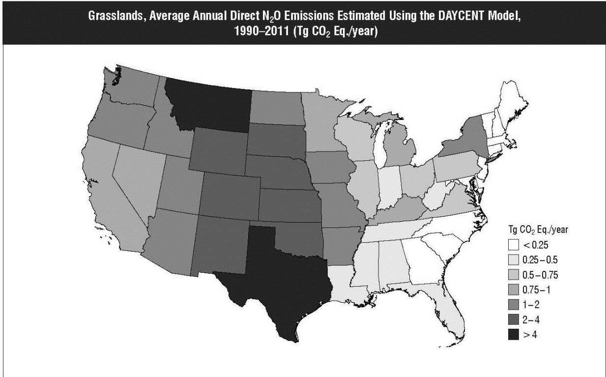
Figure 6-4: Grasslands, Annual Direct N 2 O Emissions Estimated Using the DAYCENT Model, 1990-2011 (Tg CO 2 Eq./year)
