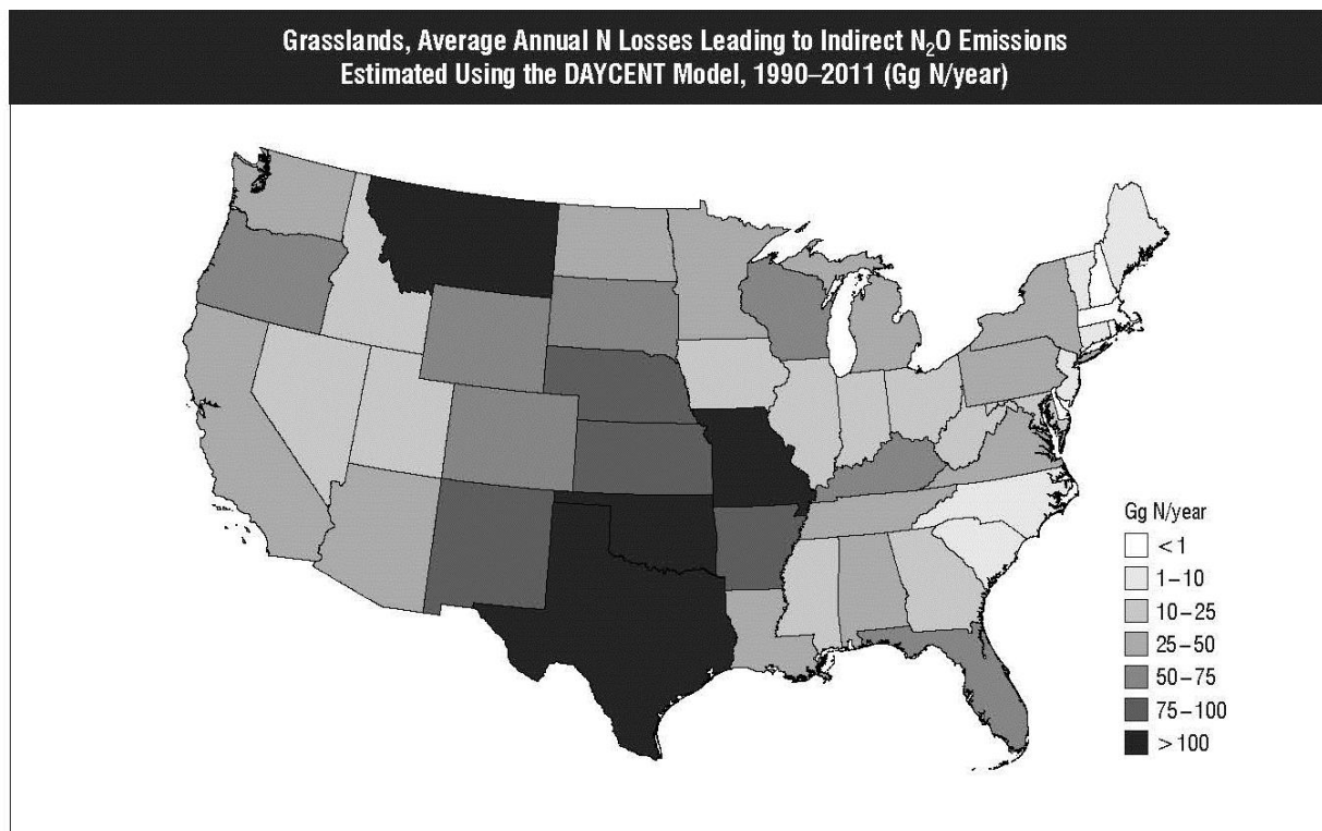
Figure 6-6: Grasslands, Average Annual N Losses Leading to Indirect N 2 O Emissions Estimated Using the DAYCENT Model, 1990-2011 (Gg N/year)
