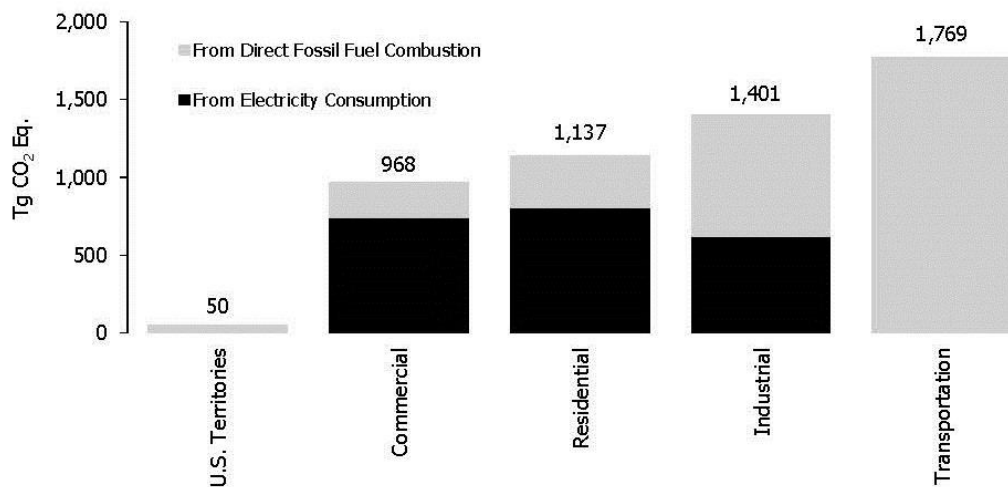
Figure 2-8: 2011 End-Use Sector Emissions from Fossil Fuel Combustion
