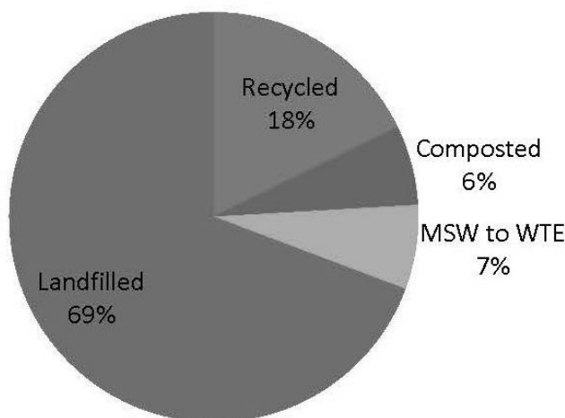
Management of MSW in the United States (BioCycle 2010)
