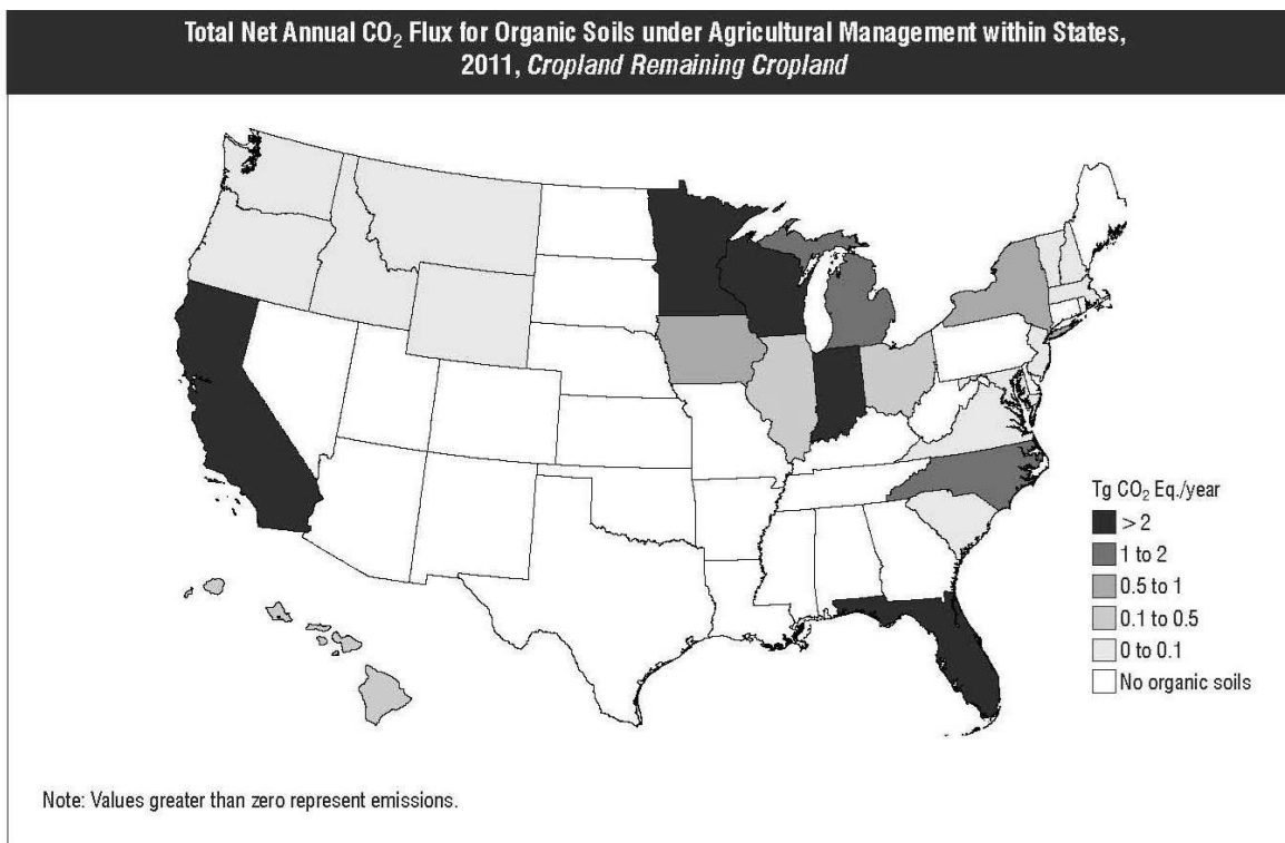
Figure 7-6: Total Net Annual CO 2 Flux for Organic Soils under Agricultural Management within States, 2011, Cropland Remaining Cropland
