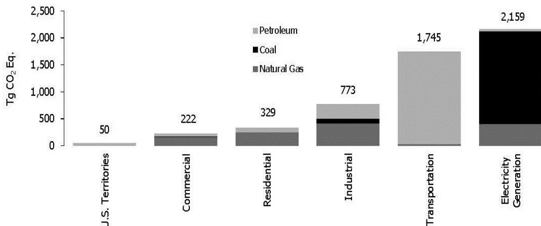
Figure 3-5: 2011 CO 2 Emissions from Fossil Fuel Combustion by Sector and Fuel Type
