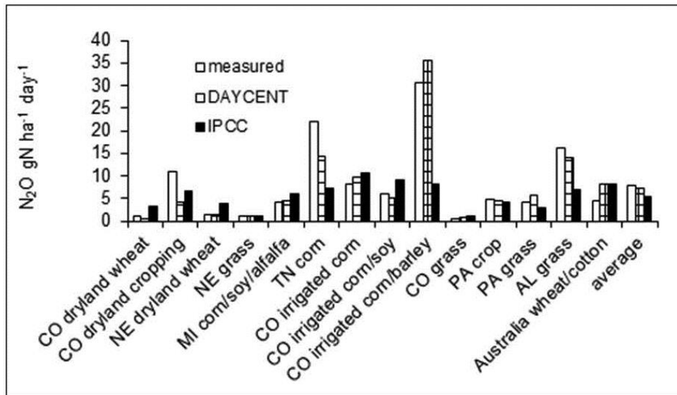
Figure 6-7: Comparison of Measured Emissions at Field Sites and Modeled Emissions Using the DAYCENT Simulation Model and IPCC Tier 1 Approach.
