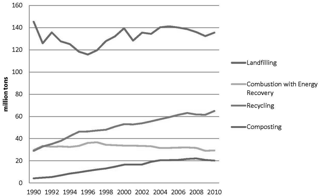
Figure 8-3: MSW Management Trends from 1990 to 2010 (EPA 2011)
