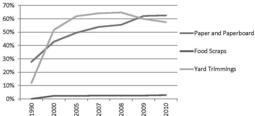
Figure 8-4: Percent of Recovered Degradable Materials from 1990 to 2010, percent (EPA 2011)
