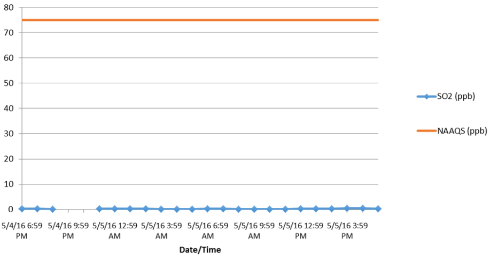
Hourly Averages SO2 (ppb)
