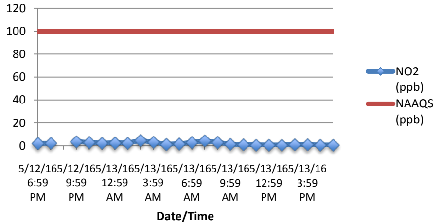
Hourly Averages NO2 (ppb)
