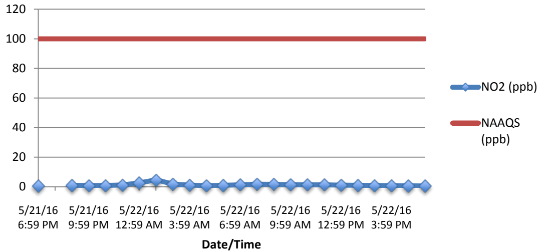
Hourly Averages NO2 (ppb)
