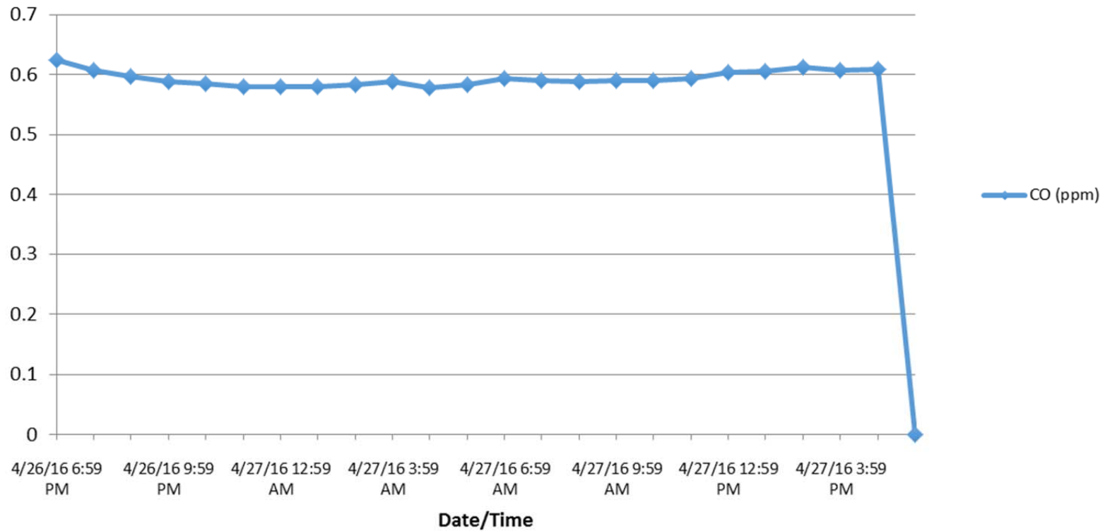
Hourly Averages CO (ppm) NAAQS 35 ppm
