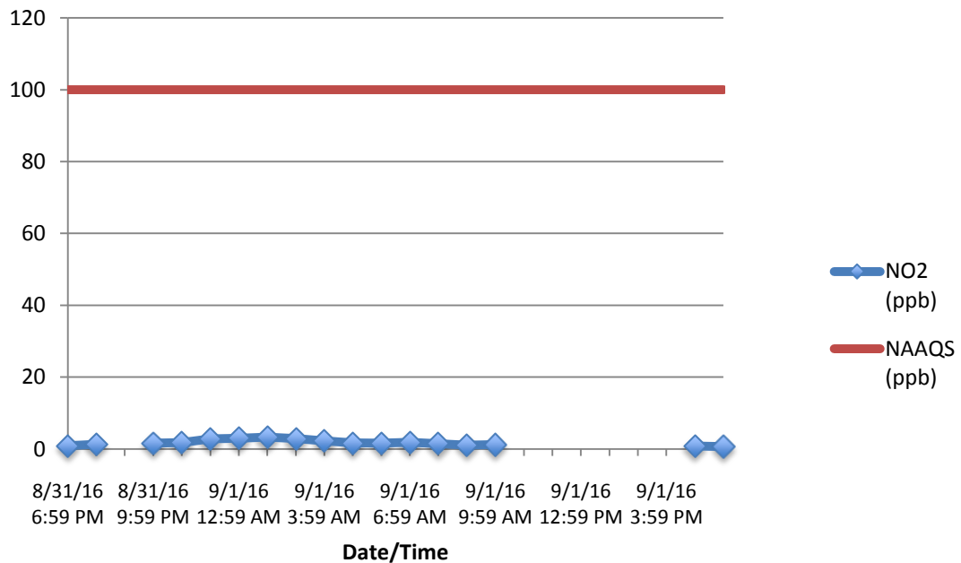
Hourly Averages NO2 (ppb)
