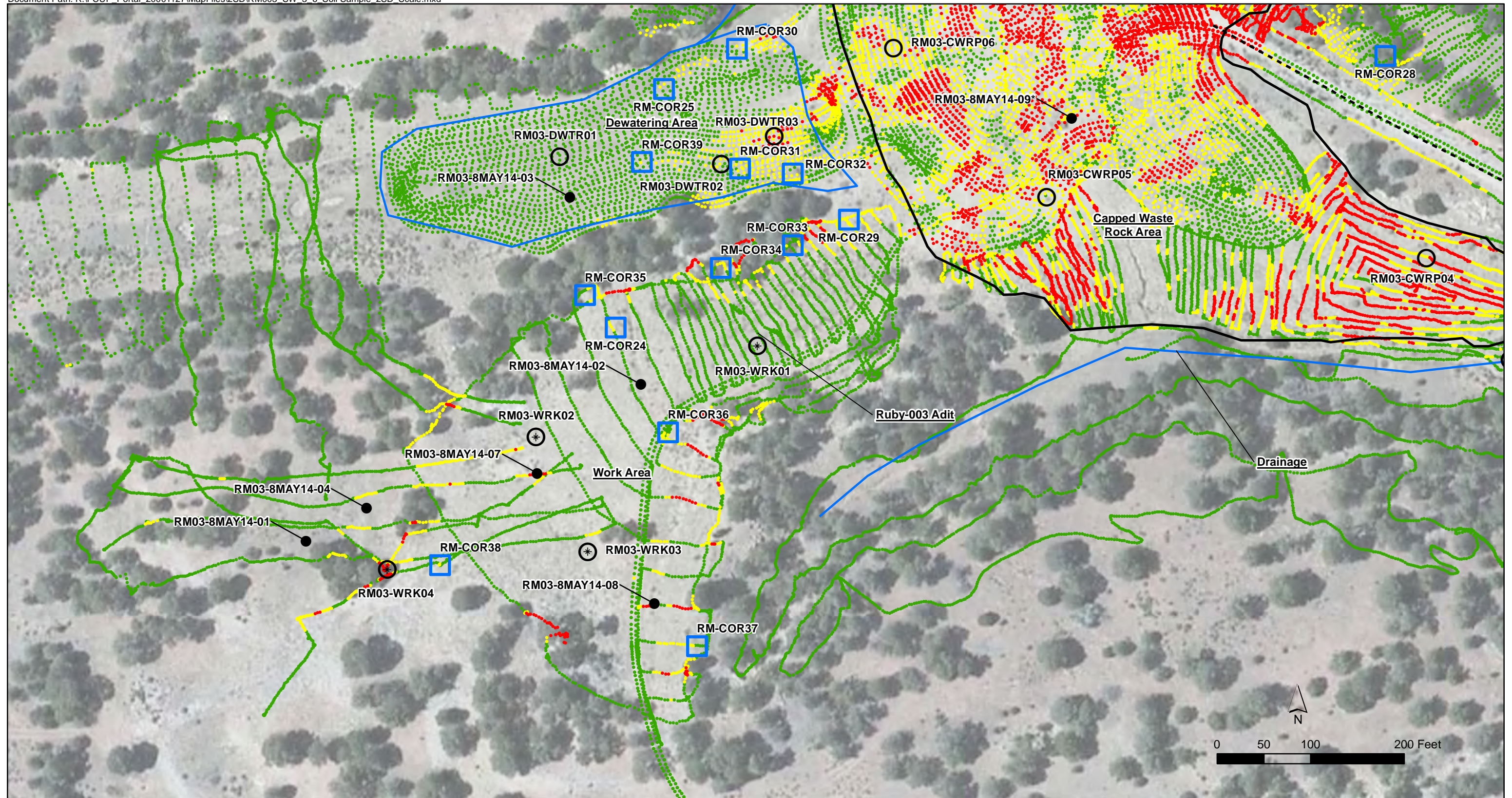
Figure 3-6 Ruby Mine No. 3 Dewatering and Work Area Soil Sample Locations Ruby Mines Phase 3 Removal Site Evaluation Work Plan
