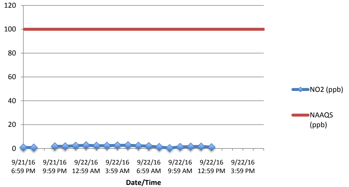
Hourly Averages NO2 (ppb)
