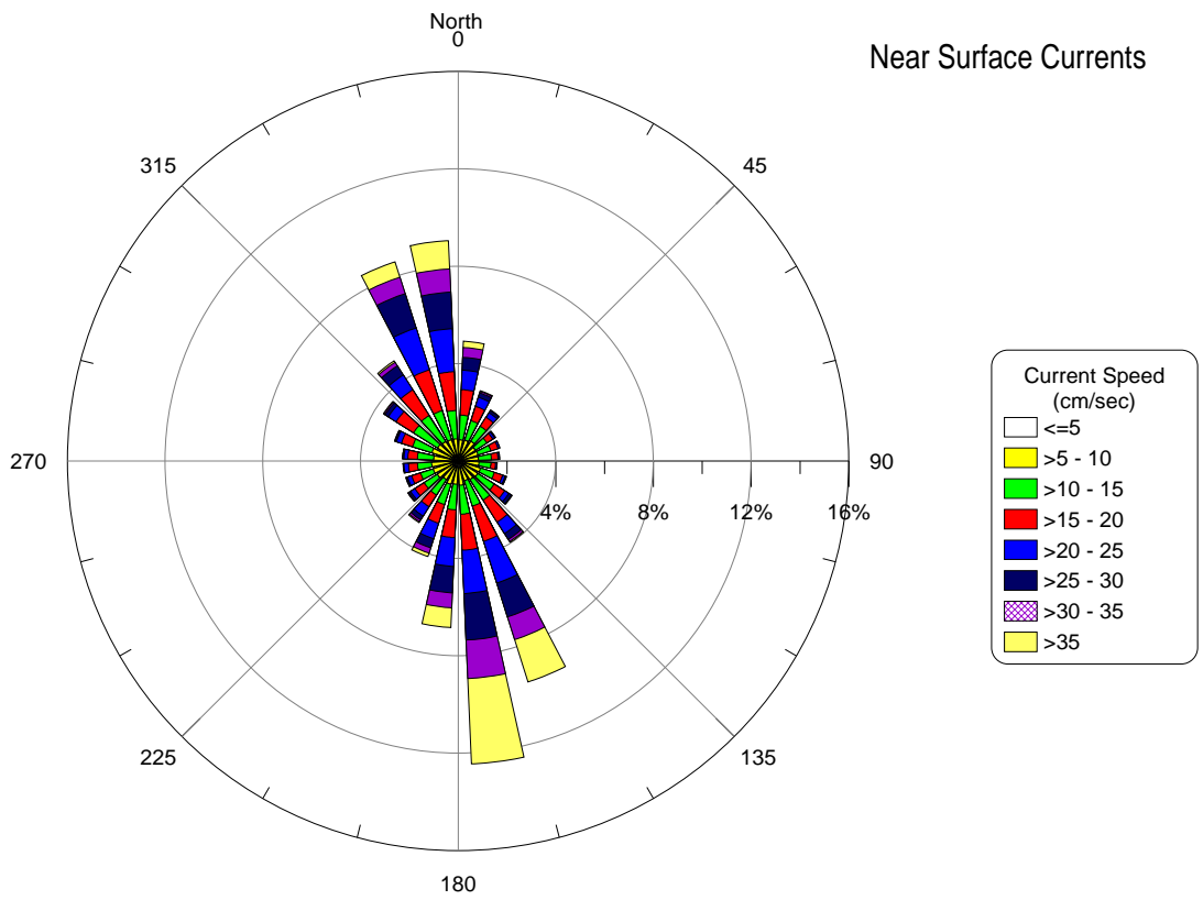
Figure 20: Jacksonville ODMDS Current Rose for Near Surface Currents
