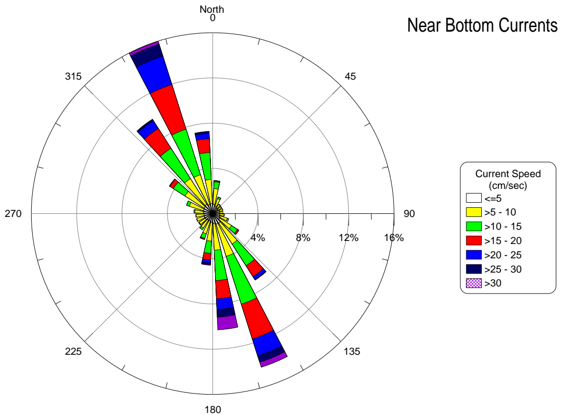
Figure 21: Jacksonville ODMDS Current Rose for Near Bottom Currents
