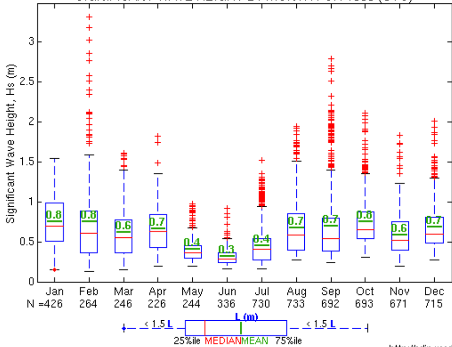
083 KINGS BAY, GA SIGNIFICANT WAVE HEIGHT BY MONTH FOR 1998 (UTC)
