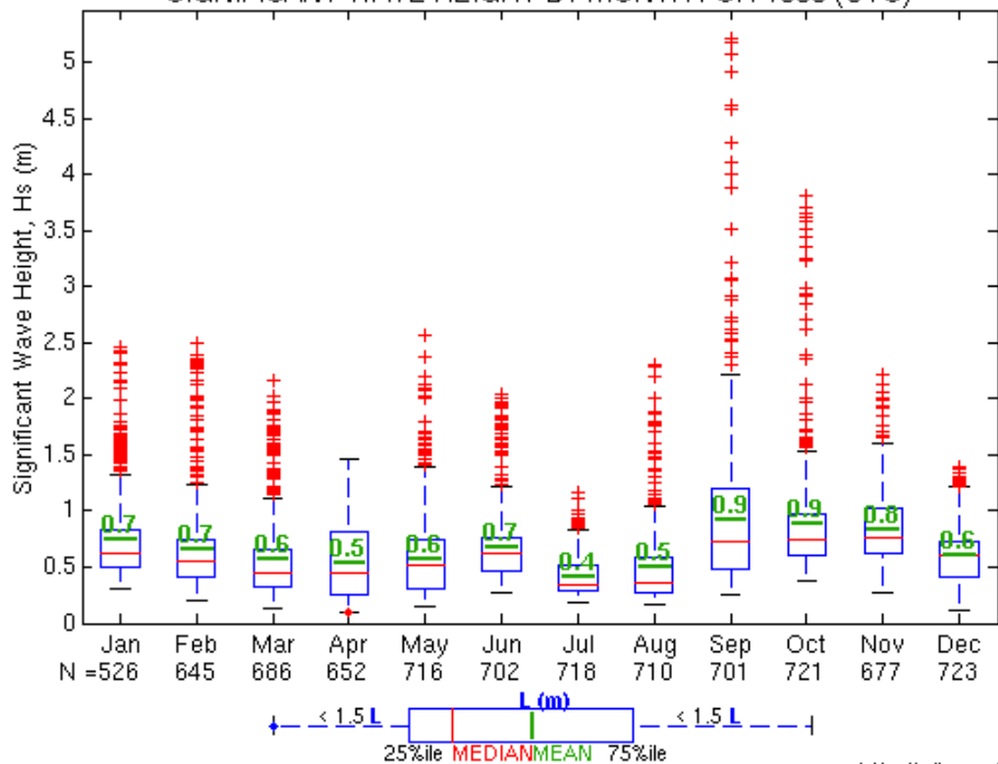
083 KINGS BAY, GA SIGNIFICANT WAVE HEIGHT BY MONTH FOR 1999 (UTC)
