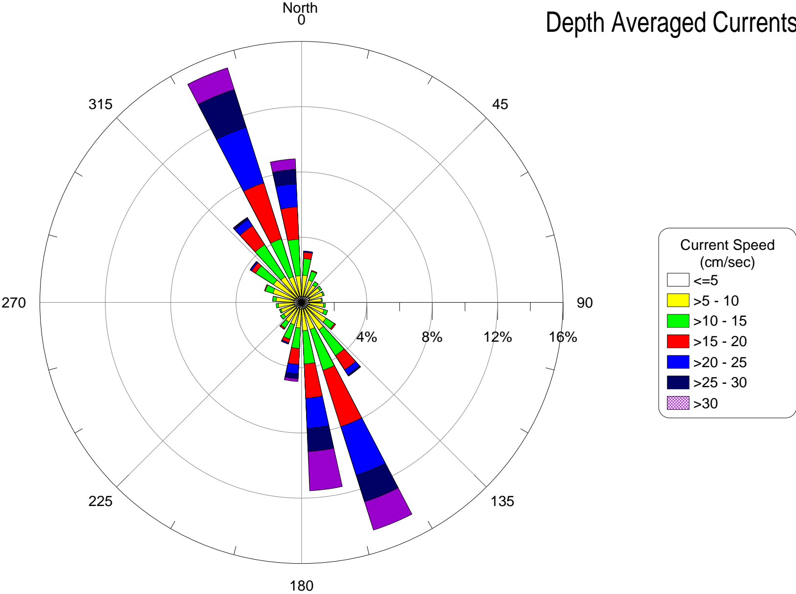
Figure 18: Jacksonville ODMS Depth Averaged Current Rose Diagram
